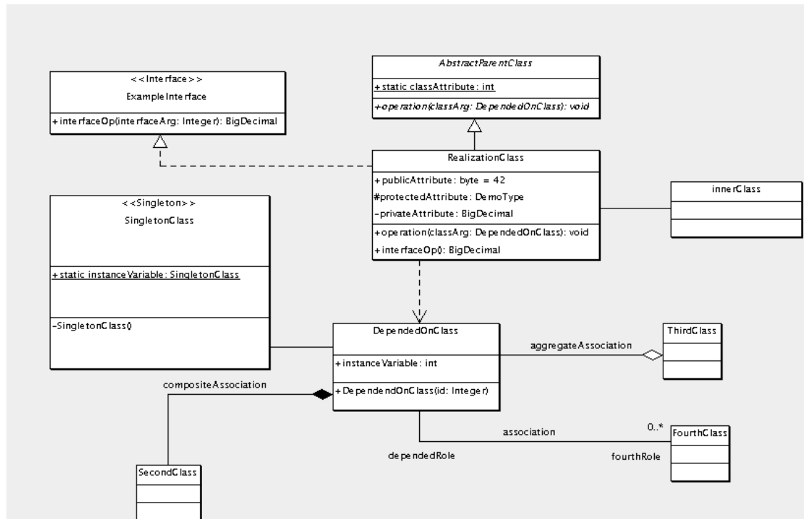
Figure 18.1. Possible artifacts on a class diagram.
