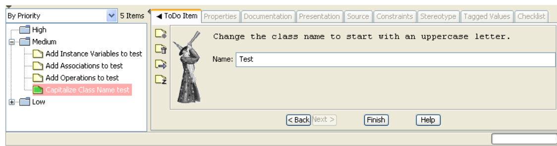
Figure 13.5. Example of a Wizard
