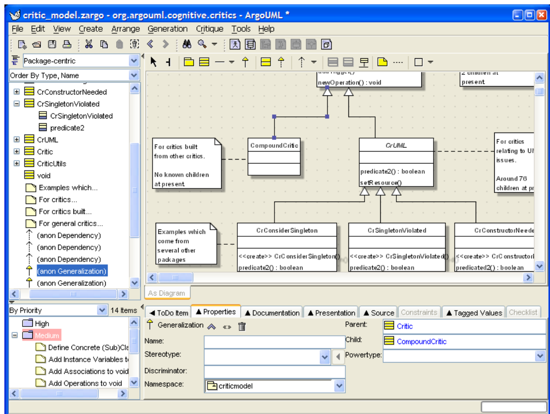
Figure 8.1. Overview of the ArgoUML window
