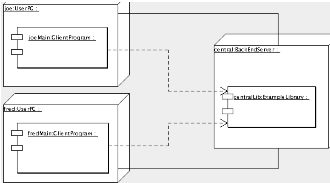
Figure 23.2. Possible artifacts on a deployment diagram.
