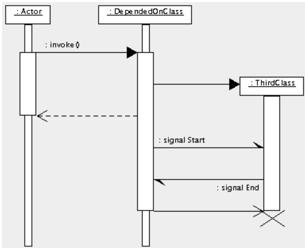
Figure 19.1. Possible artifacts on a sequence diagram.
