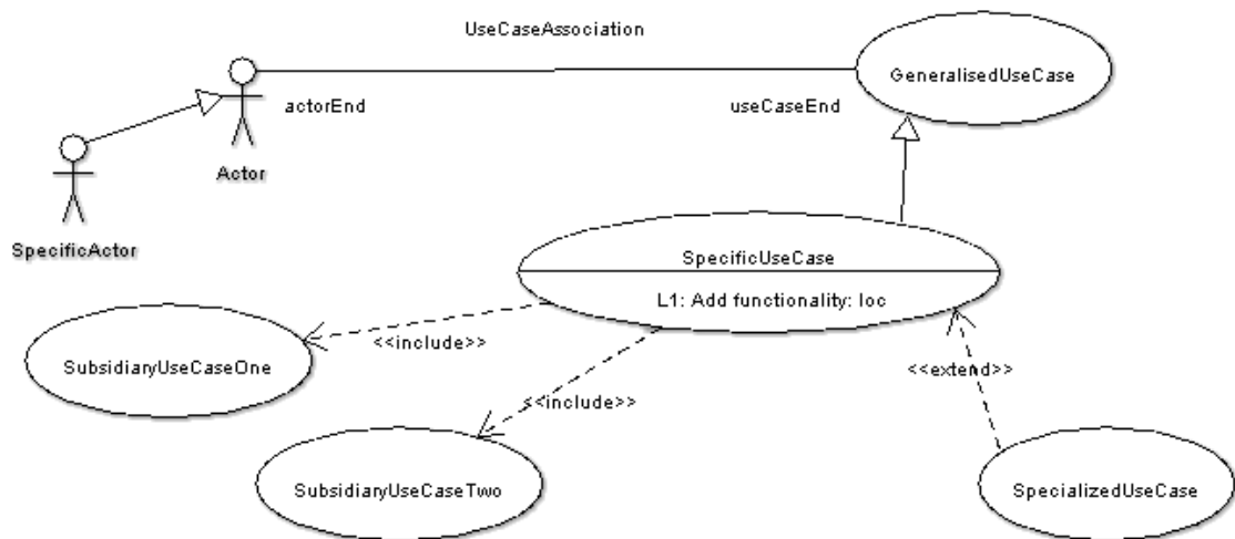
Figure 17.1. Possible artifacts on a use case diagram.
