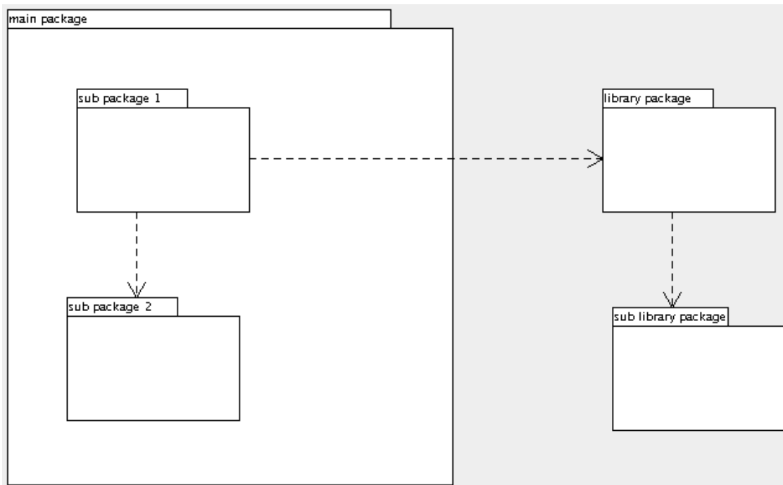
Figure 18.2. Possible artifacts on a package diagram.
