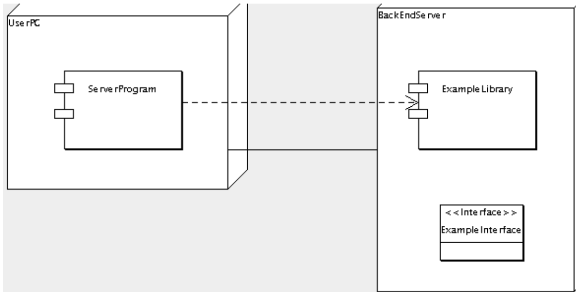
Figure 23.1. Possible artifacts on a component diagram.
