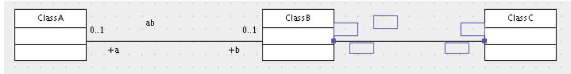
Figure 12.9. A couple of associations with adornments
