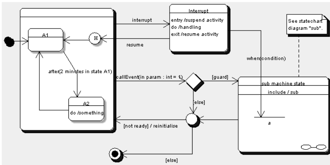
Figure 20.1. Statechart diagram artifacts 1.
