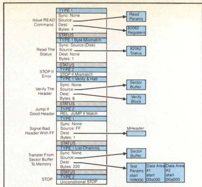
Figure 7: A command block that performs a read from the Winchester disk is easy to construct. The read command and its parameters are sent to the 82062 controller. The CPU can examine the command pointer to determine how the command block terminated. The variable MHeader indicates a mismatch of the header.
