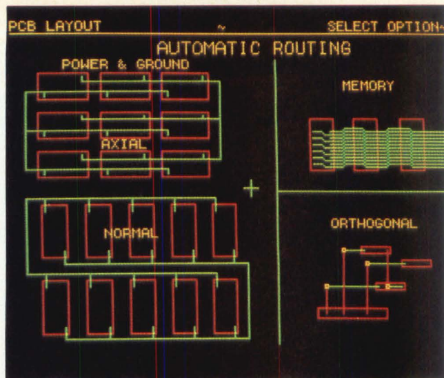
Figure 3: The Redboard system from Racal-Redac runs on an IBM PC or XT and has separate routers for power and ground, memory and orthogonal traces. By choosing components to be routed by each of these programs, optimum trace layout is possible with nested 45° angles on memory traces.
