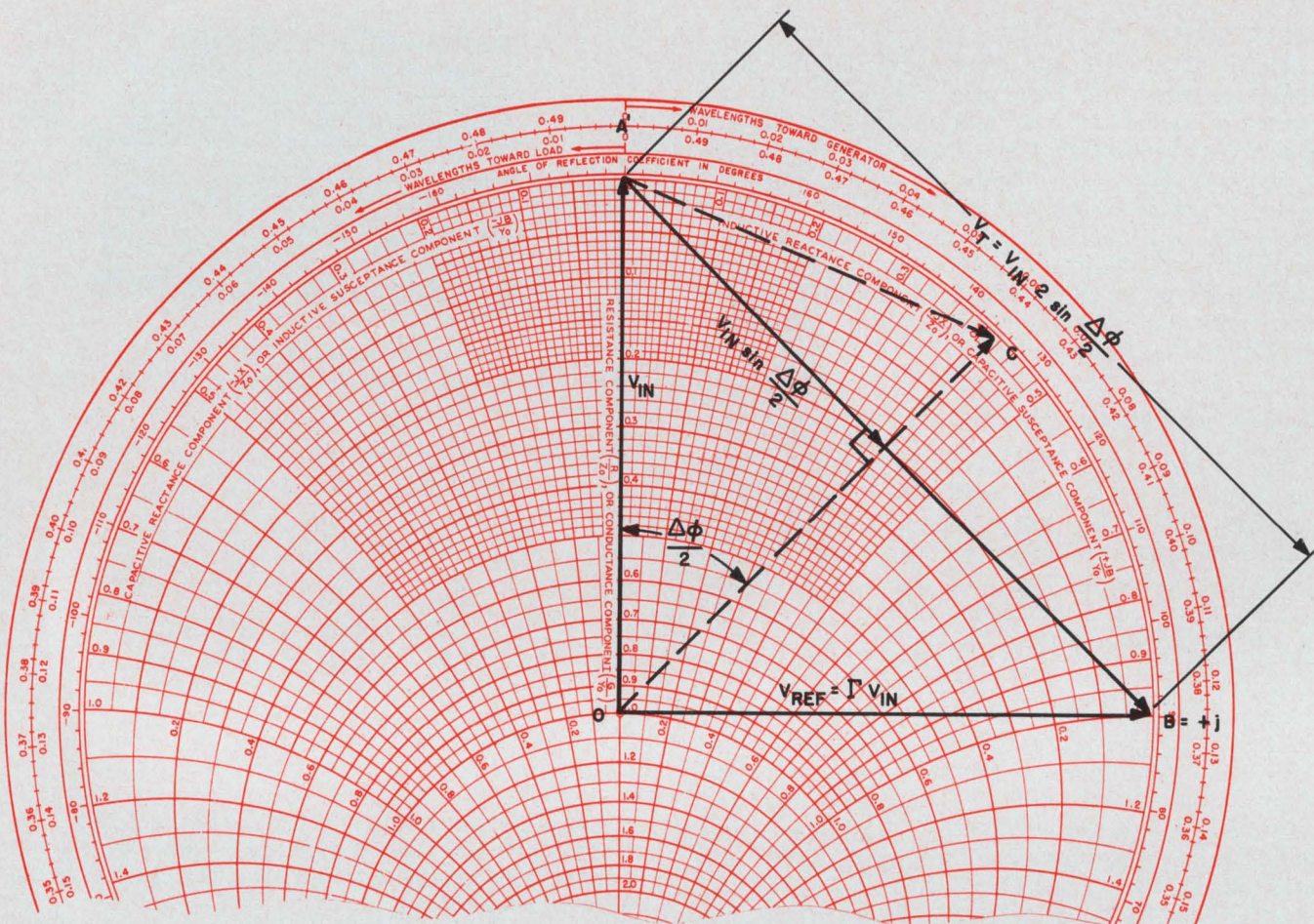
6. Impedance plot of an ideal diode and its inductive matching network shows 90^\circ (points A'B) and 45^\circ (points A'C) phase shifts. Points AA' represent the com-
