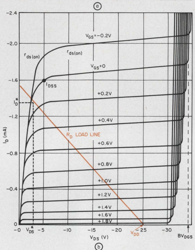
8. With two power supplies (a), the difference between I_{D(MIN)} and I_{D(MAX)} is lessened. When the FET output characteristic (b) is available, the value of R_D is quickly and easily determined. Note that in the absence of this plot, Fig. 7b may be used for constructing a value of R_D .
