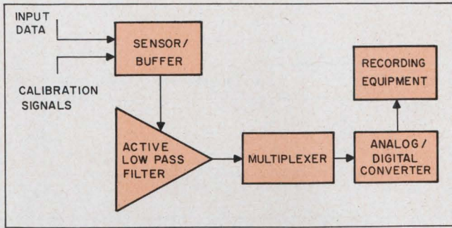
1. Typical analog processing system consists of sensing and buffering, low-pass filtering, multiplexing, A/D conversion and recording.
