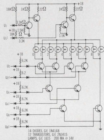
Fig. 2. Binary-to-decimal decoder drivers
