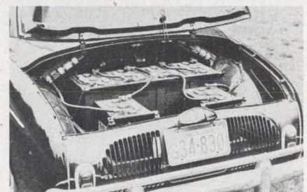
A Kilowatt's hood (above) and trunk (below) are filled with 900 pounds of lead-acid batteries. The car's range is only 35 miles.
