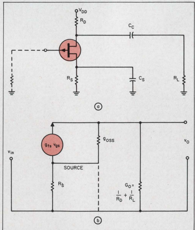
5. A FET RC-coupled amplifier (a) may be considered as a general purpose ( f < 1 MHz) type. The equivalent circuit appears in (b). FETs are superior to bipolars here because of their lower intermodulation distortion products.
