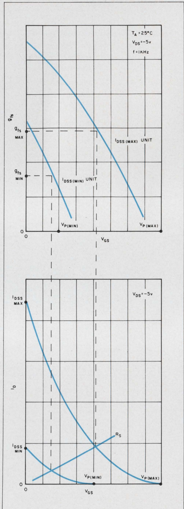
9. The relationship between I_D and g_{fs} as functions of V_{GS} are used in calculations of gain in FET amplifiers. Minimum and maximum values of g_{fs} are established by a construction procedure based on R_s intercepts.
