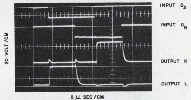
3. Input and output waveforms of the comparator, built with discrete components, show the relationship of outputs, K and L, to inputs, G_A and G_B .
