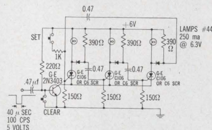
Fig. 3. High current ring counter
