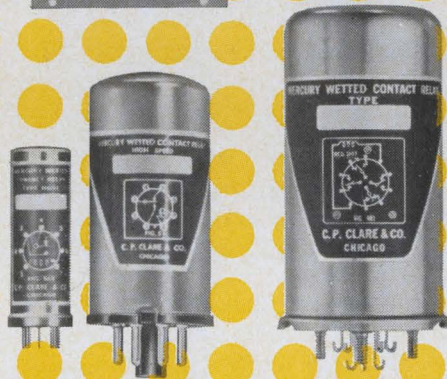
Single pole relays Seven-pin miniature (HGSL) (left). Octal plug (HGS) (right)
