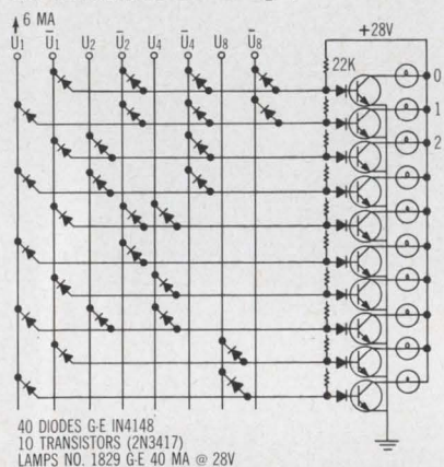
Fig. 1. Binary-to-decimal converter with drivers
