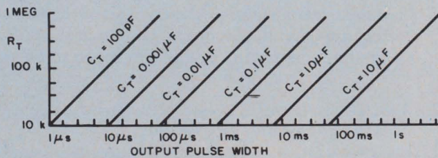
7. Wide range single-shot output pulse width can be adjusted by selecting C_T and R_T , as shown in the ac-
