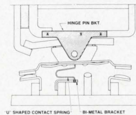
U SHAPED CONTACT SPRING BI-METAL BRACKET
