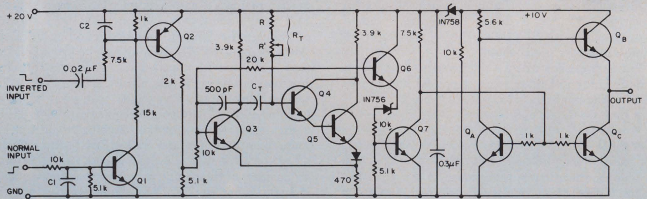
WIDTH OF OUTPUT PULSE IS DETERMINED BY C_T AND R_T WHERE R_T = R + R'/2
