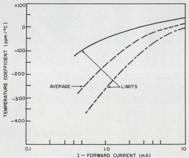
Temperature-stable 6-volt reference (a) uses a single transistor having characteristics shown in (b) and (c) and a J-FET to supply the steady current.
