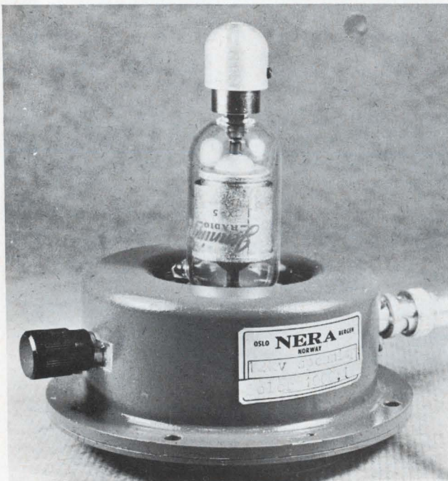
5. An accuracy of +2% is achieved with this capacitive divider by using a vacuum capacitor and a ceramic-trimmed precision mica.
