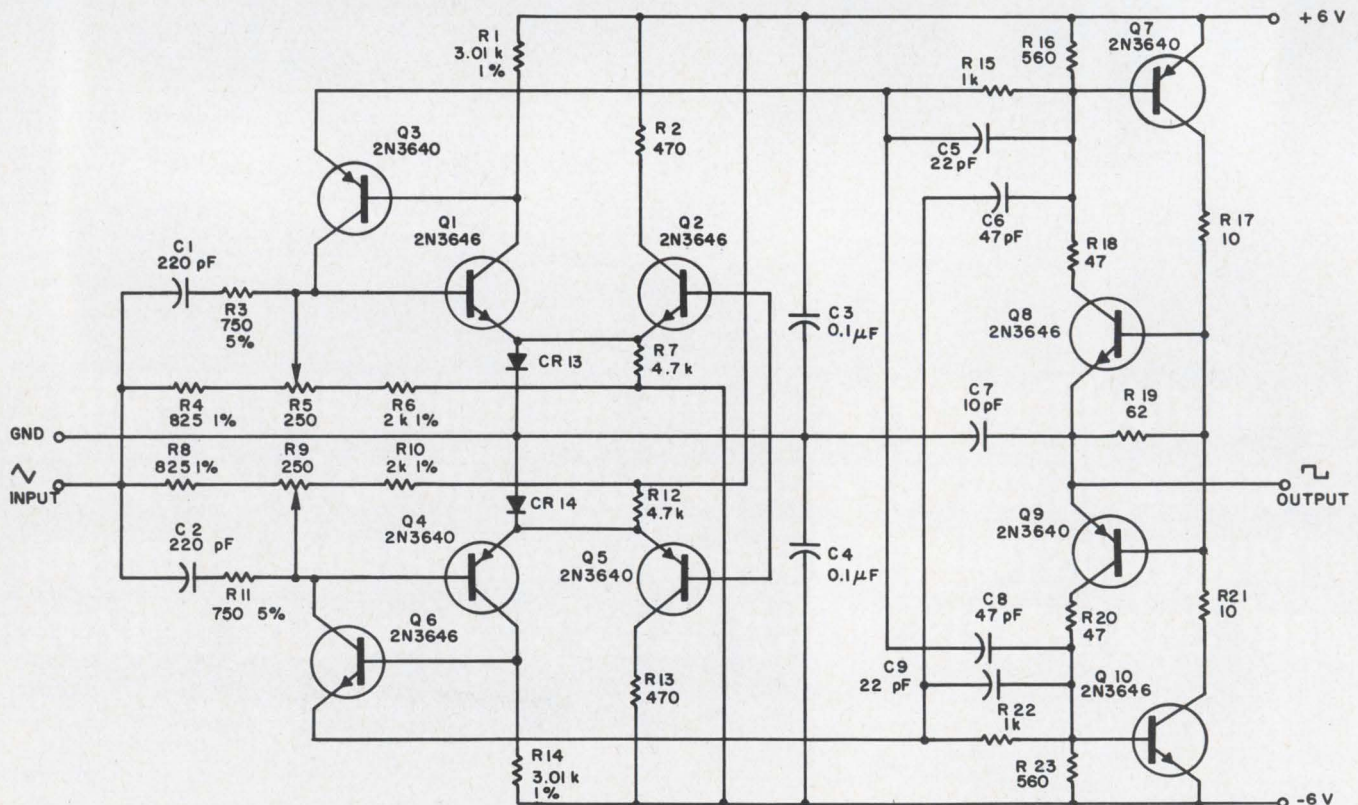
Ten-volt peak-to-peak square wave appears at the output in response to \pm 2.5 V applied to the input. The rise time
