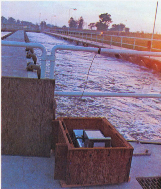
Brady brought his Beckman dissolved-oxygen meter right to his aeration tank, dropped its sensor into the effluent, and plugged it in. The instrument worked so well, it turned up a testing flaw: bacteria used the oxygen.
