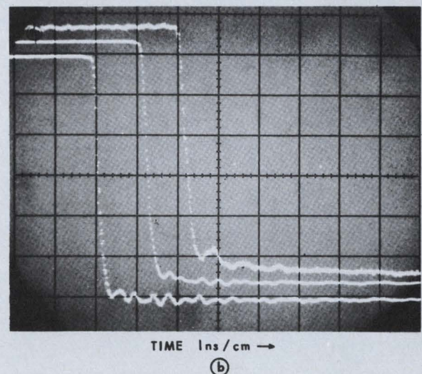
9. Add dc offset through one leg and 4:1 probe in the other (a). Photo (b) shows input, output, and tap-off.
