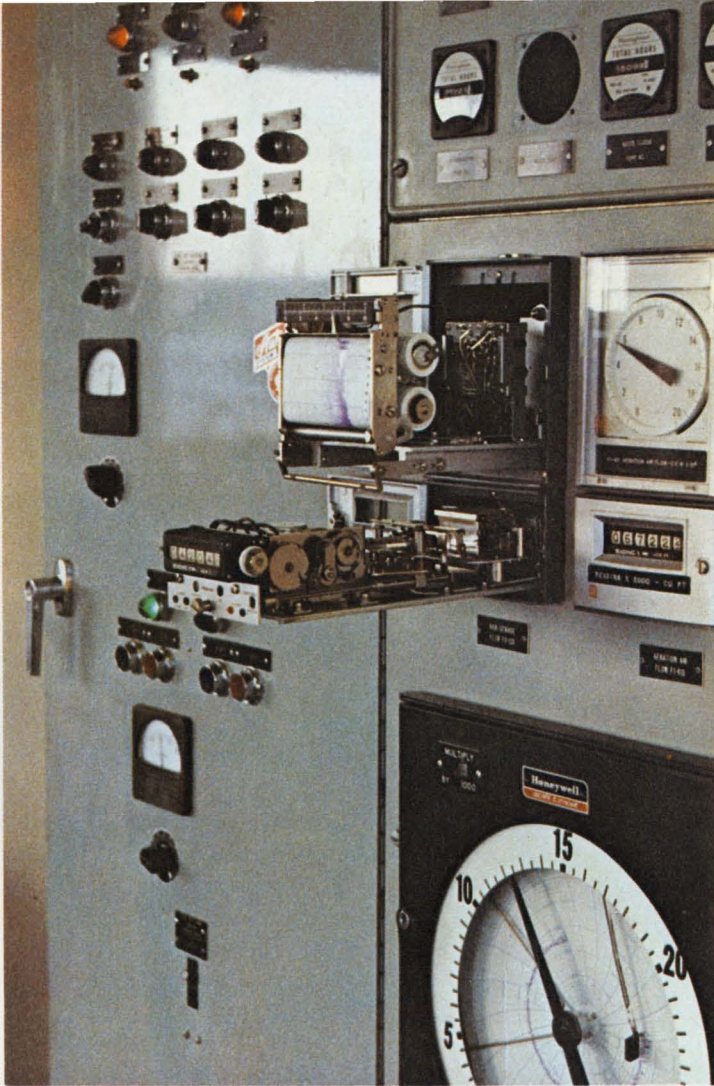
This strip-chart recorder is supposed to measure sewage flow. Its rollers, however, fail to pull paper past the pen. Below it, an electronic integrator records total sewage. Unfortunately, it loses about a million gallons a day out of about six million that the plant processes.
