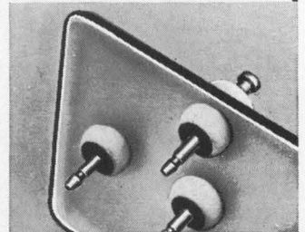
Spring push-nut locks it in position on panel — providing an hermetic seal
