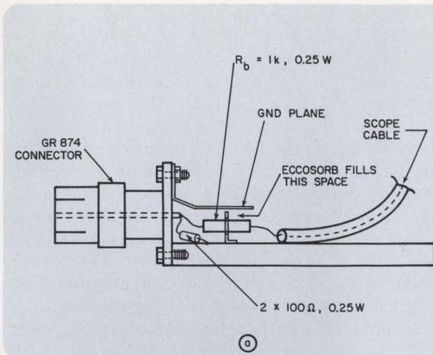
8. Mock-up for base drive circuitry (a). Top trace (b) shows a 200-ps step going directly into the scope; bot-
