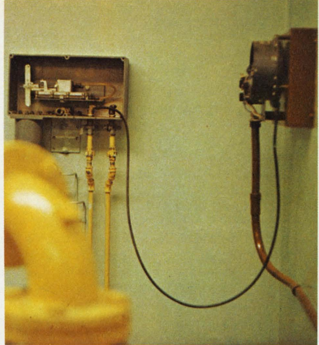
This differential-pressure sensor blew its diaphragm. A Honeywell representative was said to have ordered three replacements but when they arrived with a bill for $375, he returned them to their manufacturer.
