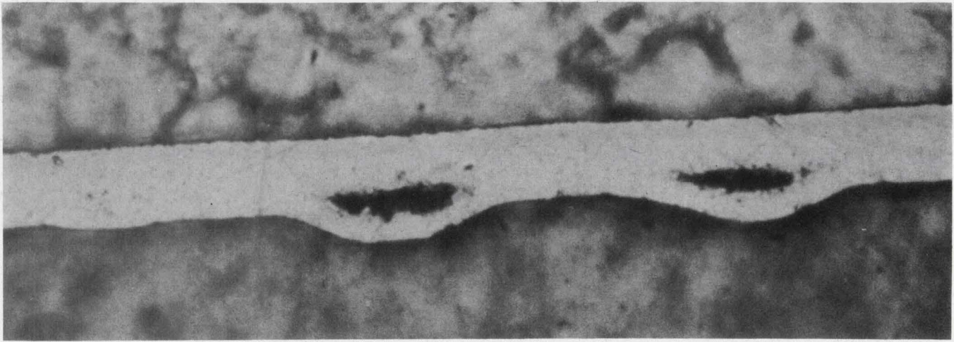
Occlusions in a gold deposit result when some electrolyte is trapped or embedded in the plate as shown in this cross-
