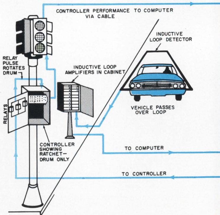
When a car passes over a buried loop detector, its metal increases the loop's inductance much like the insertion
