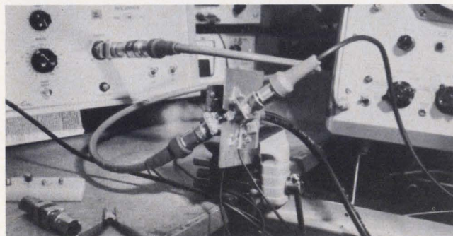
12. The finished jig. Input and output circuitry are mounted on opposite sides of a 2-sided PC board.
