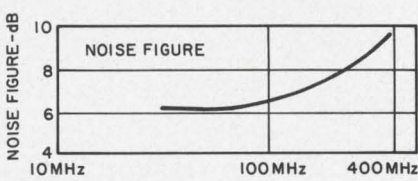
Noise vs frequency curve covers amplifier in 10-to-400-MHz range.
