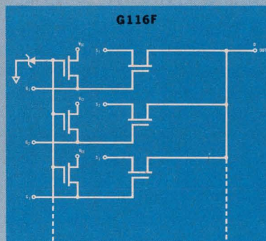
"G" Series MOS Switches
