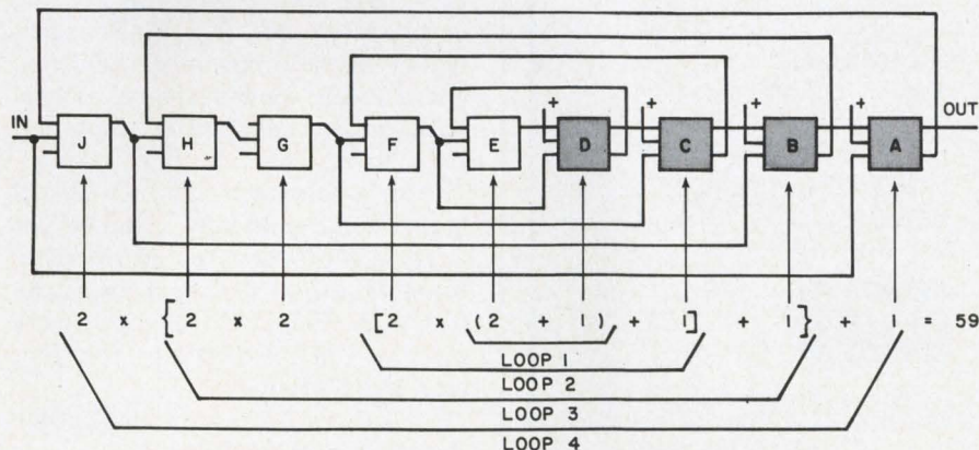
A 59s counter is built entirely with flip-flops. The ADD-ONE flip-flops (shaded) must have C and K inputs interchanged, as shown, for the counter to work.
