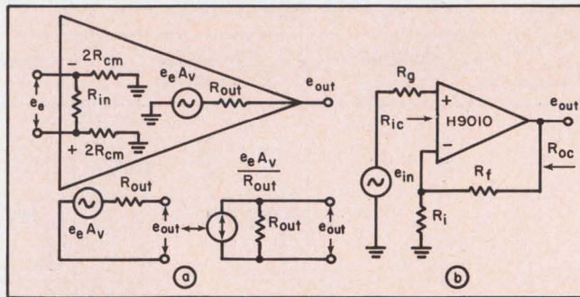
1. Voltage amplifier results when an operational amplifier is connected as shown in (b). The op-amp equivalent circuit is in (a).
