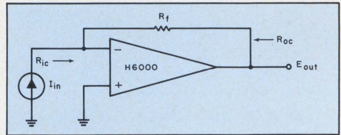
3. Transresistance amplifier connection results in low closed-loop input and output resistances.
