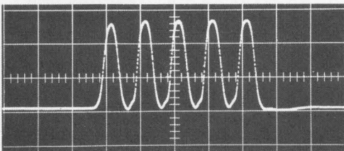
200 MHz Pulse Burst. 5 ns/cm, 0.5 V/cm
