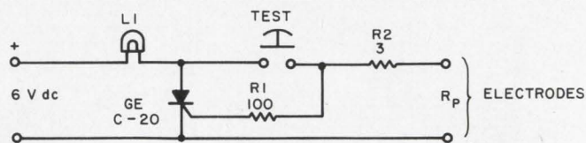
Change of 0.1 ohm is sensed with a simple single-SCR circuit. It is used to detect shorts in electrodes immersed in 0.1-ohm electrolyte.
