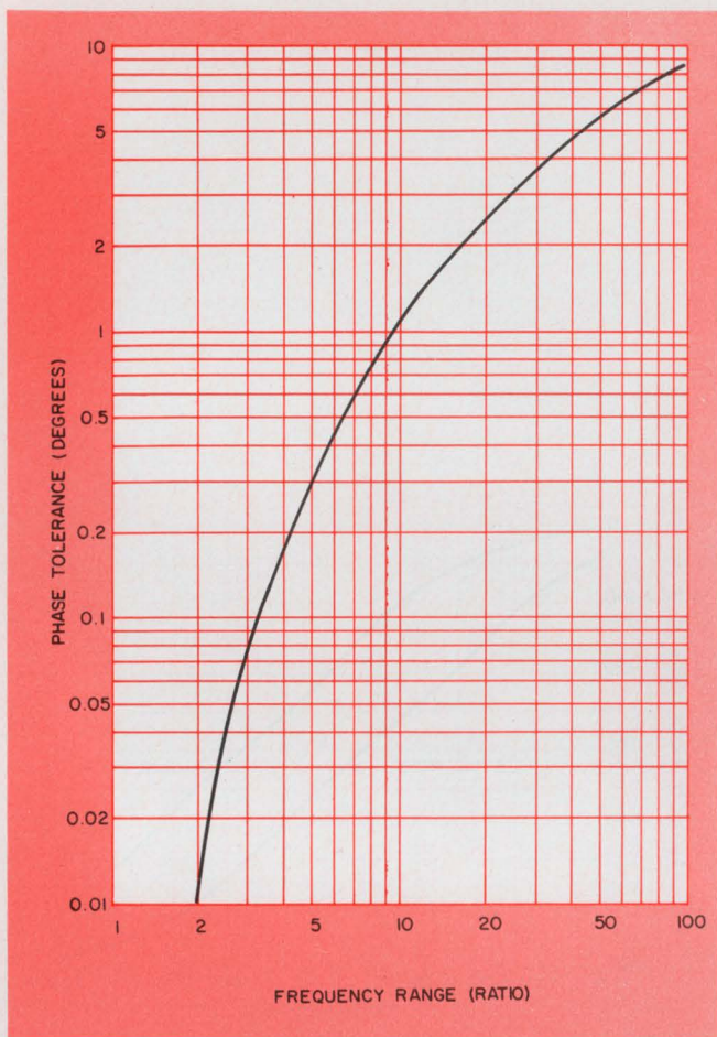
4. A four-pole phase shifter exhibits this theoretical relationship between frequency range and phase tolerance. If a tighter tolerance is required, more poles must be incorporated into the circuit.
