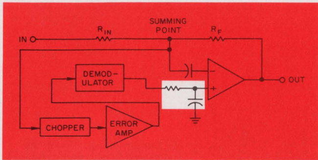
2. Chopper stabilization uses a feedback loop to keep the summing-point voltage near zero. The RC network between the demodulator and the noninverting input is a low-pass filter. A potential problem is chopper noise.
