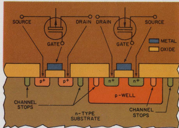
A p-channel device (left) and an n-channel (right) together form the basic element in complementary MOS. The fabrication process shown is metal-gate, which normally requires channel stops to limit inversion effects.
