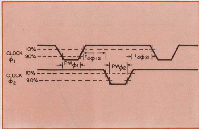
4. Minimum clock pulse widths, PW_{\phi_1} and PW_{\phi_2} , must be sufficient to permit charging and discharging of internal gate capacitors. Clock-pulse spacings, t_{d\phi_{12}} and t_{d\phi_{21}} , must always be larger than, or equal to, zero. This prevents the occurrence of two clock pulses at the same time.
