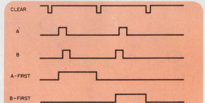
2. Input and output waveforms illustrate detection of the leading edge of whichever pulse occurs first.
