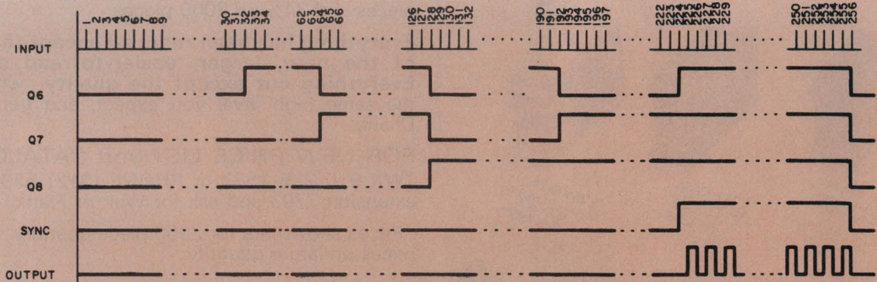
2. Timing diagram for 32-bit burst length and 12.5% duty cycle. The input signal can be any waveform.
