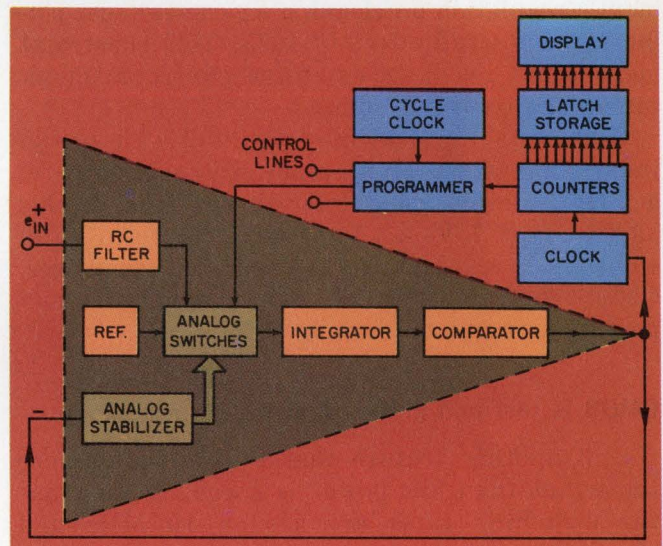
3. Analog Devices' DPM, the AD 2001, uses CMOS in its analog switch and stabilizer sections (green boxes) because of the low power requirements. A dual-slope converter, the AD 2001, features dc-error compensation through the use of the company's Analok circuit (high-lighted by the triangle).
