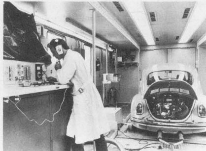
Technician in the trailer unit checks constant-volume-sampling instrument, which collects exhaust gases from the car undergoing test on the dynamometer.
