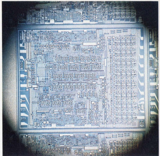
Ragen Semiconductor's touch-tone converter for telephone systems has 1150 transistors on a 169 × 137-mil chip. A custom circuit, the chip includes two oscillators, a 64-bit read/write memory and dial-interrupt conditioning circuitry.
