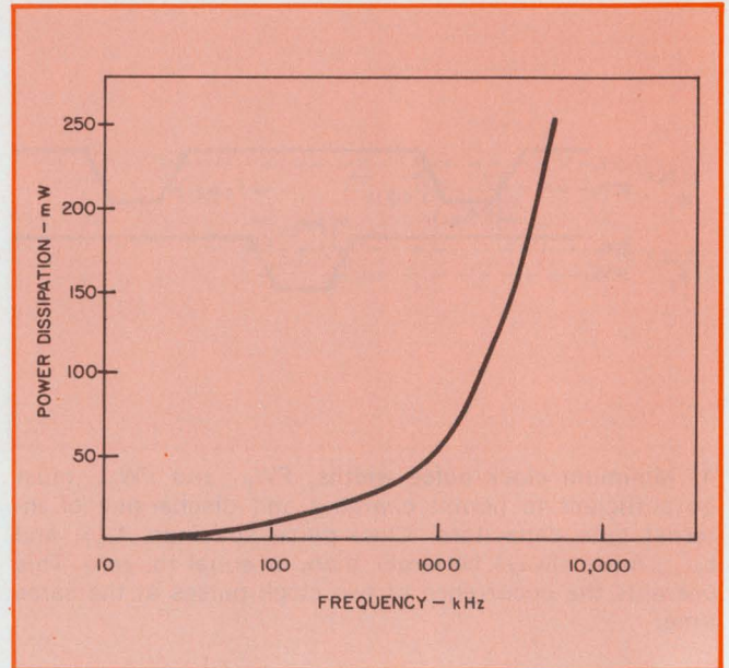
8. Operating frequency of a dynamic register sometimes is limited by the internal dissipation rather than by the internal propagation delays.
