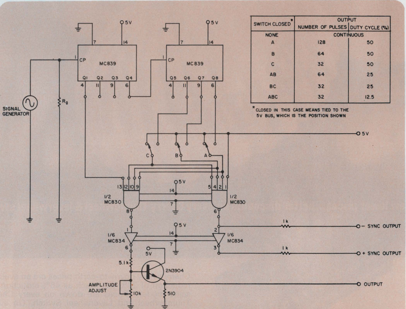
1. Tone-burst generator provides the burst lengths and duty cycles that are selected by switches A, B and C.
