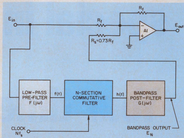
1. The notch filter reproduces the input except for sign inversion and the subtraction of a narrow notch of frequencies. The commutative bandpass section selects the narrow frequency notch and provides 180^\circ phase shift. The summation of the original signal and the bandpass signal by op amp A_1 produces the notch at f = f_s .
