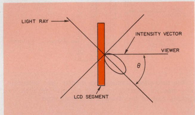
5. The illumination scheme suffers from a wide variation in light intensity with viewing angle.
