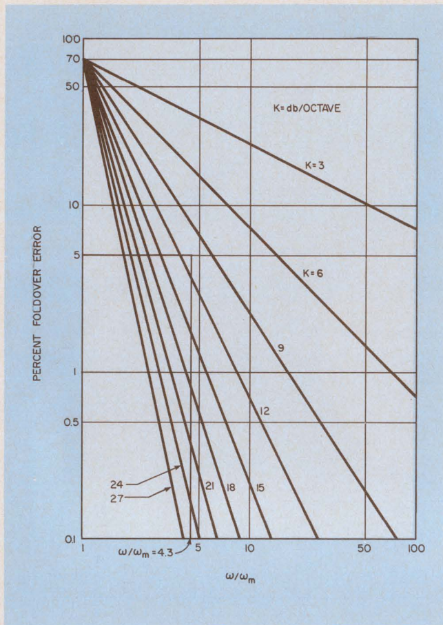
4. The required cutoff slope for the prefilter is chosen to meet the given foldover error specification of 5% with the help of this chart. The curves are normalized for a 3-dB response at \omega_m .
