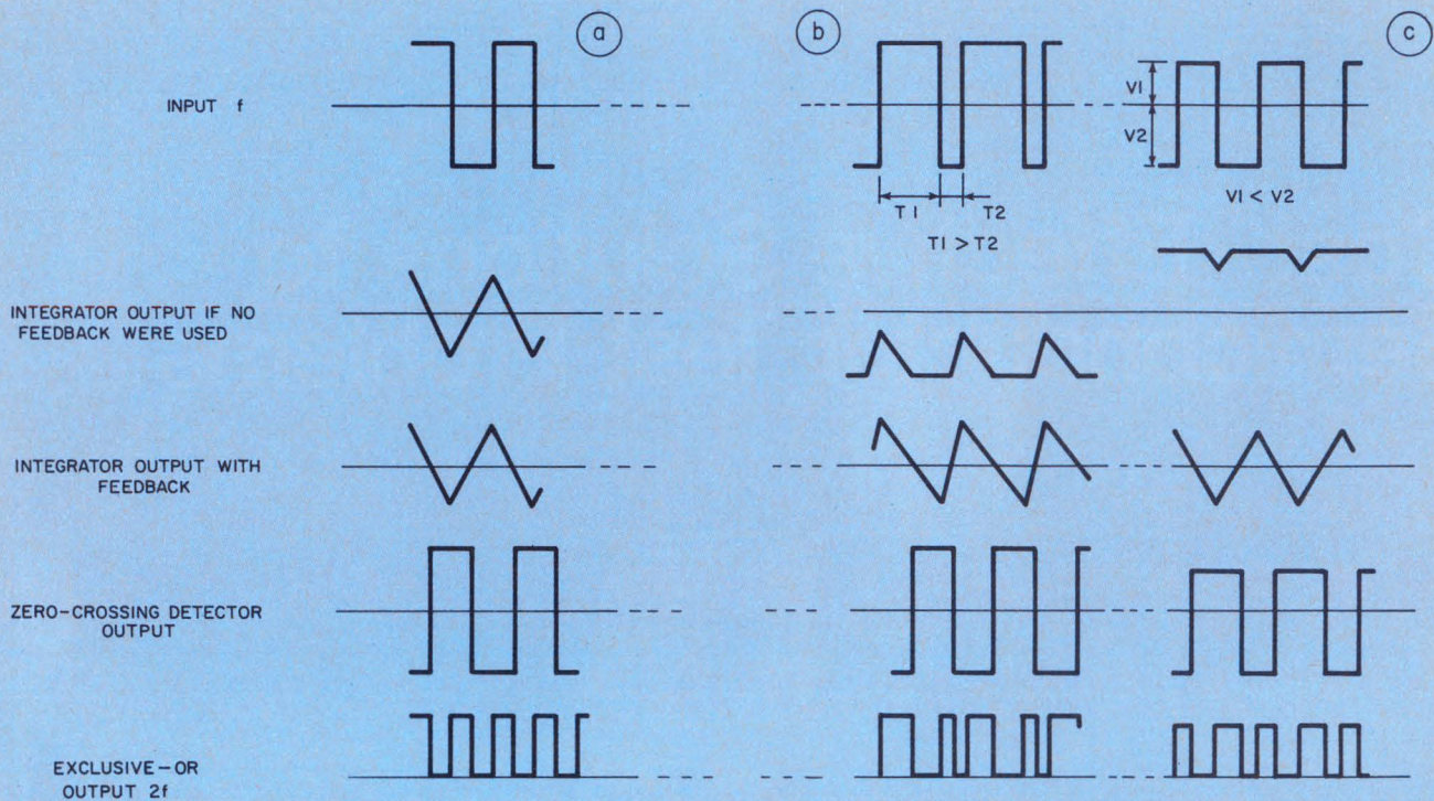
2. Both symmetrical signals (a) or unsymmetrical signals (b) and (c) are readily frequency-doubled.
