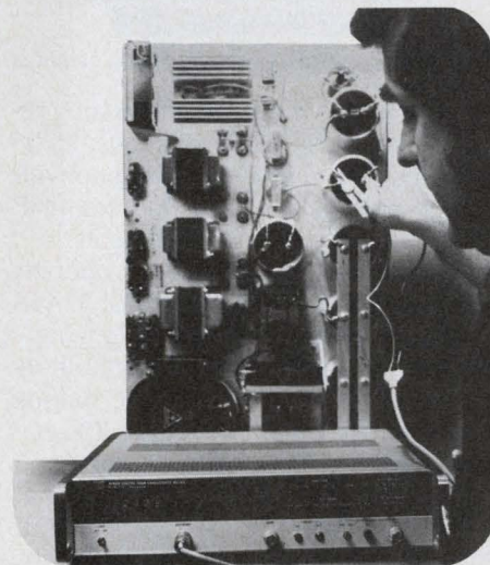
Here, the 4282A digital meter checks some tantalum capacitors.
