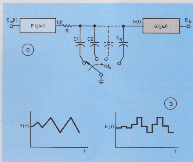
2. One resistor and N identical capacitors comprise the commutative filter (a). Each of the N contacts is closed periodically, one at a time. In effect, f(t) is sampled at the rate Nf_s . If the period of f(t) equals 1/f_s , the output h(t) resembles f(t) but in a sample-and-hold form (b). But the filter sharply attenuates frequency components not in the vicinity of \omega_s .
