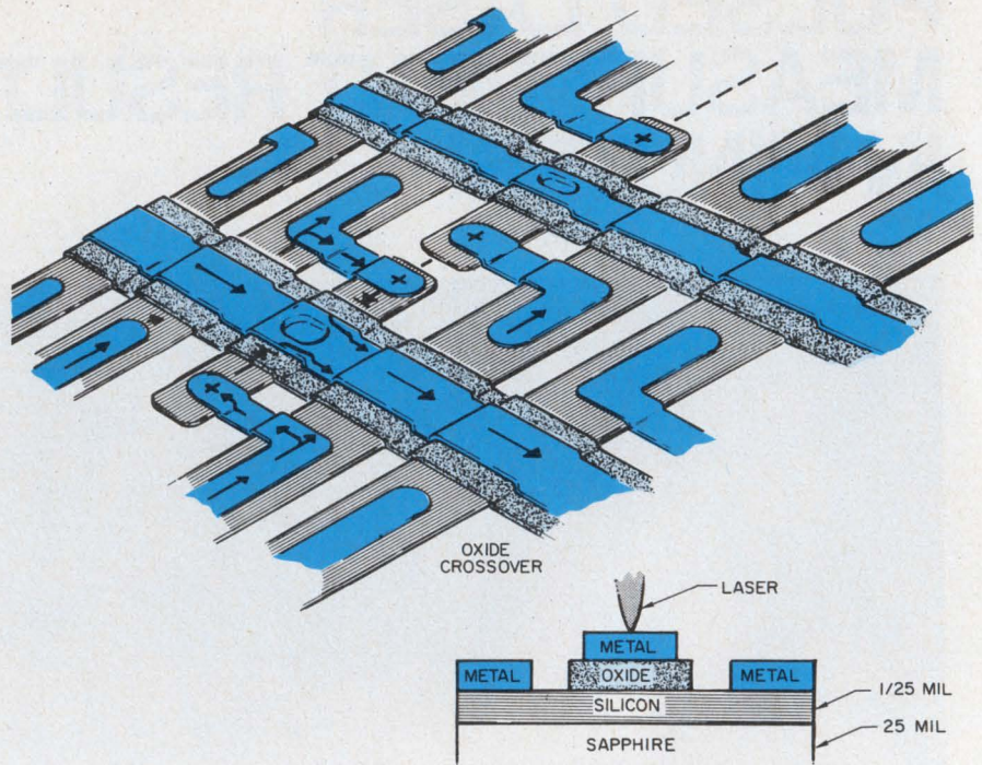
SOS programmable logic array from Rockwell International is composed of diodes and resistors. The thin silicon film on the sapphire substrate permits quick custom laser encoding via selective removal of silicon.
