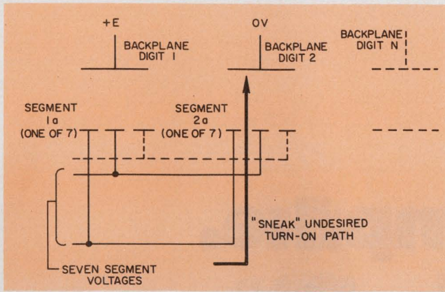
10. LCDs don't multiplex easily. Without the use of additional circuitry, LCD segments in multiplexed operation tend to turn on when they shouldn't.
