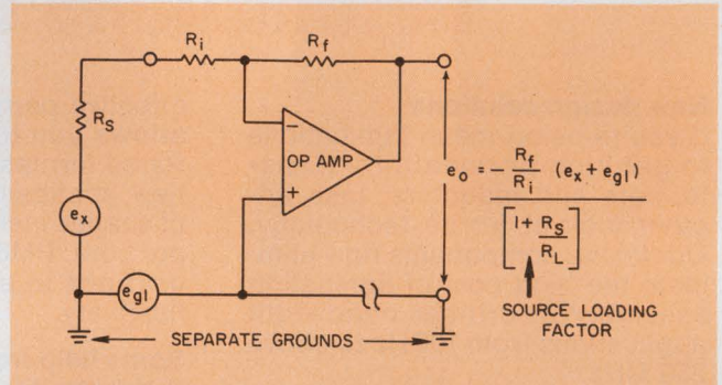
1. Single-ended inverter op amp just amplifies the ground-loop voltage along with the signal.
