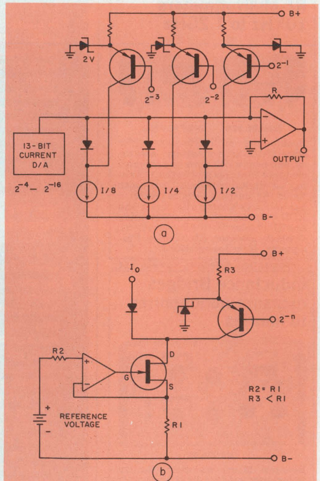
2. If current steering is used for constant-current sources (a) high precision DACs can be built. The reference (b) used by the Hybrid Systems DAC provides a stable current level.
