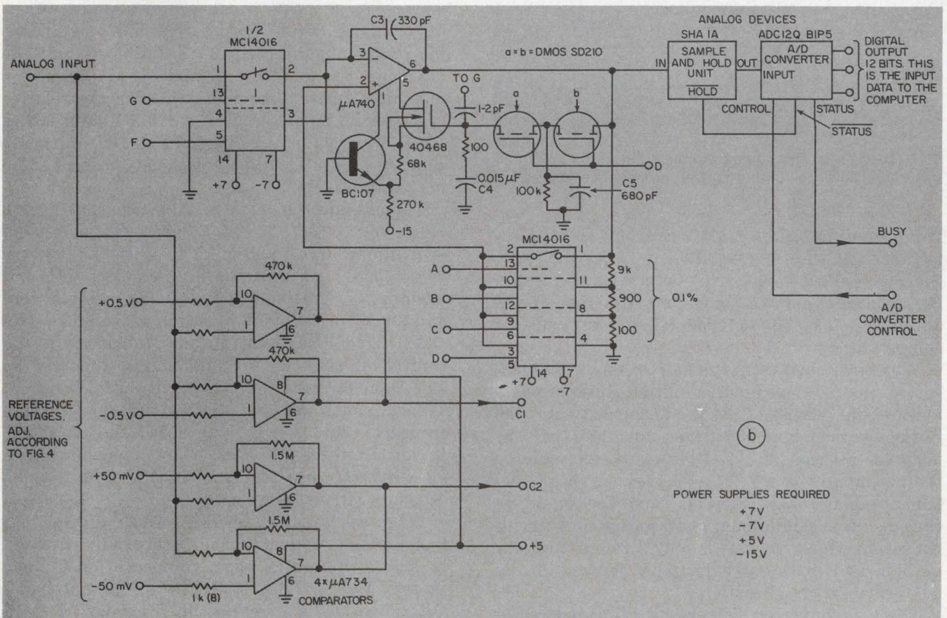
2. The complete autoranging amplifier can be divided into two sections. The digital control section (a) interfaces the analog switches to the computer, while the analog section (b) amplifies the input signal.
