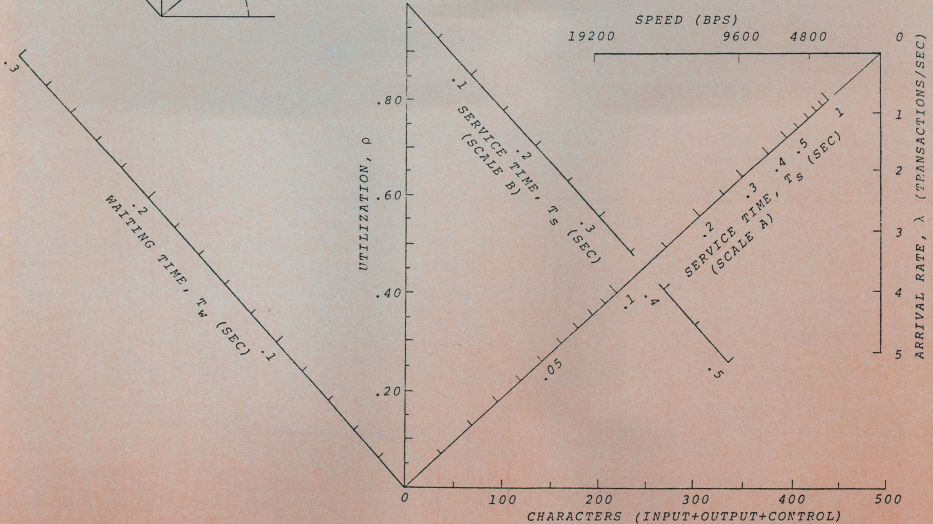
2. Nomograph for mean waiting time. The loop's response time equals the sum of the waiting time, service time and controller delay.
