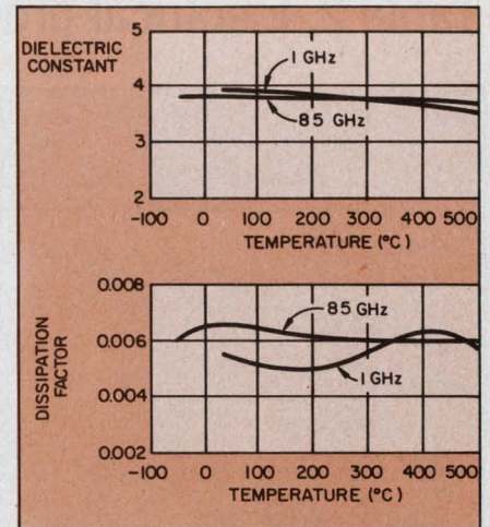
8. Silicones display only slight changes in electrical properties over a wide temperature range.
