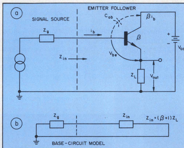
1. The emitter-follower transistor circuit (a) provides large current gain, \beta , but can be unstable at certain frequencies. A simplified base model (b) allows easy determination of the conditions for stability.
