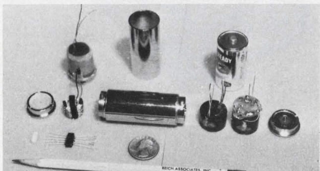
Highly compact dc-to-dc power supplies, such as this 16 kV at 1 \mu A unit produced by Reich Associates, can operate from a 1.5-V source.
