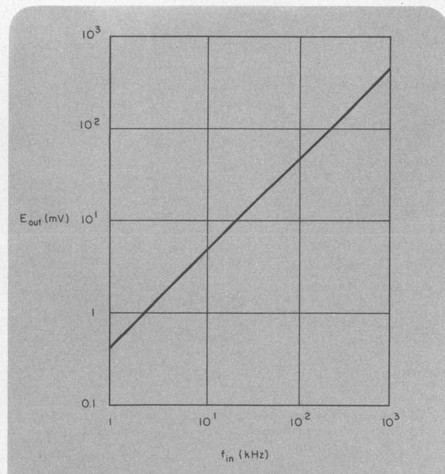
2. Linearity with an error of less than 0.072 percent is attainable over at least three decades of frequency with this very simple CMOS circuit.
