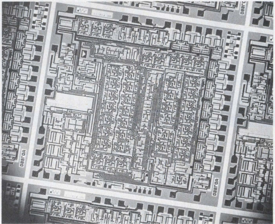
Analog Devices' 13-bit CMOS ADC uses a quad-slope conversion technique.
