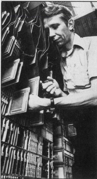
Technician inserts circuit packs in the 1A stored-program control unit of Bell Telephone's 4 ESS for long-distance calls. The hanging cables are connected to test equipment.
