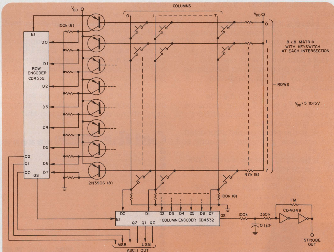
1. Few components are needed to build this 64-key ASCII encoder. Low-power consumption—only nano-
