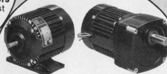
42R Induction Motors and Parallel Shaft Gearmotors. Motors 1/20 thru 1/4 Hp. All A-C winding types. Gearmotor ratios to 300:1. Helical steel gearing.
