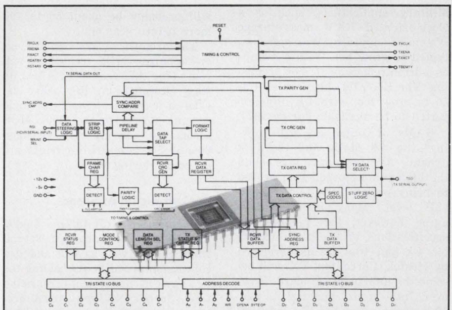
By handling both bit and byte synchronous data, the COM5025 developed by SMC Microsystems offers the designer a choice of protocols, full or half-duplex operation, and even some self-checking capability.
