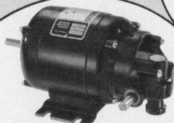
N-1R Gearmotors. Single and double reduction right angle worm gearmotors. Stock ratings thru 5 Lb-in. Many ratios available for a wide range of speed selection.
