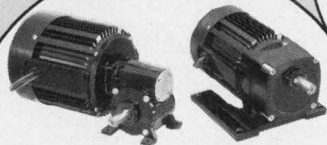
48R Induction Motors . . . Right Angle and Parallel Shaft Gearmotors. Motors thru 1/3 Hp. Available 115/230V in 50 or 60 Hz. Gearmotor ratios thru 30:1.
