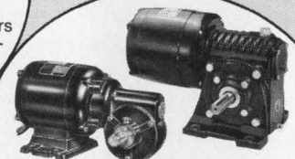
Single Reduction Right Angle Worm Gearmotors. 6 frame sizes with stock ratings to over 200 Lb-in. Ratios thru 60:1. Ample reserves for overloads.
