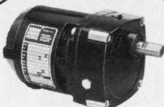
N-1D Gearmotors. Parallel shaft helical and spur gearing. Ratings thru 40 Lb-in. Ratios thru 900:1. Only 3.41" square.
