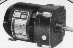
N-1S Gearmotors. Special purpose gearmotors for applications not requiring the ruggedness of the N-1D. In-line shaft. Only 3.41" square. 100 lot minimum order.
