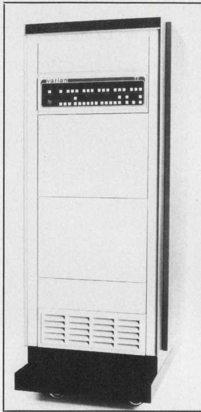
3. The V77-600 is the top of Varian's latest line of minicomputers. It has features originally introduced on large computers, such as user micro-programmability, and a cache-memory. It also uses memory mapping to address one-million 16-bit words.
