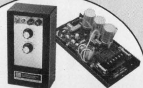
Encased and Chassis-type Speed Controls for Permanent Magnet Drives. Provides not only speed adjustment, but also adjustment of torque output. Available from stock.
