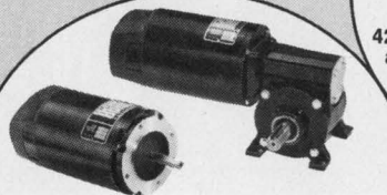
New 32A Permanent Magnet D-C Motors and Right Angle Gearmotors. Only 3.55" in diameter. TENV Hp 1/12 thru 1/8 at 2500 Rpm. Many gear ratios available.
