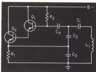
SIMPLIFIED CIRCUIT, a Clapp oscillator—Fig. 1
