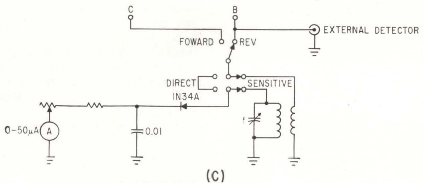
COMPLETE CIRCUIT components: coupler box (A); bridge section (B); meter circuit (C)—Fig. 2
