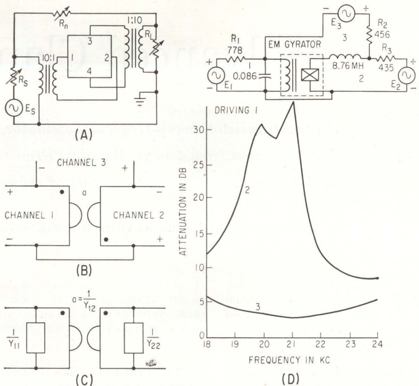
RESISTIVE network (A) neutralizes Hall isolator. Adding third terminal pair to ideal gyrator (B) forms circulator. Nonreciprocal system (C) is interpreted as ideal gyrator with complex gyration resistance. Characteristics are shown driving one channel of EM circulator (D)—Fig. 4
