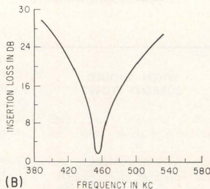
IDEAL transformer is contrasted with ideal gyration (A). Butt-joint (B) and composite-beam (C) gyrations are shown with their response curves—Fig. 1
