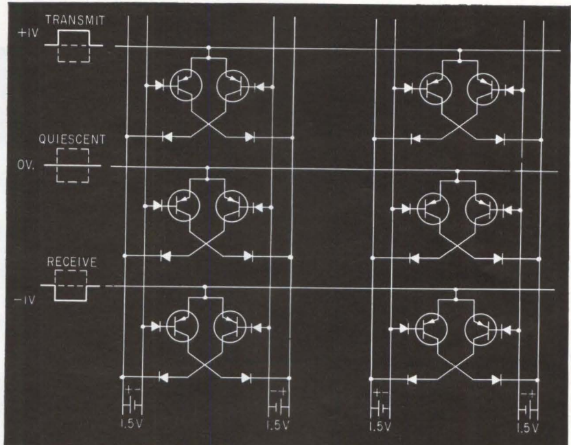
THREE STORAGE registers of two digits each. Flip-flops are drawn with resistors omitted—Fig. 2
