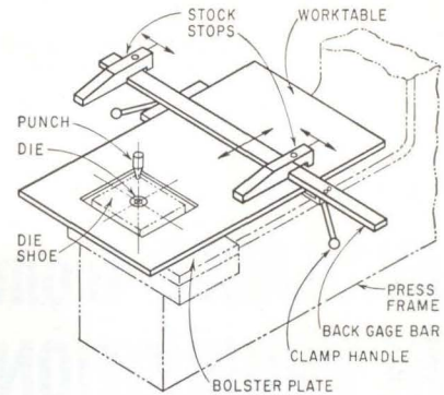
STOCK STOPS and back-gage bar of hydraulic press create a rigid nest for punching holes in remaining pieces of a run after first piece (template) is used to setup their positions
