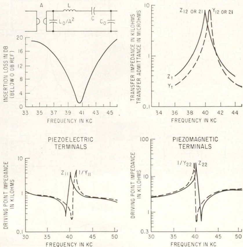
EQUIVALENT circuit at upper left is verified by data plotted for 40-Kc composite beam length expander—Fig. 2
