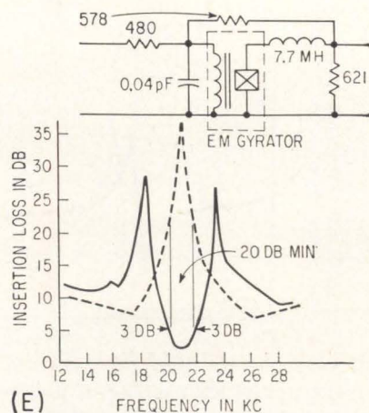
STRUCTURE, parameters and equivalent circuit are shown for a Hall gyrator (A). Isolation at one frequency (B) is obtained by neutralizing with capacitor at peak transfer admittance, while arrangement at (C) permits a resistor to be used. Fourth-order neutralizing network is used with broadbanded gyrator (D), while resistive network (E) is used with 20-Kc broadbanded isolator—Fig. 3
