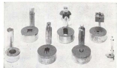
SPECIAL SHAPES and forms for punches and dies used in hydraulic press are readily made from standard drill rods and cold-roll bar stock
