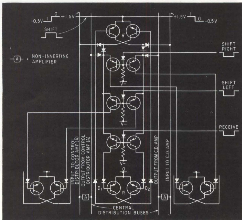
ARITHMETIC register consists of a pair of flip-flops R and \bar{R} . Flip-flop \bar{R} is the receiver and connection to the proper register for receiving is made through the coincidence gates shown—Fig. 4
