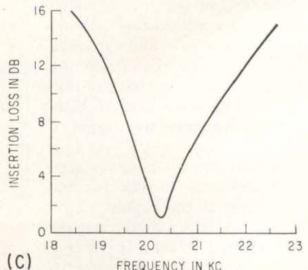
IDEAL transformer is contrasted with ideal gyration (A). Butt-joint (B) and composite-beam (C) gyrations are shown with their response curves—Fig. 1
