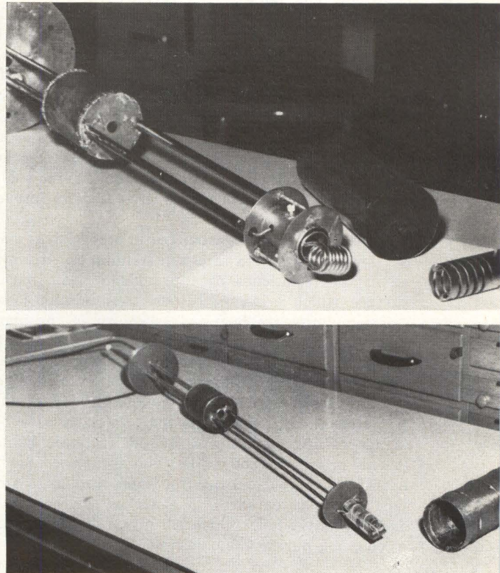
MOUNTING and coupling probes for 58-Mc (above); solid dielectric configuration (below)
