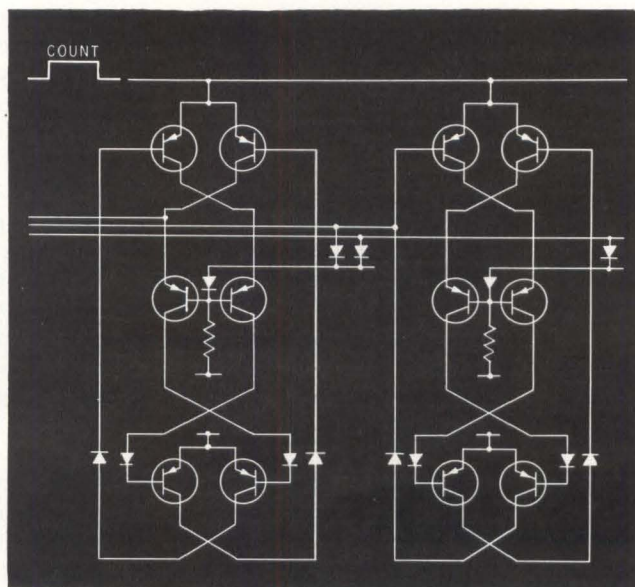
REGISTER arranged for counting. Flip-flops are drawn in simplified form—Fig. 5
