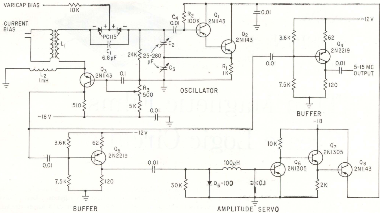
SWEEP FREQUENCY OSCILLATOR with output buffers and amplitude servo—Fig. 2
