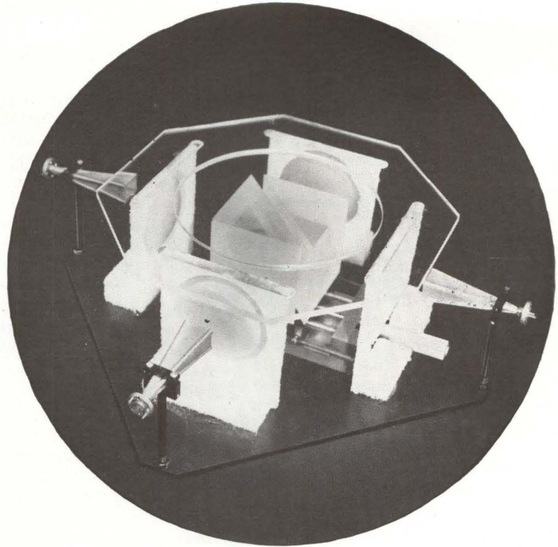
MM WAVE directional coupler—see Fig. 5 on p 36
