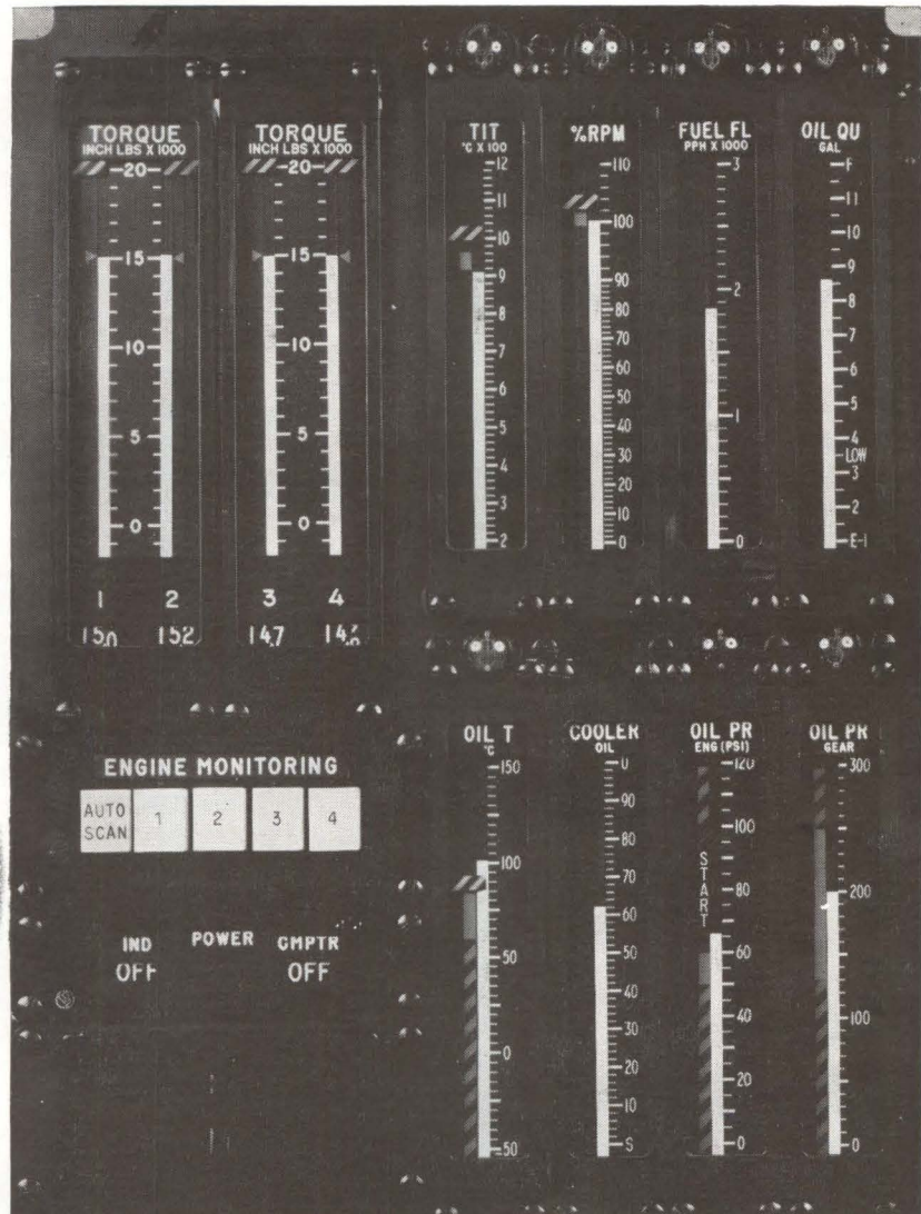
PANEL DISPLAY shows torque for each of the four engines and only the worst parameters during each scan cycle—Fig. 2
