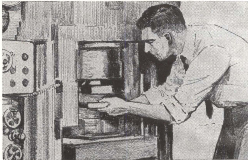
POWDERED COPPER is compressed at 50,000 psi into circuit-groove die prior to sintering in a reducing atmosphere. Rubber mat is used directly over circuit die
