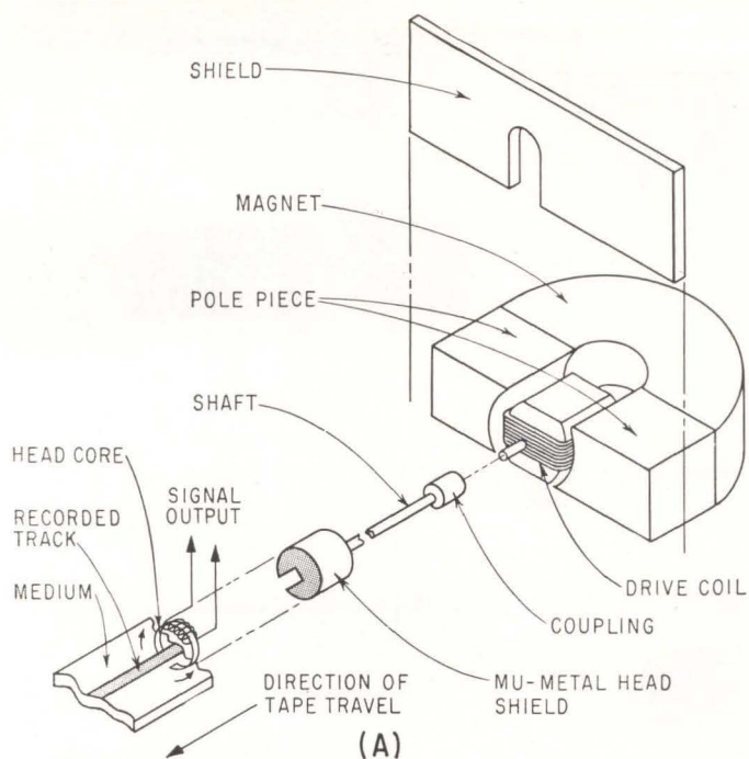
SCANNING HEAD mechanical arrangement (A) produces one pulse period when recorded track is in center of scan (B), another when track is above scan center (C) and a third when below scan center (D). The track is recorded by applying a d-c voltage to a conventional recording head—Fig. 1
