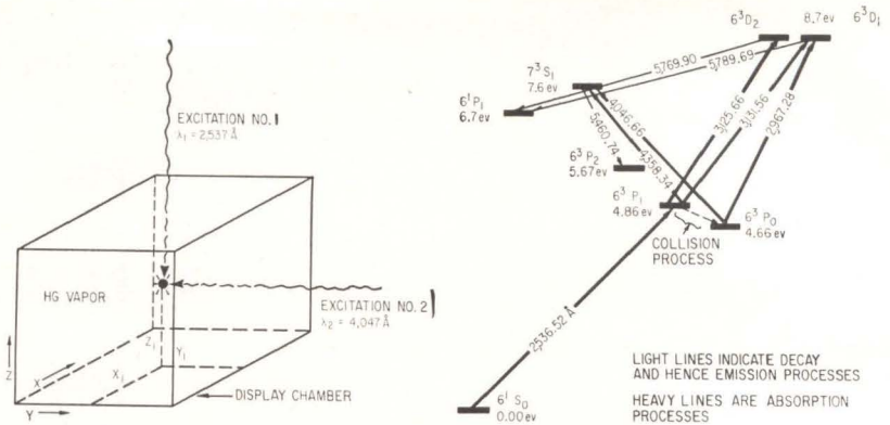
DUAL EXCITATION in space of mercury vapor, (A); mercury energy level diagram showing pertinent states of atom excitation, (B)—Fig. 1
