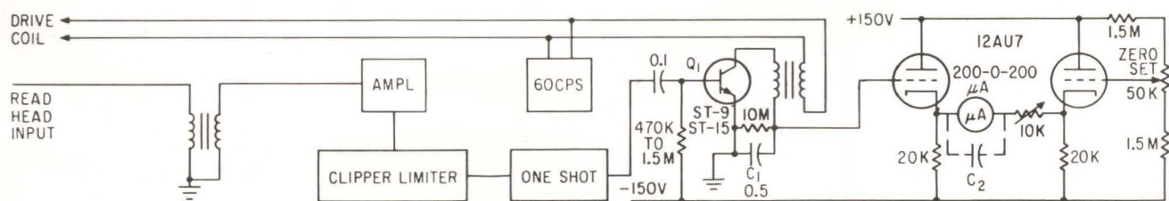
PICKUP HEAD signals are amplified, clipped and trigger a multivibrator. Pulses are detected and measured by a vtvm. An external recorder can be connected between vtvm cathodes—Fig. 3
