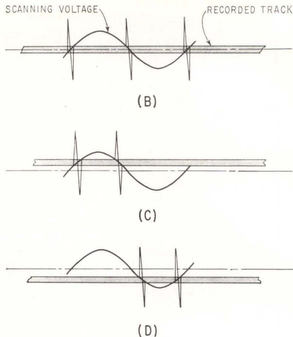
SCANNING HEAD mechanical arrangement (A) produces one pulse period when recorded track is in center of scan (B), another when track is above scan center (C) and a third when below scan center (D). The track is recorded by applying a d-c voltage to a conventional recording head—Fig. 1
