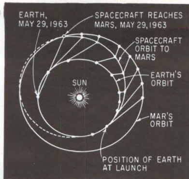
ORBITS of Mars probe and of the planet Mars projected on the plane of earth's orbit. Spacecraft will take about 16 months for a complete orbit around the sun
