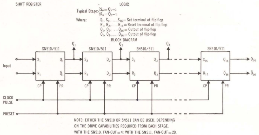
Right: 16-stage shift-register block diagram incorporates 16 SN510 or SN511 semiconductor networks. Inset photo shows actual-size shift-register card built from the logic diagram.
