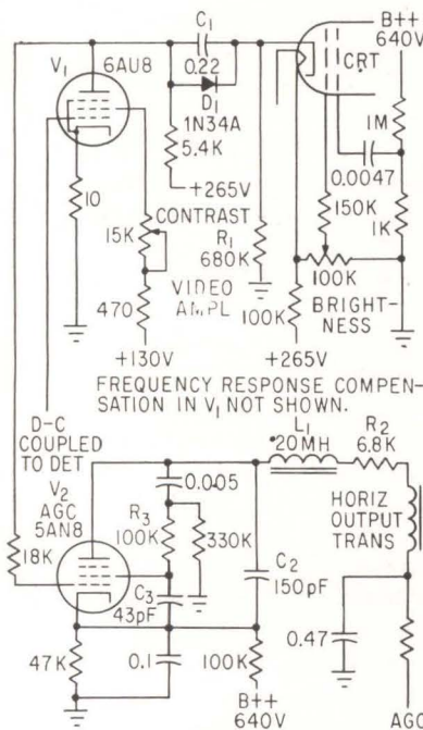
COMPOSITE a-c/d-c video coupling and keyed age produces nearly ideal picture signal—Fig. 3
