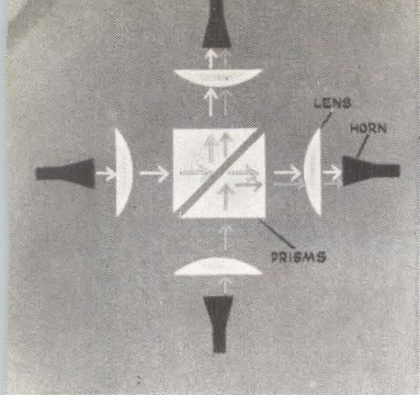
DIRECTIONAL coupler splits power equally between two output ports—Fig. 5
