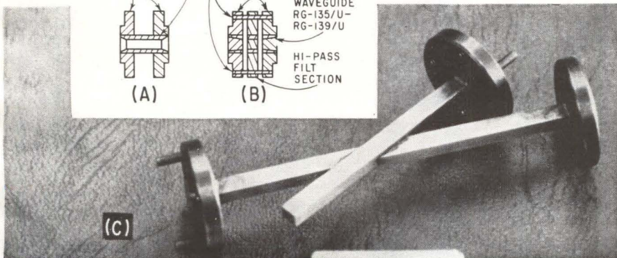
WAVEGUIDE FILTER in (A) is swaged, as are the two end pieces of the 3-piece waveguide filter (B). A Bethe-hole directional coupler is shown in (C)—Fig. 3
