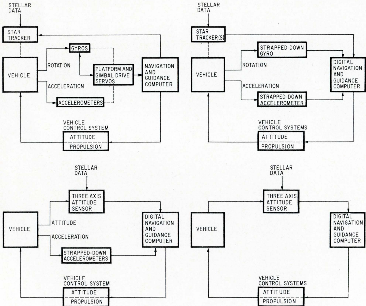
Four guidance systems. At top left, gimbals, gyroscopes and accelerometers are required. System at top right performs gimbal functions with a digital computer. At bottom left, TAAS does away with gimbals, gyros and trackers; only one angle encoder is required. Attitude-control system at bottom right does not require accelerometers.
