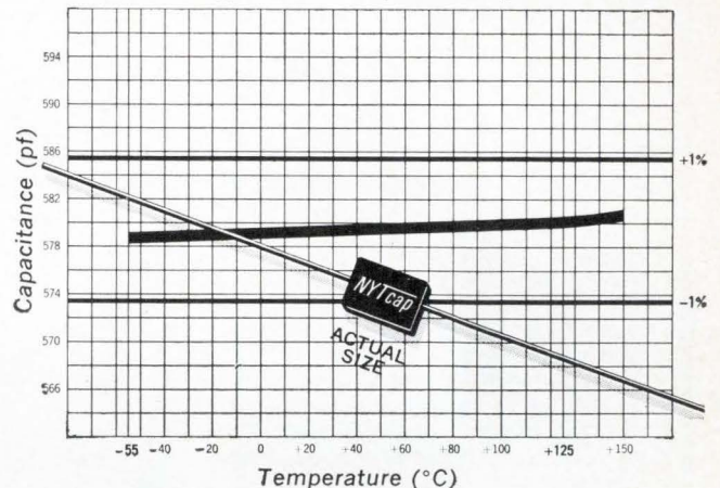
Typical NYTcap Stability
