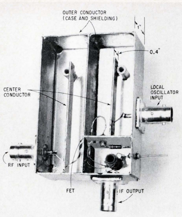
Strip transmission line construction of the uhf mixer. Two outer ground plane conductors, 1.0-inch high, form the case and the internal shielding for the circuit. Center conductors are 0.4-inch high.
