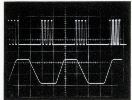
Single-Input Dual-Beam Displays. The upper beam shows bursts of 2.5 MHz pulses on Time Base A with time variation between bursts. This shows up as increasing time-jitter between the first and successive bursts. The lower beam shows B Sweep (0.1 \mu s/cm) delayed by A Sweep and triggered on the second pulse of the last burst to provide a jitter-free expanded display of the A Sweep intensified zone. The use of only one probe and one plug-in input simplifies signal connection and provides minimum loading on the source.
