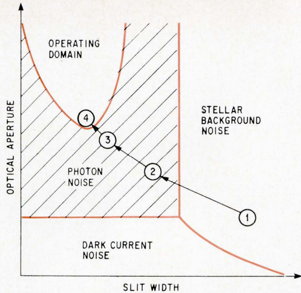
Different kinds of noise are dominant for each combination of slit width and aperture size. Numerals refer to iterative steps in the automatic design program to reach that point in operating domain at which aperture is minimal.
