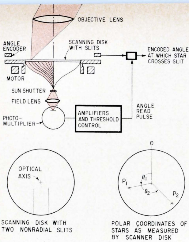
Three-axis attitude sensor consists of a lens, scanning disk and photomultiplier. Slit configuration shown can provide, through mathematical transformation, the polar coordinates of each detected star.
