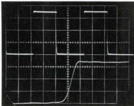
Sampling and Real-Time Displays. Upper beam shows a square wave at 1 \mu\text{s}/\text{cm} as applied to a Type 1A2 Plug-In. The lower beam shows the risetime of the same pulse at 1 \text{ns}/\text{cm} as provided by a Type 1S1 Sampling Plug-in.
