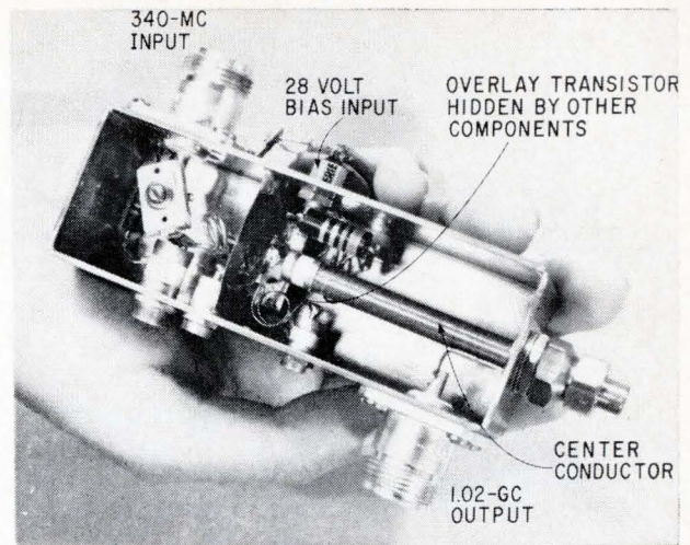
Combination amplifier-tripler uses one overlay transistor as both amplifier and frequency multiplier. The unit measures approximately 4 by 1¼ by 1¼ inches.
