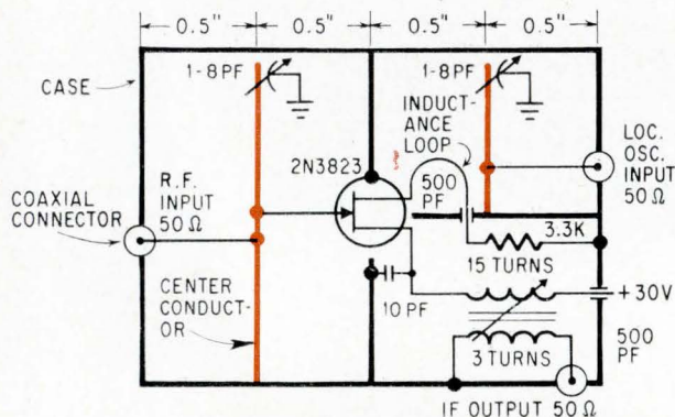
Schematic of FET mixer corresponds to actual layout of circuit. Heavy lines represent outer conductors of strip transmission lines. Lines in color represent the strip line's smaller center conductors.
