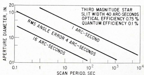
Relation of minimum aperture to scan period in information-limited scanning system. Longer scan permits the aperture, and therefore the sensor, to be smaller.
