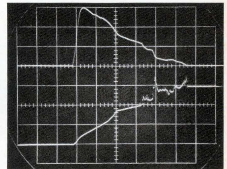
Simultaneous Single-Shot Displays. Current versus voltage display of a .75 ampere, fast-blow fuse during destructive overload. Both beams are driven by B Time-Base at 50 \mu\text{s}/\text{cm} which is delayed by pre-triggered A Time-Base to provide base reference lines before and after the event. The upper beam shows the current waveform at 30 A/cm while the lower beam shows the corresponding voltage across the fuse at 100 V/cm.
