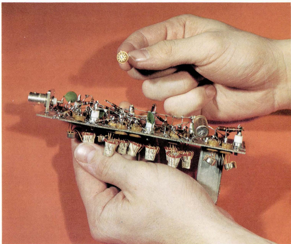
Breadboard version of the integrated circuit compared with the actual integrated circuit. Breadboard was built first to establish the IC's performance goals.
