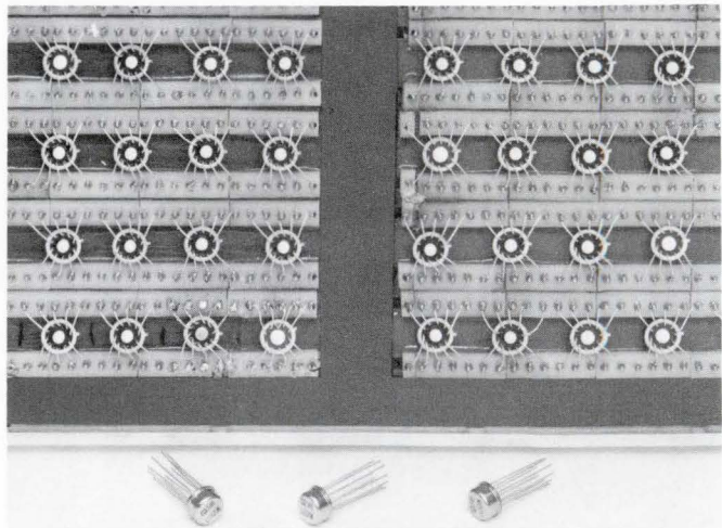
Signetics LU-Series Utilogic elements in SOLAR System logic boards. Note novel upside-down mounting technique of TO-5 cans.
