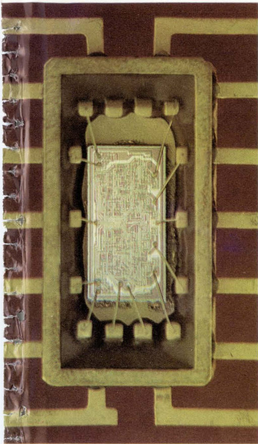
Sixteen bits of memory are packed into a chip by Texas Instruments.
