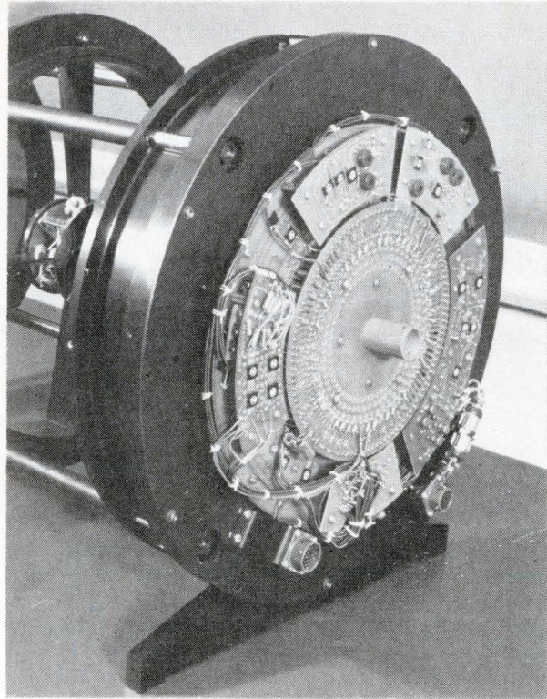
Molecular Infrared Track built by Westinghouse for airborne use. The system demonstrated the feasibility of using general-purpose chips to build prototypes.
