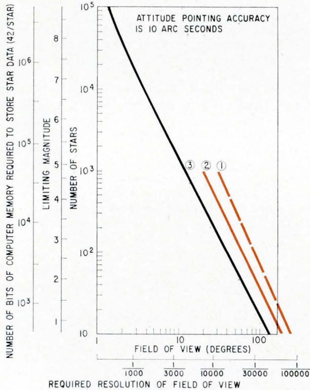
Design tradeoffs for three-axis attitude system. With wide field of view, the computer can operate with data on relatively few stars stored in its memory, and the detection system needs to consider only the brightest stars. However, this advantage requires high resolution in the field of view. Line 1 indicates conditions resulting in a 1.0 probability of finding three or more stars in field of view; line 2, probability of 0.9; line 3, an average of three stars.
