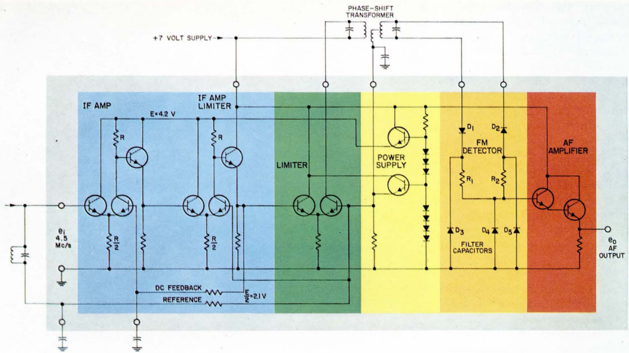
Functions provided by the chip are: blue, i-f amplification; green, limiting; orange, f-m detection; red, audio-amplification frequency. External components associated with the IC are shown outside of the color blocks.
