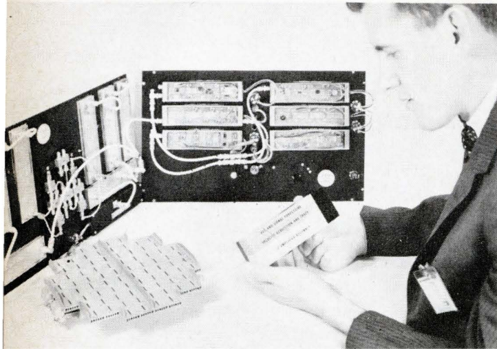
Doppler radar system , built for the Air Force, demonstrated that it was practical to mix Mirt and Lava chips in breadboarding prototype equipment. Breadboarded system is in background. Bill List holds actual-size model of final equipment.
