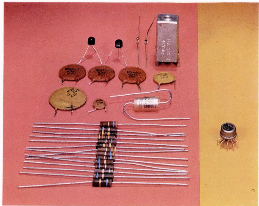
Integrated circuit replaces the discrete components shown. Eliminated are 2 transistors, 2 diodes, an interstage transformer, 14 resistors and 7 capacitors.
