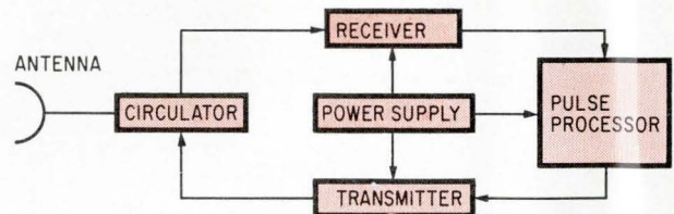
Simplified block diagram for a radar transponder. Pulse-processing portion of transponder consists of 11 sections, 8 of which can use the same multipurpose integrated circuit.
