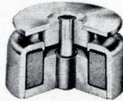
LEDEX FLAT-FACE PLUNGER (Short Stroke)
