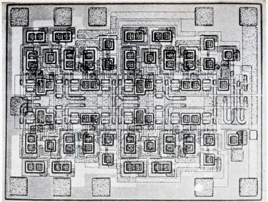
Array structure being developed by Motorola for fast memories. Second layer of wiring will connect this four-bit group to adjoining cell groups.
