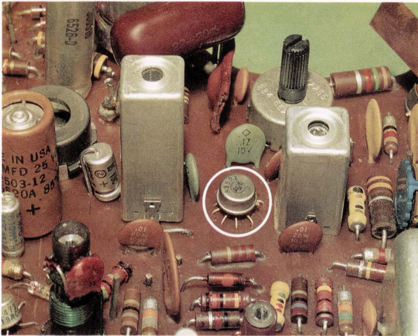
Integrated circuit in a production-line tv receiver manufactured by the Radio Corp. of America. Circle denotes the IC. Large cans are transformers.
