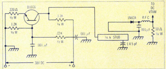
Test circuit—940 mHz oscillator
