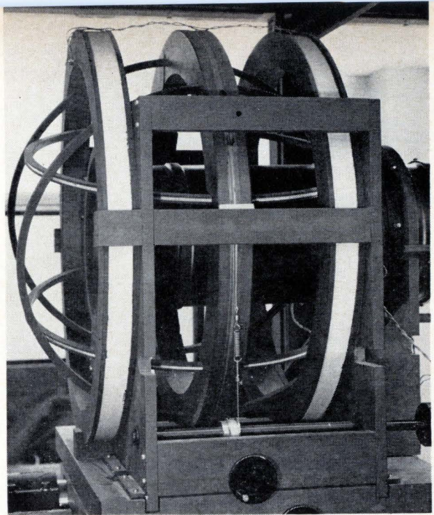
Large Helmholtz coils at the ends of the image section are the focusing coils. Between them is support ring. Two smaller pairs of coils are for vertical and horizontal deflection.
