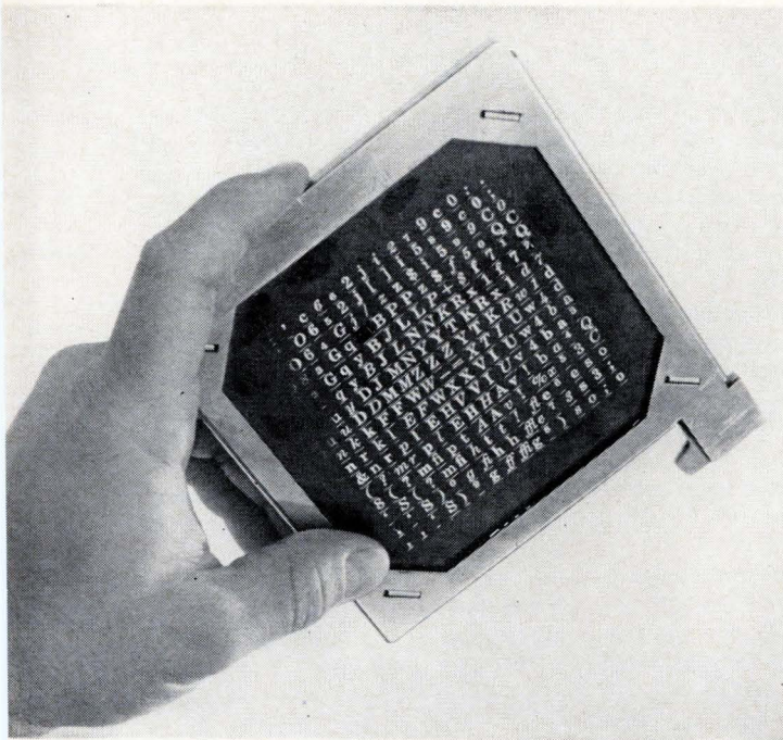
Character grid is a photographic store of 256 type characters. Linotron tube selects one character at a time which is transmitted as a video signal for projection onto crt display.
