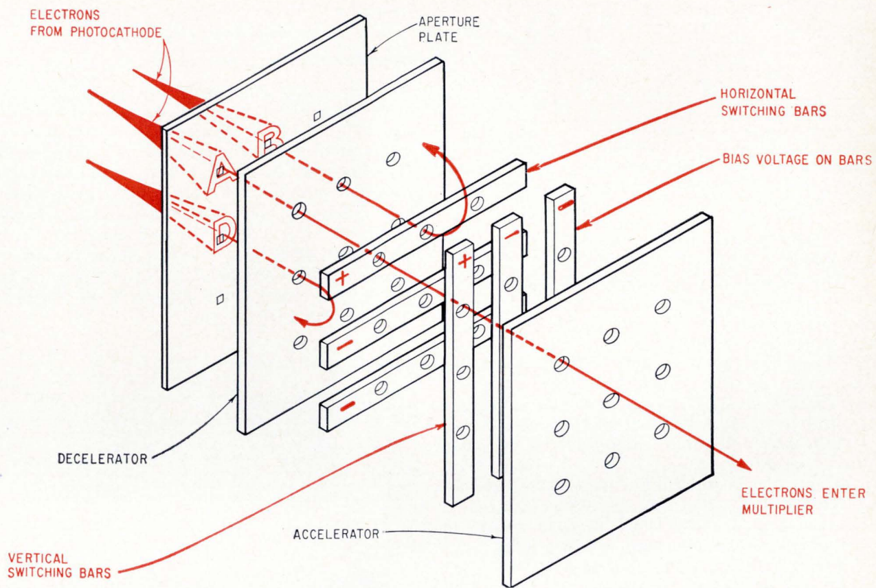
High voltage applied to one horizontal and one vertical switching bar select a beam carrying the video signal for a single character.
