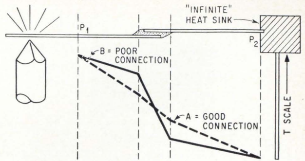
Spot weld quality is checked by infrared determination of the thermal resistance of the joint. A large thermal differential across the weld, line B, indicates a poor connection; a linear differential, line A, indicates a good one. The heat sink at the right speeds the transfer of heat through the joint.
