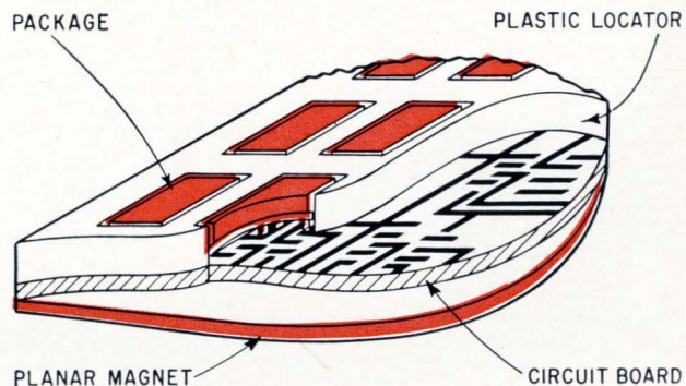
Individual packages are positioned for butt soldering by a molded locator as a planar magnet holds the packages in place. The same arrangement can be used to position packages during testing.
