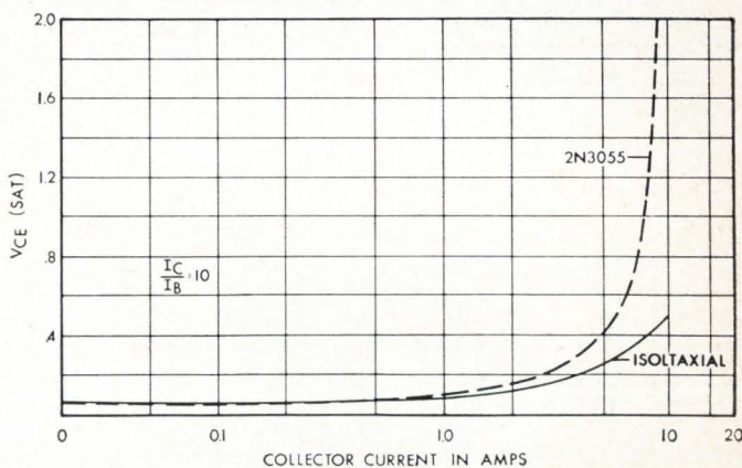
COMPARISON OF ISOLTAXIAL DEVICE TO COMPETITIVE 2N3055
