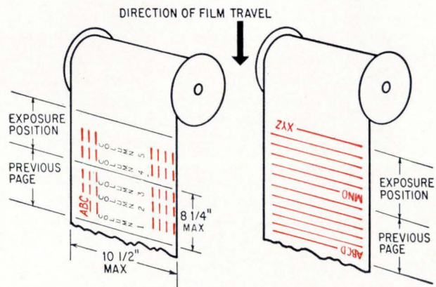
Normal printing mode on film (left) has crt display positioned on its side. This allows wide, multi-column pages to be printed. In turn-page mode (right) pages are composed after being rotated 90° so long lists of information can be printed.
