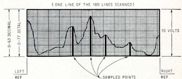
A typical oscilloscope trace of one scan line from the radiometer containing all 97 resolution elements. A complete scan for a circuit usually consists of 180 of these analog traces. The heavy lines indicate the four sample points in this trace whose values are entered into the processor's core memory. The left and right elements are reference values used to continuously calibrate the trace.
