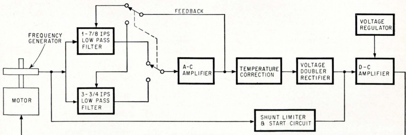
Running smoothly. Servocontrol for tape-recorder motor keeps tape speed constant and eliminates idlers, belts, and pulleys. Tape speed—either 1 7/8 or 3 3/4 inches per second—is set by switching in corresponding active low-pass filter.
