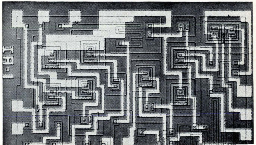
Chip for Sony's radio integrated circuit has nine npn transistors, four diodes, and 14 diffused resistors (shown in color). Transistors Q_1 , Q_2 , and Q_3 are audio stages; Q_4 is a temperature stabilization unit; Q_5 a detector; Q_6 and Q_7 i-f linear amplifiers; and Q_8 and Q_9 a Darlington i-f agc stage.
