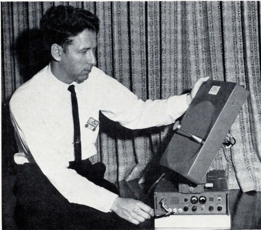
Small wonder —Harold V. Lind, program manager, adjusts antenna elevation of tiny terminal built by Hughes Aircraft.
