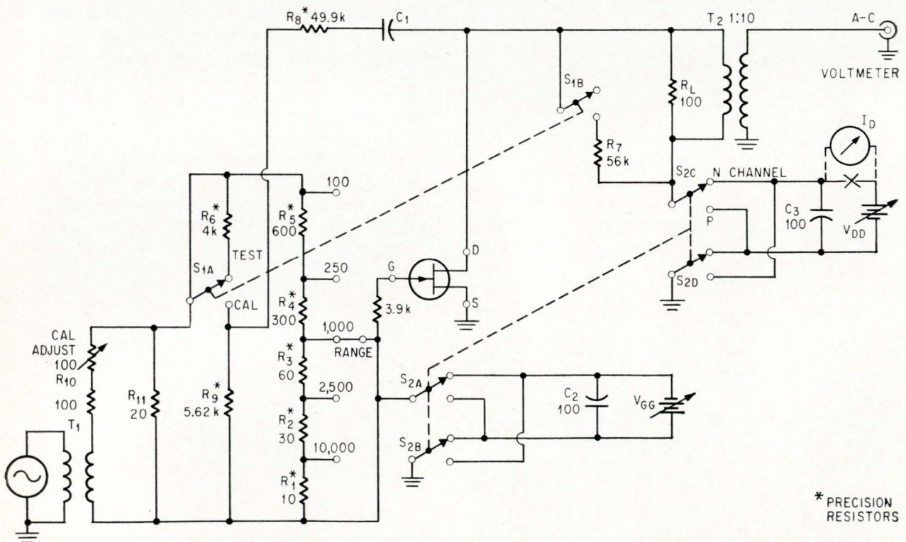
Improved test set for measuring g_{fs} includes a circuit that automatically compensates for most of the sources of errors. The new test set accurately measures a wide range of values of transconductance. The range switch at the gate of the device being tested accommodates the test circuit to the type of voltmeter used.
