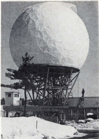
Under cover. Antenna at Mitre Corp.'s Bedford site now sports a radome.
