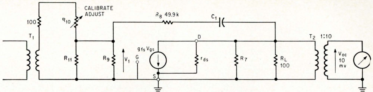
Simplified a-c circuit represents the test set in the calibrate mode. V_1 is adjusted for a full-scale deflection on the meter, and R_0 is selected to simulate the loading of the range attenuator when the set is placed in the test mode. This prevents V_1 from changing when the mode is switched.
