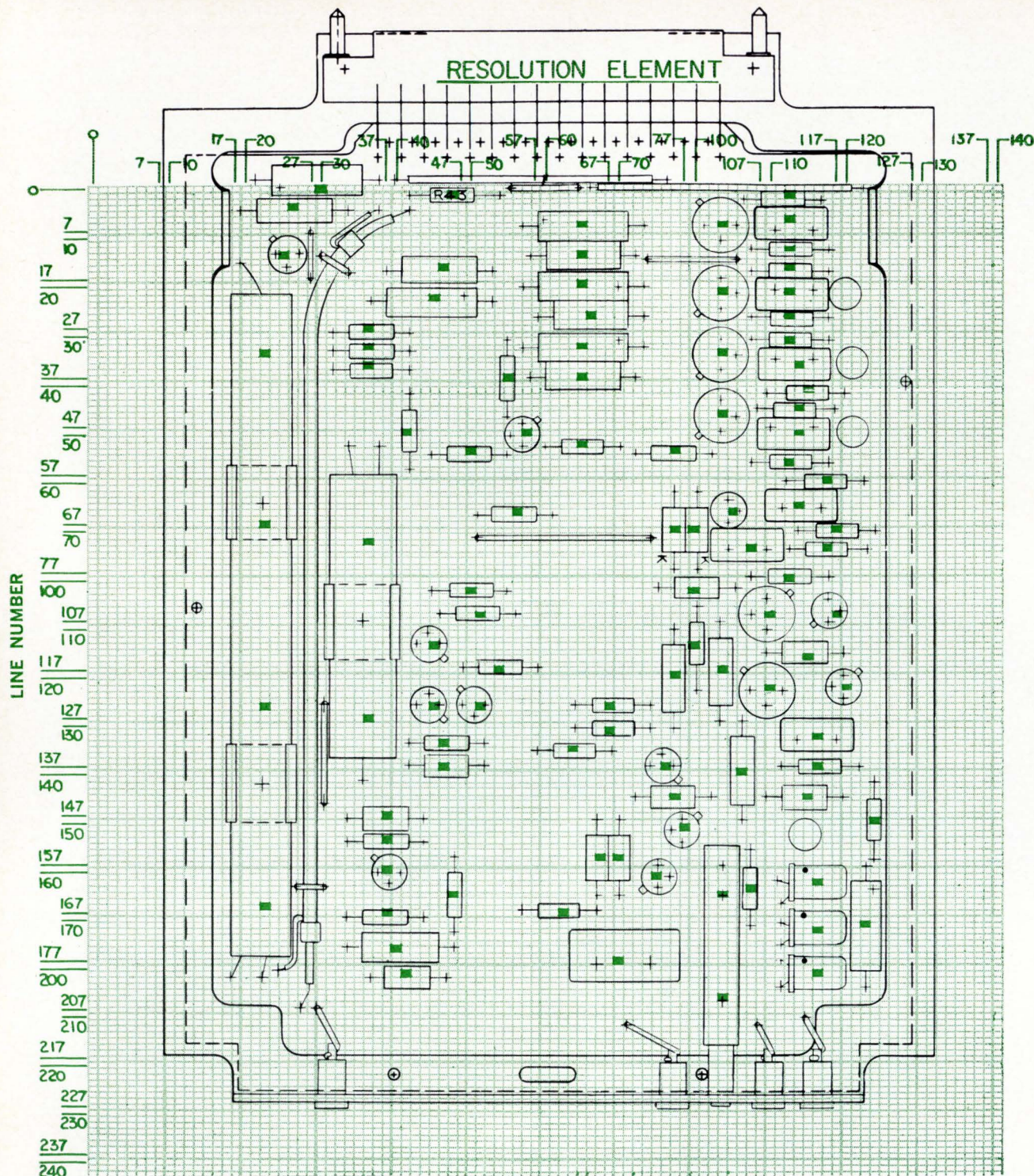
Layout of printed-circuit board and grid overlay used to select the points to be sampled from the radiometer scan. The dark squares in the overlay define the line and element numbers to be programmed into punched tape.
