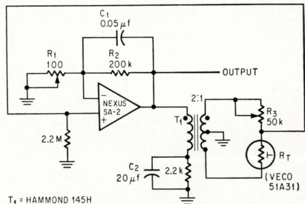
T_1 - HAMMOND 145H
