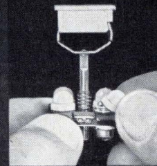
COMPLETELY REMOVABLE FRONT-END ASSEMBLY Will not actuate switch when replaced.
