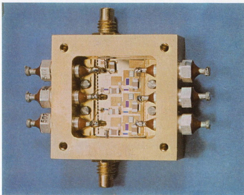
Power block. Hybrid microwave IC amplifier is designed for 25-db gain over the band from 10 Mhz to 1.3 Ghz.
