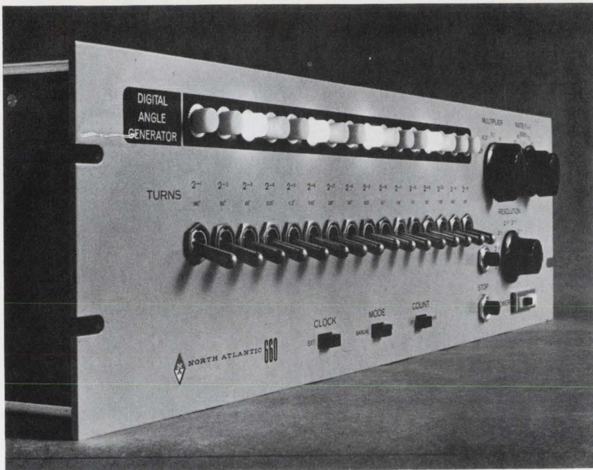
Computer's pal. Angle generator frees computer from the repetitious job of sending digital positioning commands to synchro or resolver converters.
