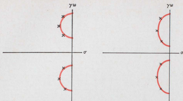
Pole-zero diagram. Poles on a semicircle produce a flat response while the poles on a semiellipse produce constant time delay.
