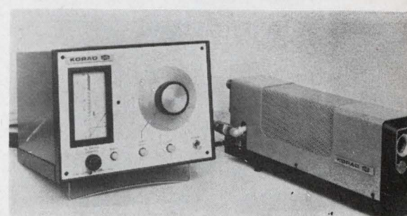
Trimmer. First application for laser is in component modification.
