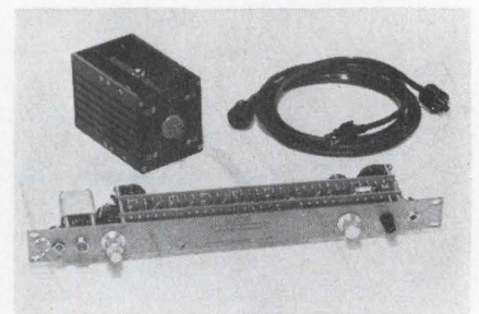
Equalizer. Correction amplifier with power supply and connecting cables is used at remote f-m sites.
