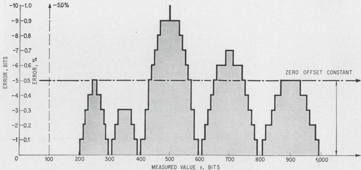
Error histogram. To see how well the linearization circuit actually works, error is plotted throughout the range. This histogram is for the square-root linearizer. The error is always negative, and its maximum value is -1\% . The error is larger below 200, but is disregarded. Because the error exceeds the prescribed \pm 0.5\% , an extra five bits is added to the BCD counter using the shifting circuit to translate the reading +0.5\% .
