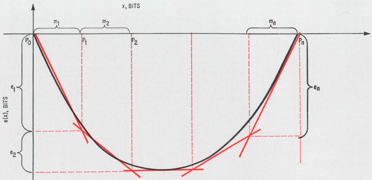
Plot and correct. Difference between nonlinear characteristic and its linearized equivalent equals the amount of correction, e(x) . Straight lines approximate the correction curve, and are used in circuit design.
