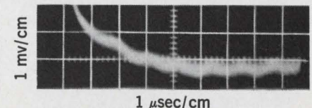
Response of D/A converter output to a full-scale change of 10 volts.
