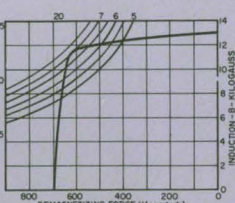
Demagnetization vs energy output, Alnico 5-7
