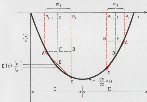
Like triangles. Geometry applied to correction curve aids development of error equations on page 121.
