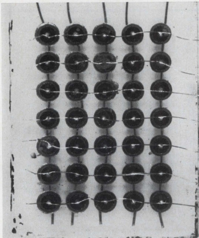
Dot array. Five-by-seven array of injection electroluminescent diodes was batch fabricated in single wafer of gallium arsenide phosphide. The diodes are individually addressable through x-y contact lines, which were soldered in place in earlier versions, but are now vacuum evaporated.
