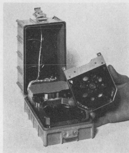
Airborne. Small cartridge recorder stores 130 million bits of data.
