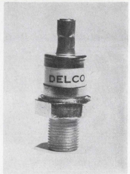
On guard. The DRZ-250, a diffused-junction, silicon device, handles 250 watts of continuous power.
