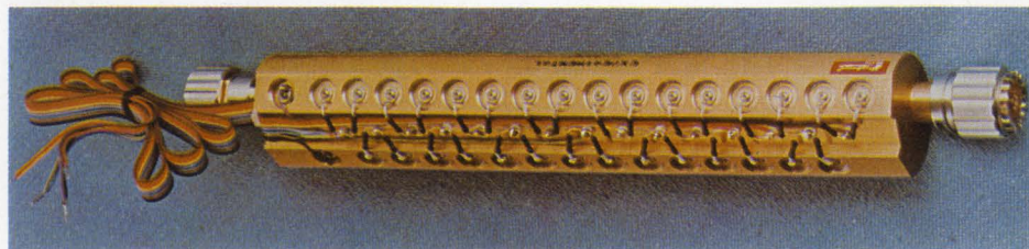
C-band shifter. By using 15 pairs of p-i-n diodes as switches, the device can introduce phase shifts in 22.5° steps up to 337.5°.
