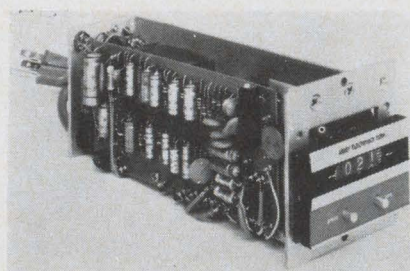
Inky. Printing wheel connected to readout provides permanent record.
