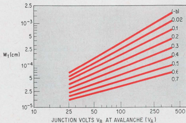
Intersection. After measuring the two diode parameters, V_A and b , one can use this graph to find the depletion width, W_1 .
