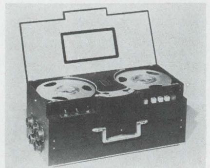
Earthbound. Portable 8-inch reel recorder has data capacity of 14-inch ground station equipment.
