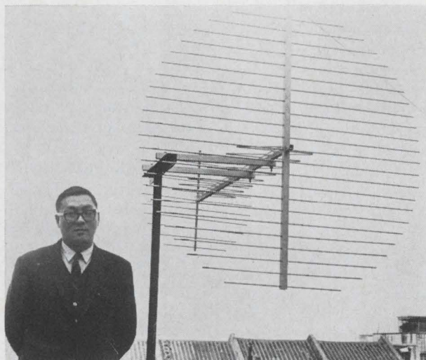
Reflective. Shiu-chang Loh added a plane reflector to an endfire antenna to get a backfire array that improves gain by 3 decibels.
