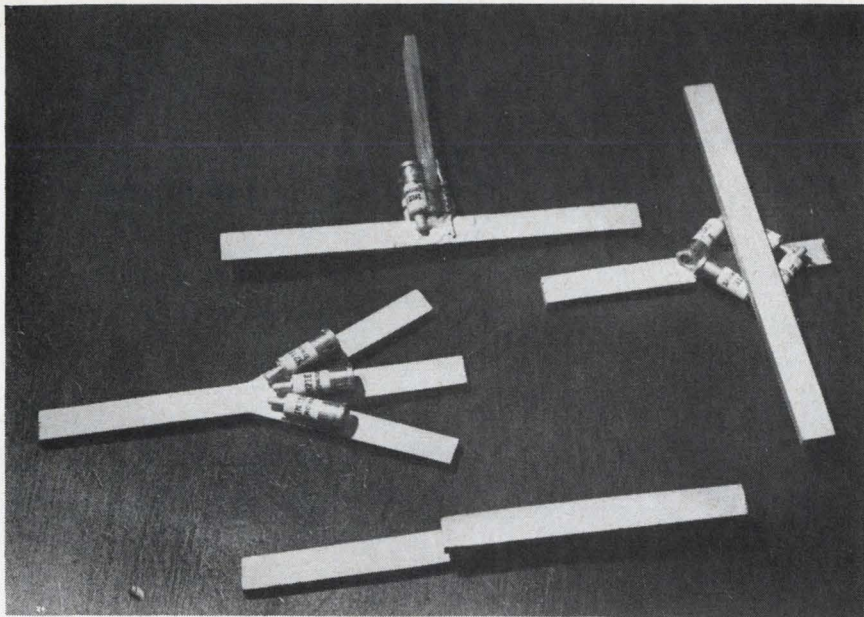
Assortment. Logic blocks for demonstration microwave computer are made of Fiberglass that's coated with conductive paint and point-contact diodes.
