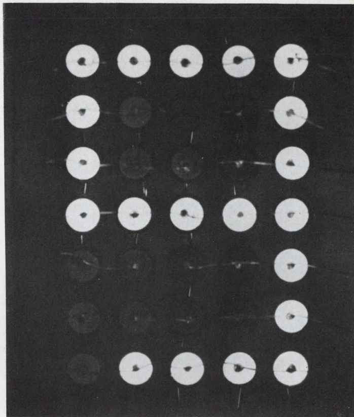
Dot array. Five-by-seven array of injection electroluminescent diodes was batch fabricated in single wafer of gallium arsenide phosphide. The diodes are individually addressable through x-y contact lines, which were soldered in place in earlier versions, but are now vacuum evaporated.
