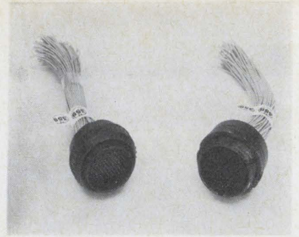
Mark 4. High-density connector has a shrinkable Teflon sleeve around each contact for insulation and support.
