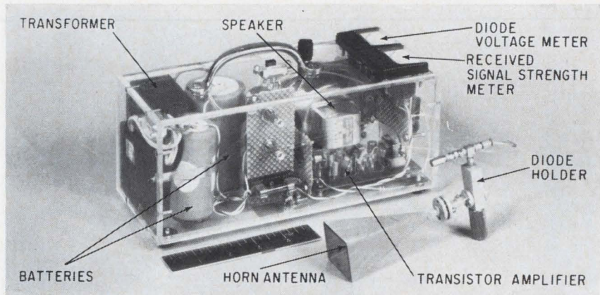
Electronic eyes. Doppler radar designed at Bell Labs demonstrates the use of a limited space charge accumulation diode to simultaneously oscillate, mix, and amplify a signal. The developers say the portable unit could be used by the military and as an aid to the blind.
