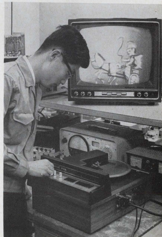
Video plateau. Television signals stored on record-like sheet of magnetic material can be played back instantly—fast or slow.
