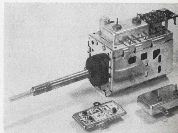
Replacement. Thick-film module, front, contains electronic elements of tuner
