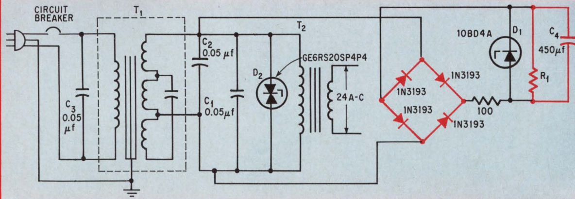
Voltage reduction. Rectifier and its RC load bleed the a-c filter and keep the primary voltage on transformer, T_2 at 117 volts. Thus, equipment that operates off T_2 is protected.
