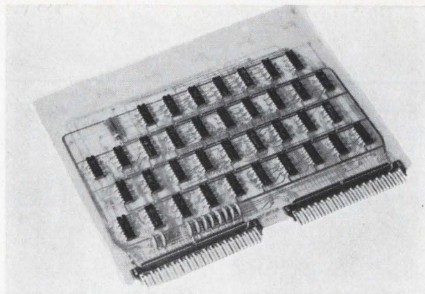
Five on one. Printed-circuit card contains functions for linearizing five transducers. Some portions of the circuits are shared, reducing cost per function.
