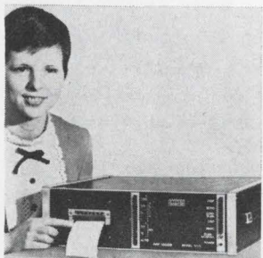
Multichannel data logger model DL-2 provides for automatic and precise measuring and recording. It is designed with a digital display and a printed record of up to 100 different electrical signals. Monitoring speed is normally one signal per second and intervals between scans can be adjusted up to 5 minutes duration. P/P/M Inc., 7016 Euclid Ave., Cleveland 44103. [425]
