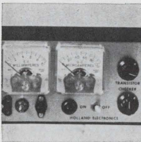
Transistor tester TT285 checks for npn or pnp configurations, shorts, opens and gain. It includes two 1 5/8 in. square ammeters, 0-100 \mu a base current and 0-10 ma collector current. A potentiometer, as part of a voltage divider circuit, applies current to the base connection. The unit measures 2 1/2 x 5 3/4 x 3 in. Holland Electronics 842 E. 94th St., Brooklyn. [361]
