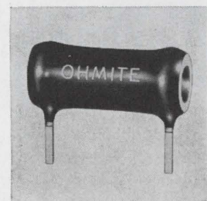
Radial-lead, power wirewound resistors designated PC-58 are available in 3-, 5-, and 8-watt sizes. By eliminating cutting, bending and forming leads, the PC-58 cuts labor costs up to 21.9% with productivity increases of 28.1%. Resistance range is 0.51 to 7,000 ohms. Price of the 3-w unit is 24 cents in lots of 500. Ohmite Mfg. Co., 3601 W. Howard St., Skokie, Ill. [342]
