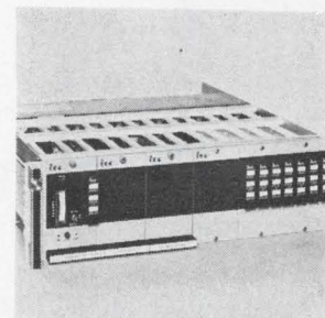
Tape data synchronizer 2755 provides coherent clocks for data processing systems where precise signal analysis or output display is required from unstable data containing record/reproduce errors. The unit tunes to all standard tape playback speeds over input reference frequencies from 3.125 to 400 khz. Interstate Electronics Corp., E. Vermont Ave., Anaheim, Calif. [428]
