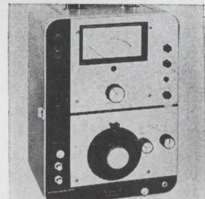
Standard deviation meter 140A is designed to accurately measure the peak frequency deviation of f-m communications transmitters. The output system includes a 750 \mu sec de-emphasis network which allows the unit to be used as a standard test receiver. The meter has direct reading ranges of 0 to 5 khz and 0 to 20 khz. Measurements, McGraw-Edison Co., Box 180, Boonton, N.J. [364]
