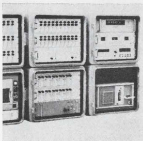
Multichannel transducer data acquisition system model SY-156(P) provides optimum portability. All system components are installed in rugged enclosures that serve as shipping containers by latching the covers in place. The system accepts inputs from strain gages, thermocouples, and can accommodate frequencies and a-c signals. B&F Instruments Inc., Cornwells Heights, Pa. [421]
