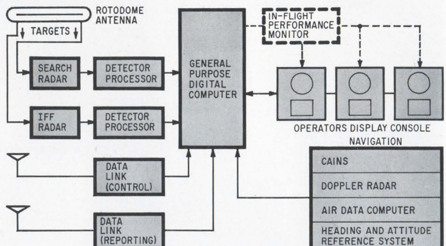
Nerve center. The E-2C's sophisticated avionics are designed around a large-capacity digital computer to be supplied by Litton Industries.
