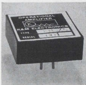
FET operational amplifier KM45 includes internal frequency compensation and short circuit protection. Features include a typical voltage offset drift of 10 \mu v/ ^{\circ} C, bias current of 10 pa, voltage gain of 10 6 , and input impedance of 10 12 ohms. Unit is for instrumentation, integrator and general purpose application. K&M Electronics Corp., 408 Paulding Ave., Northvale, N.J. [385]
