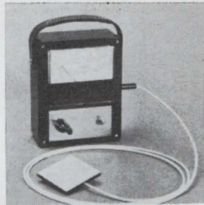
Thermal instrument model H-1 Heatprobe measures heat loss directly. It features 1/2% repeatability, accuracy of 2 1/2% and a maximum testing temperature of 275° F. No power supply is required. Three heat loss ranges provide direct reading between 0-50, 0-500 and 0-5,000 Btu/hr ft 2 . Basic price is $274.50. International Thermal Instrument Co., Del Mar, Calif. [362]
