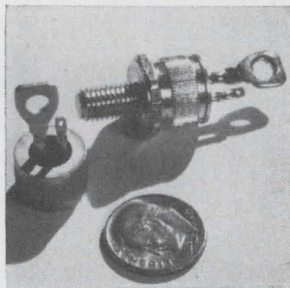
Twenty-five ampere triac thyristors SC60 (stud mounted) and SC61 (press fit package) offer a high surge current of 250 amps peak, high dv/dt and can handle up to 6 kw at 240 v. Voltage range is 200 to 500 v. D-c gate trigger current is rated at 50 ma maximum and d-c gate trigger voltage is 2.5 v maximum. General Electric Co., 1 River Road, Schenectady, N.Y. 12305 [440]
