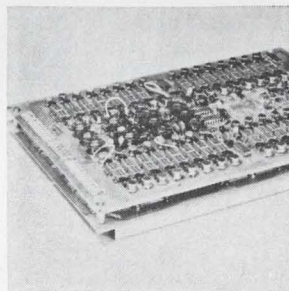
Core memory model 140 features 900 nsec full cycle time and 300 nsec access time. Modular design permits a wide range of word capacity/word size memory systems from this basic building block. Capacity of the module is 4,096 words x 8, 9, 10 bits. Unit measures 8 \frac{5}{8} x 17 \frac{5}{8} x 12 \frac{1}{2} in. and weighs 3.5 lbs. Micro Systems Inc., 644 E. Young St., Santa Ana, Calif. 92705. [423]
