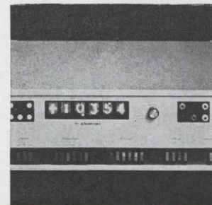
Digital multimeter 6653A is an all IC logic 4-digit instrument with fifth digit, 10% overrange. The basic unit measures d-c and d-c/d-c ratios with an accuracy of \pm 1 digit from 0 to 1099.9 v. The unit is standard 19-in. rack mount. Price of the basic unit is $1,740; delivery, 30 days. Lear Siegler Inc., Cimron Division, 1152 Morena Blvd., San Diego, Calif. 92110. [368]
