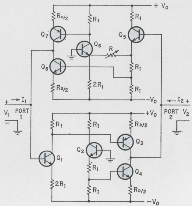
Voltage-current converter. A common-base stage, converter's collector current is proportional to base voltage. Output impedance at the common-collector terminal can be made as high as 6 megohms.
