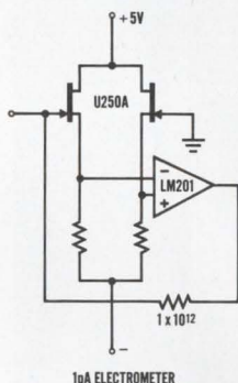
1pA ELECTROMETER
