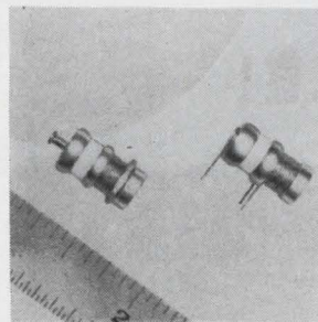
All-metal, air variable capacitors series MVM meet or exceed Mil-C-14409C. They are adjustable from 0.8 pf to 10 pf. The Q factor exceeds 2,000, measured at 10 pf and 100 Mhz. Insulation resistance at 25° C and 500 v d-c is 10 9 megohms, and temperature coefficient of capacitance is 0 \pm 20 ppm./° C. JFD Electronics Co., 15th Ave. at 62nd St., Brooklyn, N.Y. [348]
