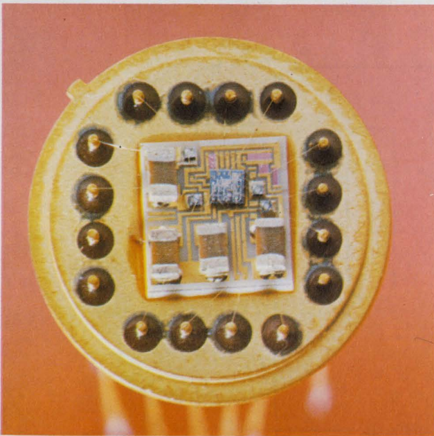
First . . . Chip and wire preamplifier with FET input is TI's first product in a new line of standard hybrid IC's.
