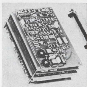
Four-microsecond random access memory system FI-2 is a 1024 word by 8 bit/word ferrite core assembly built on five interconnected circuit cards and designed to slide into a card cage or mounted remotely. Access time is 600 nsec. Power required is \pm 12 v at 3 amps. Size 8 \frac{3}{8} x 4 \frac{7}{8} x 3 \frac{3}{8} in. North American Philips Co., Ferroxcube Systems Div., Englewood, Colo. [422]
