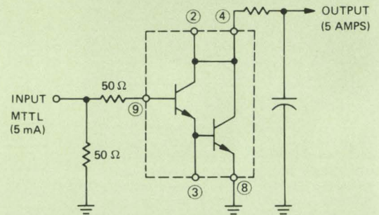
I/C Hybrid (Thin -Film) 5 Amp Darlington Driver
