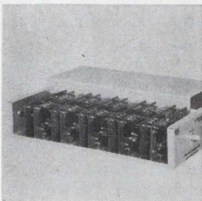
Logarithmic amplifiers series 200 convert 1-f/i-f signals to a d-c voltage that is directly proportional to the log of the input signal level. Units operate over a center frequency range of 100 to 250 khz with a bandwidth of 8 to 24 khz. They have a dynamic range of 80 db at a logarithmic accuracy of 2 db. Aerospace Research Inc., 130 Lincoln St., Brighton, Mass. [381]
