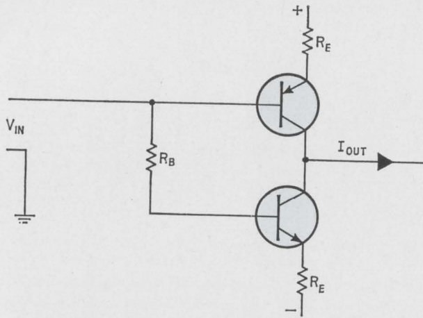
Voltage-current converter. A common-base stage, converter's collector current is proportional to base voltage. Output impedance at the common-collector terminal can be made as high as 6 megohms.
