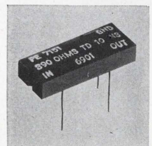
Distributed constant delay lines are designed to be compatible with dual in-line IC packaging. Standard units are available with 100 or 390 ohm impedances and delay times of 5 to 100 nsec. Distortion is 15% maximum; temperature coefficient, approximately 200 ppm/ ^{\circ} C. Prices are $2.05 in 1,000 lots. Pulse Engineering Inc., Robert Ave., Santa Clara, Calif. 95050 [388]
