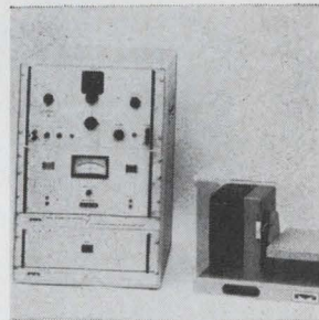
Single-axis portable flight motion simulator model 12A features less than 0.0025° threshold and 0.01° accuracy. It can statically and dynamically test gyros, accelerometers, flight control systems and guidance packages. The equipment can be driven by an analog computer, tape recorder or function generator. McFadden Electronics Co., 8953 Atlantic Blvd., South Gate, Calif. [363]
