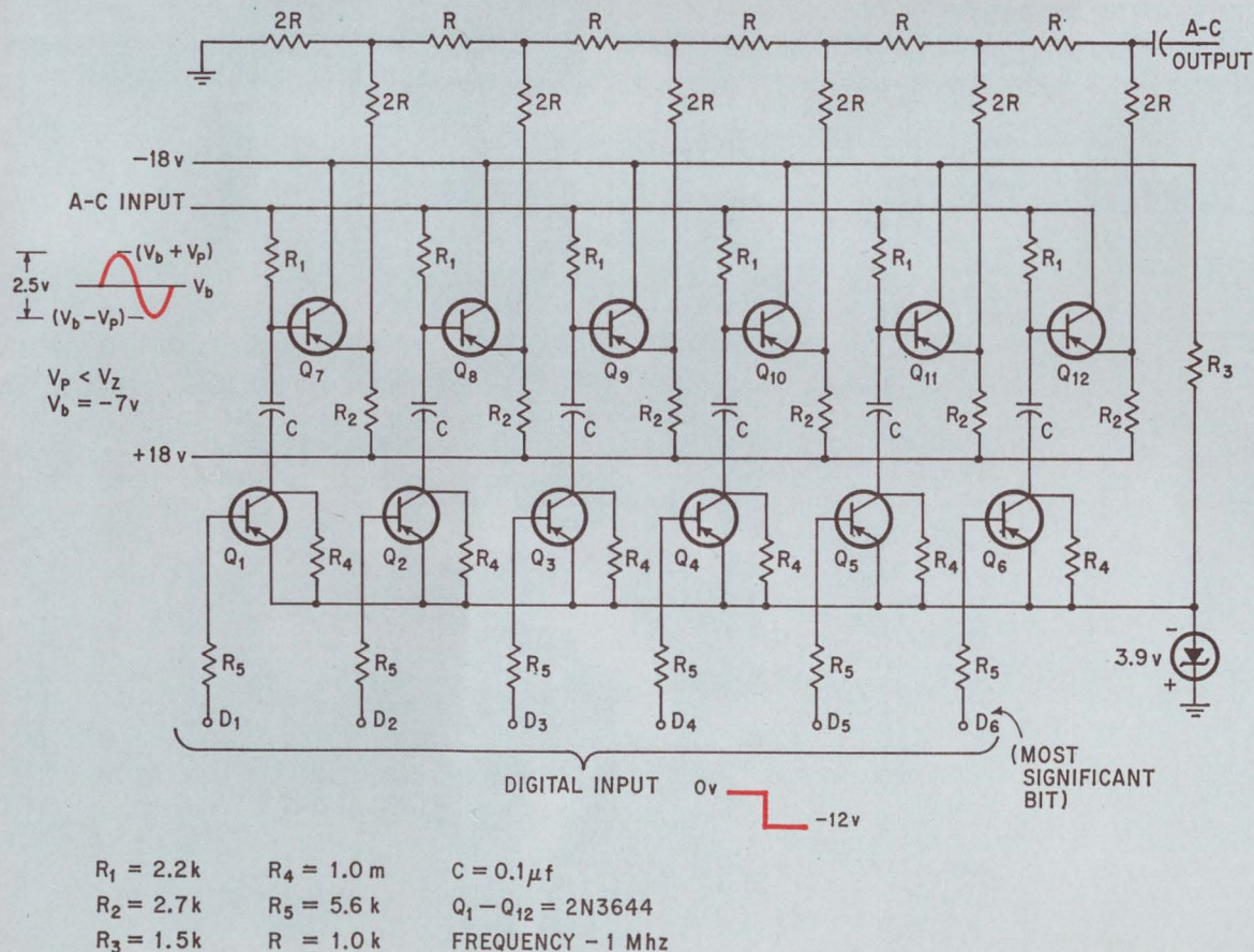
Ladder. Binary D_1 through D_6 saturate or cut off transistors Q_7 through Q_{12} whose bases are driven by an a-c signal. Those transistors that are saturated by the binary inputs, deliver the a-c signal to the output with a voltage weighted by a conventional resistive ladder network.
