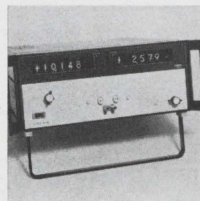
Automatic capacitance bridge C357 is a 1-khz unit with four-digit resolution, five-terminal connections, and an on-range measurement time of only 150 msec. It measures capacitance from 0.1 pf to 15.99 \mu f and dissipation factor from 0.00001 to 0.15999. Basic accuracy is \pm 0.1\% for capacitance, \pm 0.2\% for dissipation. Teradyne Inc., 183 Essex St., Boston, Mass. [367]
