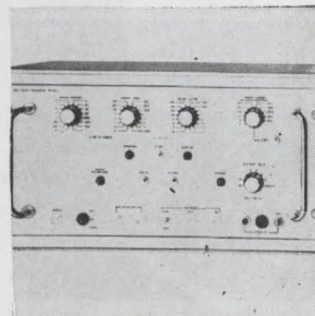
Signal averagers models 101/102 are used to pull out the signal-to-noise ratio of low level repetitive signals buried in a high background noise. Both can sample at intervals as fast as 2 \mu sec, yet handle slower sweeps with samples taken up to 100 msec apart. Aperture time is 20 nsec, with resolution to a 7-bit binary. Biomation, 1076 East Meadow Circle, Palo Alto, Calif. 94303 [366]
