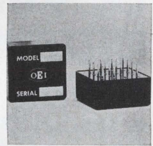
Sinusoidal function module model 5217A comes in a 0.5 cu in. package with a height of 0.5 in. It features \pm 1\% static accuracy, \pm 3\% dynamic error at 10 khz, and 100 khz useful bandwidth. Applications include trigonometric computers, sine and cosine generators, visual display rotation circuits, etc. Price is $43 each. Optical Electronics Inc., P.O. Box 11140, Tucson [384]
