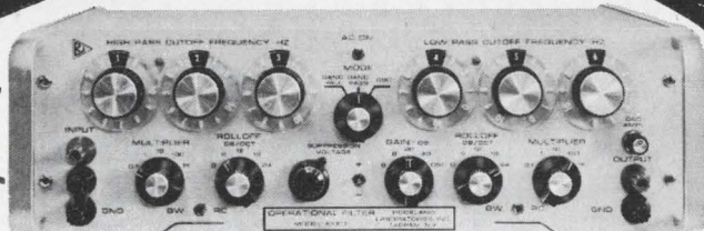
OPERATIONAL FILTER
