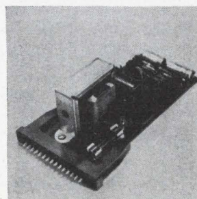
Dual power supply model 222A provides regulated \pm 15 v d-c at 50 ma. It also provides unregulated \pm 24 v d-c at 100 ma. The \pm 15 v units are for use with operational amplifiers and similar equipment. The \pm 24 v d-c output can be used to supply power output stages and as a source of unregulated relay drive voltage. California Electronic Mfg. Co., Alamo, Calif. 94507 [387]
