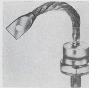
Silicon rectifier diode D0-8 has forward current capability up to 150 amps and prv ratings to 1,000 v. Freedom from thermal fatigue is achieved by use of a hard solder construction and matched thermal coefficients. The design utilizes the Solitron chip which features the hermetically sealed, glass passivated junction. Solitron Devices Inc., 256 Oak Tree Rd., Tappan, N.Y. [442]
