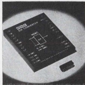
Modular d-a converters series HDAC are 8-12 bit devices that settle to 0.05% of full scale within 1 \mu sec maximum. Both output amplifier and reference are internal. The module measures 2.625 x 3.125 x 0.4 in. high and is intended for p-c board mounting. Price (1-9) starts at $200 each. Delivery takes 2 to 4 weeks. Data Device Corp., 100 Tec St., Hicksville, N.Y. 11801 [382]
