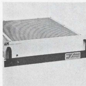
Video message generator series 44 is for communication and data systems. It converts alphanumeric data or messages in the form of standard teletypewriter codes to a visual display on a standard tv monitor or commercial tv set. Only 5 \frac{1}{4} inches of panel space is required and power consumption is less than 35 w. Data Technology Corp., 1050 East Meadow Circle, Palo Alto, Calif. [427]
