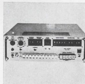
Self-contained data logging system DLS-500 will simultaneously accept and multiplex up to 20 analog and 5 digital inputs and provide outputs in IBM computer-compatible form capable of driving most incremental magnetic tape recorders. Each analog input is converted into digital data 11-bit plus sign. Applied Electro Mechanics Inc., 2350 Duke St., Alexandria, Va. 22314. [424]
