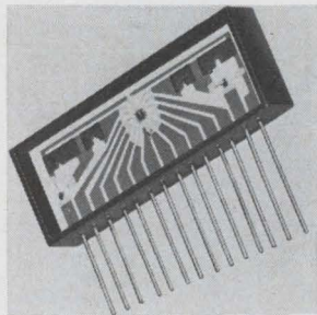
Dual power hybrid IC model MCH1002 is for interfacing high-threshold logic levels with electromechanical hardware. It features a maximum output current of 0.5 amp, a collector-emitter breakdown voltage of 40 v minimum a typical turn-on time of 115 nsec, and a typical turn-off time of 260 nsec. Motorola Semiconductor Products Inc., P.O. Box 20912, Phoenix 85036. [441]
