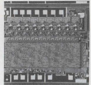
Random access, read only memory EA3000 is organized as 256 words, 9 bits per word (2304 total bits). Features include low power (90 mw typical at 1 Mhz), less than 1 \mu sec access time over a temperature range of -55^{\circ} to +85^{\circ} C, variable output buffer voltage and bipolar output drive capability. Electronic Arrays, Inc., 501 Ellis St., Mountain View, Calif. 94040 [439]
