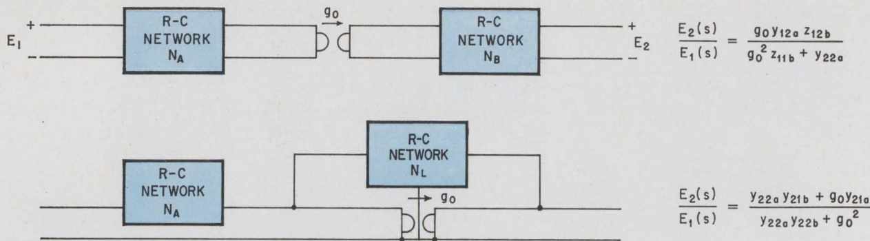
Variety. Several configurations are possible for coupling gyrators to R-C networks. Two possibilities are cascading with a gyrator in the center (top), and another is a parallel arrangement between the two R-C networks.
