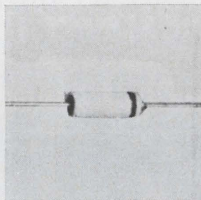
Varactors series SQ5461A, by maintaining a leakage spec of less than 4 na at the 30 v breakdown rating, can be conveniently tuned with high impedance voltage sources. The diodes are available in standard nominal capacitance values from 6.8 pf through 100 pf. Price (1-99) is $9 each; delivery, 2 weeks. MSI Electronics Inc., 34-32 57th St., Woodside, N.Y. 11377. [437]
