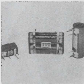
Miniature diaphragm relay JDYA features a moving contact that is a flexible diaphragm sealed in an inert atmosphere. It will interrupt up to 1 amp at 30 v d-c or a-c in either 1-, 2-, or 4-Form-A configuration. The 1-Form-A type is only 0.67 inch long. Units are available as standard coils of 6, 12, 24, or 47 v d-c. ITT Jennings, 970 McLaughlin Ave., San Jose, Calif. [341]
