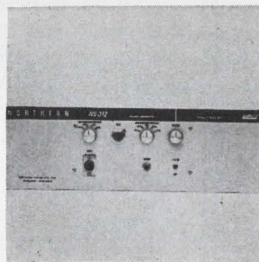
Low-level preamplifier type NS-312 is designed for biomedical applications where the signals are in the microvolt range. It has a maximum gain of 10,500. The low and high frequency cutoff are switch selectable. Common mode rejection is greater than 10,000:1 from 0.2 to 1 khz. Price is $495. Northern Scientific Inc., 2551 West Beltline, Middleton, Wis. 53562 [383]
