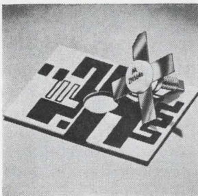
Balanced-emitter r-f power transistors 2N5644-2N5646 can provide 12 w in the 450-470 Mhz band with a 12.5-v power supply. They are for use as power amplifier stages of mobile transmitters in the uhf f-m band. Units come in the 3/8-in. ceramic stripline opposed-emitter package. Price (100-999) ranges from $8.30 to $22.50. Motorola Semiconductor Products Inc., Phoenix [436]
