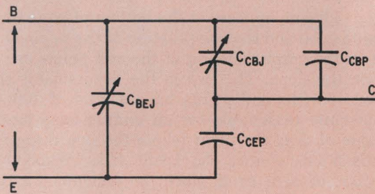
Base-emitter capacitance measured with collector-base not shorted.
