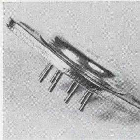
High-power d-c voltage regulator HCCA 100 features regulation of 0.05% maximum, 0.01% typical, no load to 1 amp load. The voltage range is 8 v to 50 v with maximum output current of 3 amps. Unit has 25 w dissipation at 25°C with heat sink and a temperature coefficient of less than 0.005%/°C. Solitron Devices Inc., 1177 Blue Heron Blvd., Riviera Beach, Fla. 33404 [438]
