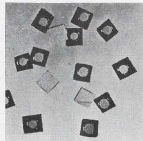
Silicon glass passivated mesa diode dice are available. Typical computer die sizes are 16.5 x 16.5 x 5 mil, with specifications at less than 2 pf capacitance and recoveries at less than 4 nsec. The dice meet or exceed MIL-S-19500 and MIL-STD-202 reliability specs without further treatment or encapsulation. Micro Semiconductor Corp., 11250 Playa Court, Culver City, Calif. [441]
