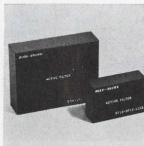
Low-pass active filters are designed for Butterworth response. Model 5720 is the 2-pole version at $25 each. Cutoff frequency range is 10 hz to 20 khz. Model 5721 is the 4-pole version with a frequency range of 1 hz to 20 khz and a price of $45. Both units have an output impedance of less than 20 ohms. Burr-Brown Research Corp., Int'l Airport Industrial Park, Tucson [386]
