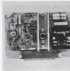
Programmable d-c voltage source model VS-510, designed for use as a system module, is packaged as a 4x6 in. p-c board assembly. Output voltage is 0 to 32 v d-c. Current rating is 100 ma. Line regulation is 0.005%; load regulation, 0.01%; and temperature coefficient, 0.01%/°C. Price is $103.50; delivery, from stock. North Hills Electronics Inc., Glen Cove, L.I., N.Y. 11542 [383]
