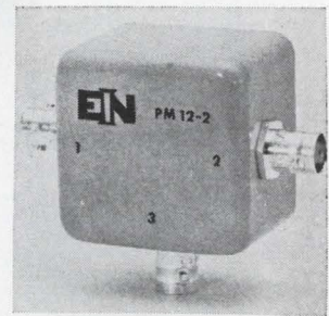
Power multicoupler model PM12-2 is a two-way hybrid coupler covering the range of 250 khz to 110 Mhz. Unit is capable of handling up to 12 w of average r-f power at +65°C ambient temperature. Maximum insertion loss is 0.4 db; amplitude balance, 0.1 db, phase balance, \pm 1^\circ ; vswr, 1.1:2 maximum. Electronic Navigation Industries Inc., 1337 Main St. East, Rochester, N.Y. [384]
