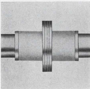
Back-to-back varactors DEP1712-1726 are for electronic tuning. They come with nominal capacitance values from 1.2 pf through 12 pf, with Q's of over 1500 measured at 50 Mhz. In the back-to-back configuration, one bias voltage supply, either a-c or d-c, is applied to the common flange contact with other contacts on ground. MSI Electronics Inc., 57th St., Woodside, N.Y. [440]
