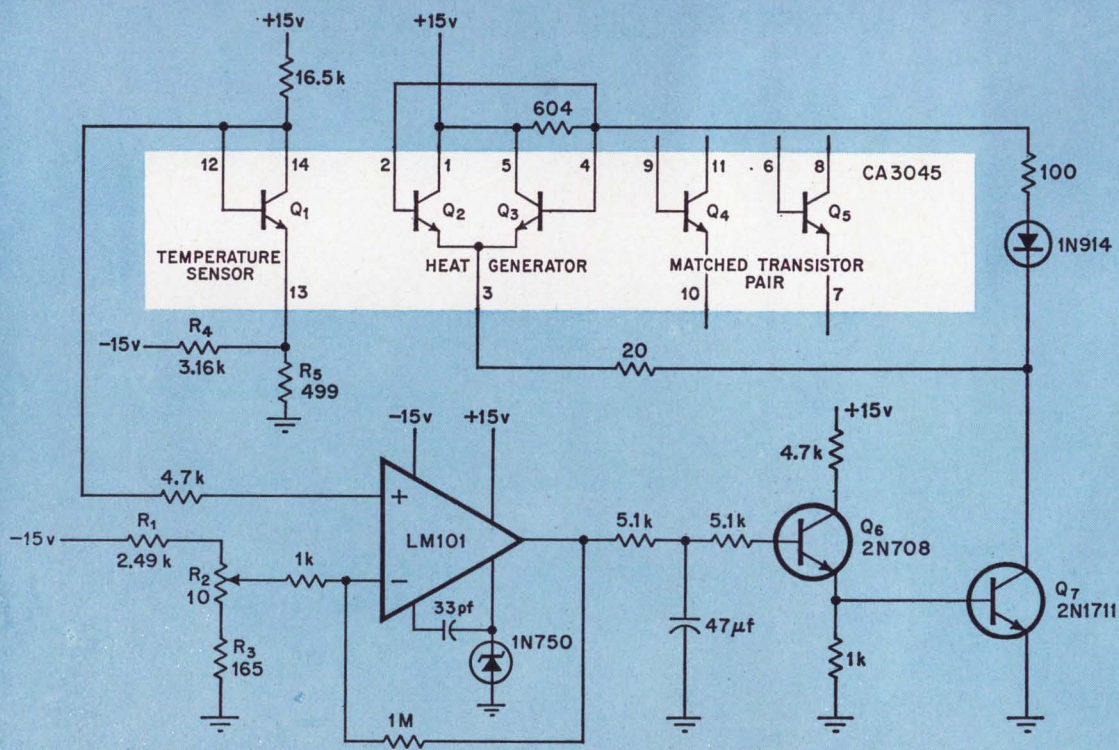
Good Match. Q_1 senses the substrate's temperature and delivers the corresponding voltage to one input of the op amp. The other input is set to the voltage equivalent of the desired temperature. This voltage difference drives the current regulator, Q_2 - Q_3 which heats the chip to hold its temperature constant.
