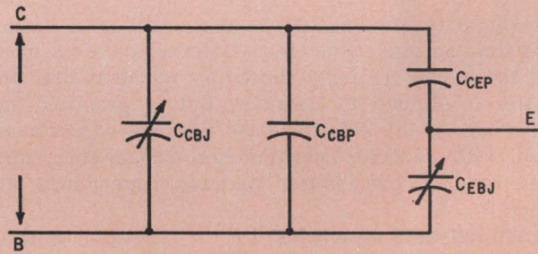
Collector-base capacitance measured with emitter-base not shorted.
