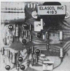
Dual output power supply model 2Q15-250PC operates from 105-125 v a-c, 60 to 400 hz, and furnishes \pm 15 v d-c with 250 ma capability from each side. Line and load regulation is held to 0.1% maximum with ripple and noise held to 2 mv rms max. Price (1-9) is $47 each. Delivery takes less than 2 weeks. Elasco-Eastern Inc., 5 Northwood Rd., Bloomfield, Conn. 06002 [385]
