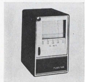
Voltage recorder model 2186 for high resolution line monitoring is an expanded scale recording voltmeter with low end of scales suppressed. Scales centered on nominal commercial line voltages have a resolution of 0.5 v per division on the basic range and 2 v per division in the 460 v a-c range. Rustrak Instrument Division of Gulton Industries Inc., Manchester, N.H. 02103 [368]
