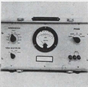
Output power meter model PM-2 is a passive device for determining the power output of audio-frequency generators, transducers, amplifiers and transmission lines while terminated with a known impedance. Power range is from 1 mw to 100 w. Impedance range is 2.5 to 20,000 ohms, and frequency range is 10 to 20,000 hz. Aul Instruments Inc., 139-30 34th Rd., Flushing, N.Y. [365]
