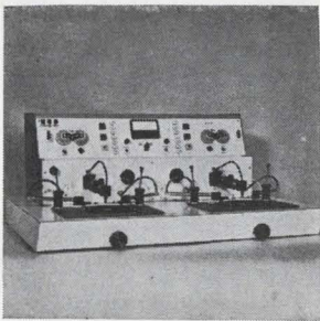
Dual resistor trimmer model DT-5 for use with thick film circuitry is a semiautomatic unit capable of trimming resistors to 0.1% accuracy from 10 ohms to 1 megohm. An X-axis adjustment of the work surface and Y-axis adjustment of the cutter nozzle enables the operator to accurately position the substrates. Modern Printing Methods Corp., 9 Harvey St., Cambridge, Mass. [421]
