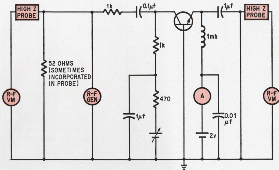
Measuring f_{hfbI} . Inverse alpha cutoff, f_{hfbI} , is obtained by providing a constant r-f signal at the collector and increasing its frequency until the output signal at the emitter drops by 3 db.
