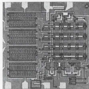
Eight-channel multiplex switch 3708 uses silicon gate technology. It offers channel switching of 0.4 μsec typically and interfaces directly with npn current sinking logic elements without the need of level shifting circuitry. The 3708 comes in a unit that multiplexes at -5 v to +5 v and in another that multiplexes at 0 to +5 v. Fairchild Semiconductor, Mtn. View, Calif. [442]
