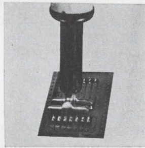
DIP soldering tip model 4918 is easily inserted in a standard 3/8-in. screw-type soldering gun of 35 w or more. Grooved and channeled for 10, 14, or 16 lead dual in-line packages, the tool will effectively desolder a complete 16-pin DIP in one pass. Unit also has end tips shaped for straightening bent connector pins. Techni-Tool Inc., 1216 Arch St., Philadelphia 19107 [422]
