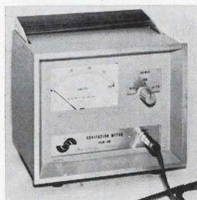
Cavitation meter model CVM-100 gives direct measurements for a broad range of research and testing applications in ultrasonics and many other technologies. It is the size of a small table radio and is simple to operate. Frequency is from 10 hz to 1 Mhz. Reading response time is under 2 sec. Price is $395. Macrosonics International Inc., 12 Calvin Rd., Watertown, Mass. [367]
