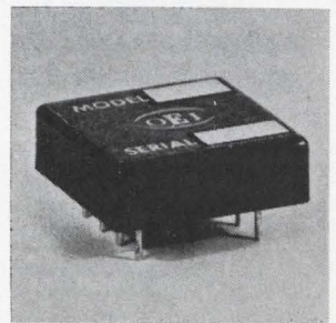
Hybrid operational amplifier model 9706 comes in an 8-lead jumbo dual in-line package measuring 0.32 in. high and 1 in. square. It features 60 db typical open loop voltage gain; \pm 360 v/ \mu sec typical slewing rate; 1,300 Mhz typical gain bandwidth product; and 10,000 megohm input impedance. Price (1-2) is $54 each. Optical Electronics Inc., P.O. Box 11140, Tucson 85706 [388]
