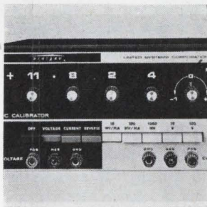
Precision calibrator model 311 offers 0.01% accuracy in both voltage and current. Five voltage and two current ranges are available. Current resolution is 1 \mu a and voltage resolution is 1 \mu v. Operational features include illuminated readout of setting, and pushbutton mode and range selection. Price is $650. United Systems Corp., 918 Woodley Rd., Dayton, Ohio 45403 [361]
