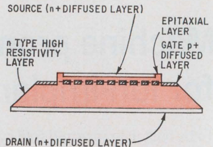
Pyramid. Thick intrinsic layer between gate, drain gives high power rating.
