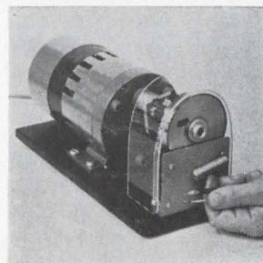
Motorized coaxial cable stripper model CX-2's operation consists of inserting the end of a co-ax cable into the rotating cable holder, and turning a handle which engages the 3 cutters to cut the insulation and shielding. Upon removal, end of cable is prepared with a 3-step strip for appropriate connector. Western Electronic Products Co., San Clemente, Calif. [427]
