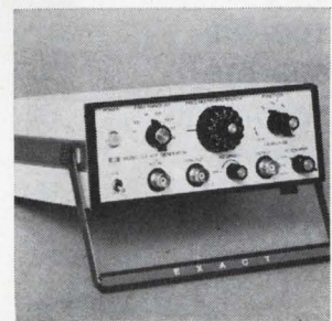
Miniature waveform generator model 123 features voltage controlled frequency over a 1,000:1 ratio and a bandwidth from 0.1 hz to 3 Mhz. It produces sine, square and triangle wave forms, as well as a sync pulse. Output voltage for all waveforms is at least 20 v p-p into an open circuit or 10 v p-p into a 50-ohm load. Price is $345. Exact Electronics Inc., Hillsboro, Ore. [364]
