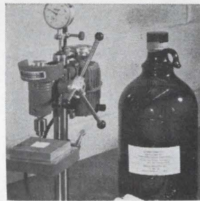
Accu-Drill 3300 kit includes all the equipment and materials necessary to drill holes from 0.025 in. diameter to 0.113 in. diameter in fired ceramic substrates used in IC's. Included in the kit are a sensitive drill press and a variable speed motor control necessary in controlling spindle speeds. Aremco Products Inc., P.O. Box 145, Briarcliff Manor, N.Y. 10510 [423]
