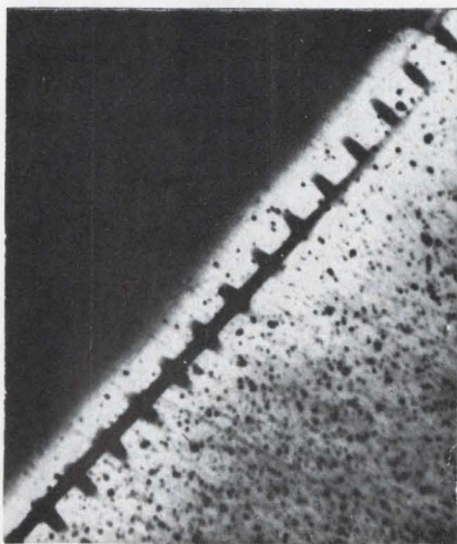
Cross section. Slightly angled slice through wafer shows gate's profile.
