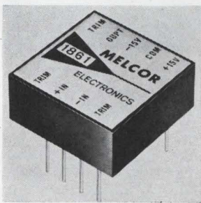
Amplifier model 1861 features a FET input stage combined with an IC. All shaping networks are internal, with no extras required except a zeroing potentiometer, if desired. Other features include an output of \pm 10 v \pm 5 ma minimum, minimum d-c gain of 15,000, and unity gain bandwidth of 1 Mhz. Price (1-24) is $10. Melcor Electronics Corp., Farmingdale, N.Y. [381]
