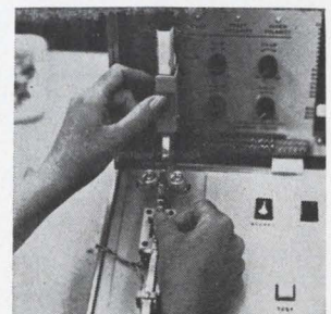
Semiautomatic DIP chip handling accessory permits operators of the model 997 IC tester to triple production test speeds achieved by manual methods for handling individual IC devices. Besides handling both 14- and 16-pin chips, the unit eliminates all extraneous sorting and handling time before and after testing. Beckman Instruments Inc., Richmond, Calif. [428]
