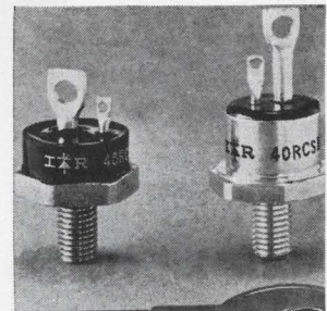
Silicon controlled rectifiers series 40RCS are new 40 amp devices available in two versions: epoxy package, up to and including 600 v rated units; and glass-to-metal sealed units rated from 700 v through 1200 v. Applications include d-c motor controls, power supplies, heater controls, and airborne and mobile converters. International Rectifier, 233 Kansas St., El Segundo, Calif. [439]
