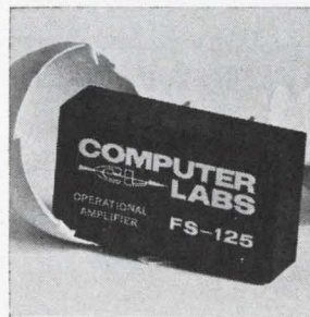
Operational amplifier model FS-125 is designed for fast settling on step function input signals. With a closed-loop gain of 1, the unit will settle to within 0.1% of full scale less than 80 nsec after the input is applied. It can be accurately calibrated with d-c. Price in small lots is $97; delivery, stock to 30 days. computer Labs, 1109 S. Chapman St., Greensboro, N.C. [387]
