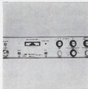
Frequency synchronizer/sampling detector LFS spans 50 khz to 4 Ghz. It may be used to phase-lock any oscillator exhibiting some degree of voltage tunability, or as a narrow band coherent receiver across its range. Sampling/lock spacing of 0.1, 1, 5 and 20 Mhz are selectable from the front panel of external 3 line logic inputs. Microwave/Systems, East Syracuse, N.Y. 13057 [362]
