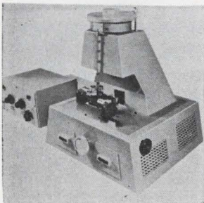
Automatic core handler model X-13 is used with a core tester to electrically test 14 to 30 mil outside-diameter ferrite memory cores at rates from 200 to 1,300 cores a minute. The handler transports the core to a test station where programed current generators determine the core's acceptability. Horex Electronics Inc., 1729-21st St., Santa Monica, Calif. 90404 [425]
