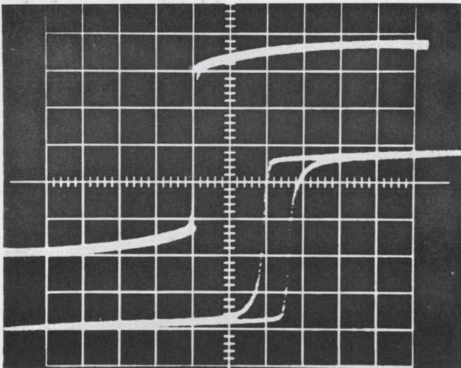
Enhanced. Top figure, hysteresis trace of bulk TT1-390 at a 400-oersted drive field shows a remanence ratio, M_r/M_s , of 0.67. The trace of the deposited film (bottom figure) made with same material has enhanced ratio of 0.82. Lower traces in each figure, expanded 500 times, show the deposited film with a squarer loop than the bulk material.
