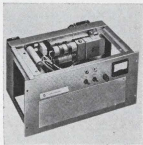
Uhf amplifier A80U is an 80-w unit for use with a fixed station transmitter to form a high power base station. It can also be used with uhf link and multiplex transmitters operating in the 440-470 Mhz frequency range. It requires a drive power of 5 w at 50 ohms impedance to provide a f-m r-f output of 80 w. Pye Communications Inc., U.S. Highway 46, Mountain Lakes, N.J. [382]
