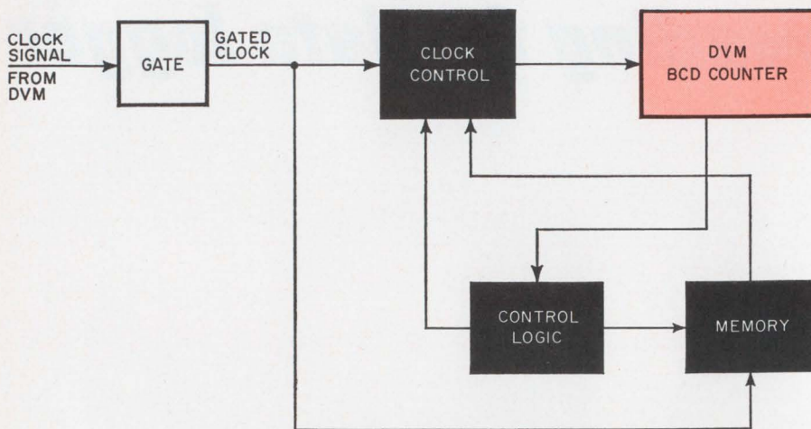
Three functions. Basic actions of digital reference-temperature simulator (dark boxes) coordinate with clock signals and functions (colored boxes) in digital voltmeter.
