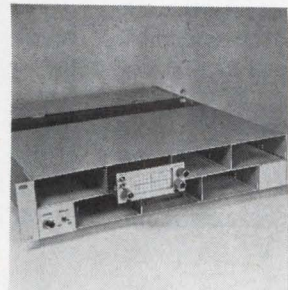
Up to seven series MS200 monitor oscilloscopes (10 Mhz bandwidth) can be plugged into a 3½ x 19 in. rack-mountable chassis for use in providing a continuous monitor of analog and digital signals. Input sensitivity is 0.1-10 v rms per in. Accuracy (vertical) is less than \pm 3% full scale. Sweep rate is 10 hz-1 Mhz. Vu-Data Corp., 7595 Convoy Court, San Diego, Calif. [366]
