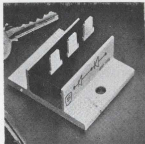
Silicon rectifiers series S6276 can be used singly as half-wave voltage doublers or paired to form full-wave bridge circuits. They are available in 8 piv ratings from 100 to 800 v. All units are rated for 50 amp continuous duty at case temperatures up to 60°C and will withstand surge currents up to 400 amps. Sarks Tarzian Inc., 415 N. College Ave., Bloomington, Ind. [437]
