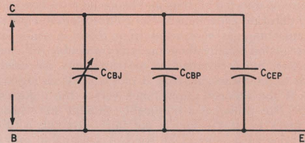
Collector-base capacitance measured with emitter-base shorted.
