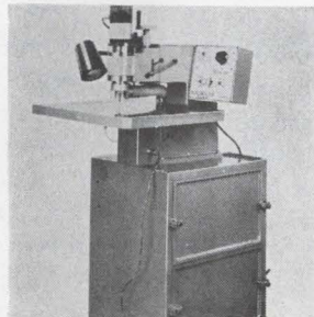
Precision pin router, the Acro-Router, for circuit board profiling and inside routing, features a constant torque spindle. Spindle speed is infinitely variable to 40,000 rpm max. Peak power is 0.6 h-p at 24,000 rpm. An integral dust collector sucks up chips and dust, keeps work and table surface clean. Aetna Mfg. Co., 245 Park Ave., Bensenville, Ill. [426]
