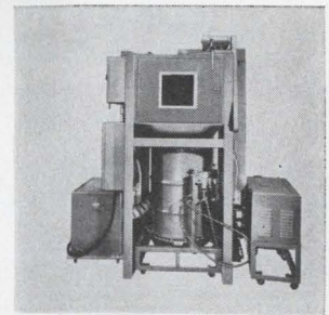
Varnish coater for electric motors and coils provides high reliability coatings, while cutting production time and material requirements in the process. The unit, which uses a powdered epoxy, imparts uniform, tack-free coatings in less than 7 minutes, and eliminates need for cleanup of the component prior to final assembly. Armstrong Products Co., Argonne Rd., Warsaw, Ind. [424]
