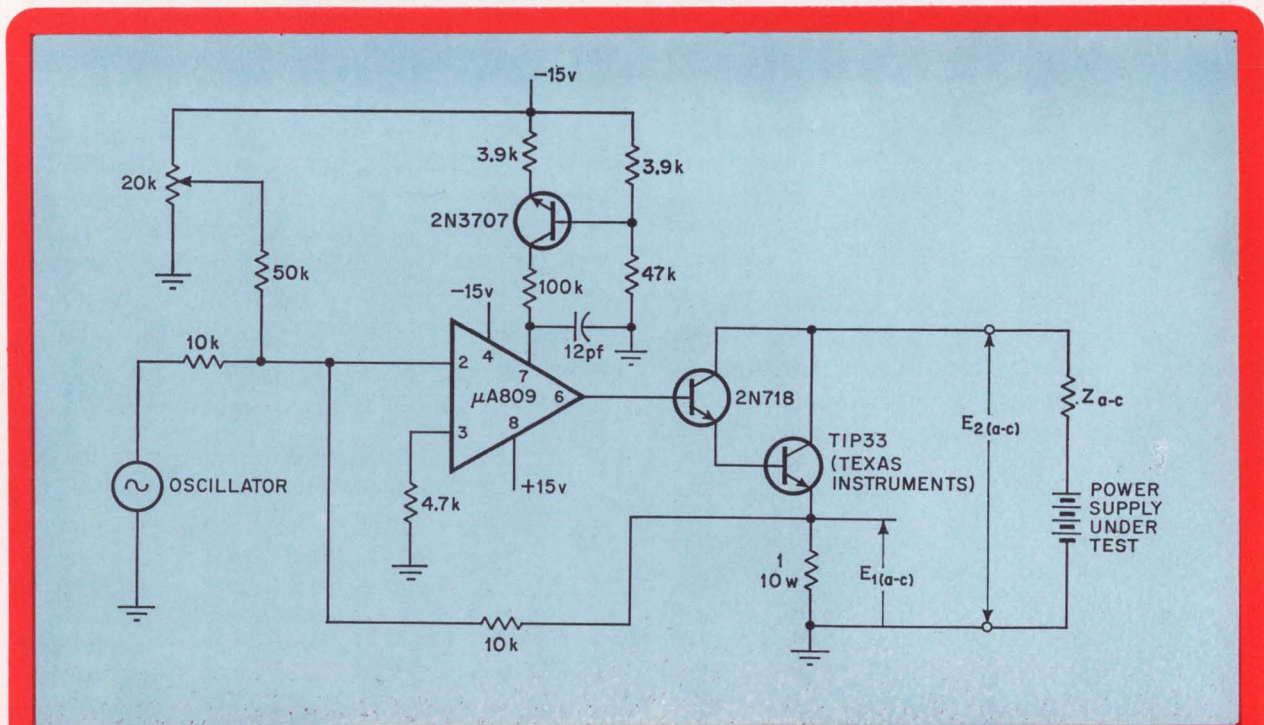
Impedance. An a-c component from the oscillator and a d-c component from the potentiometer are delivered to the input of the op amp. The power transistor forces an a-c voltage across the 1-ohm resistor from which the power supply's impedance, Z , can be readily determined from the relation Z = E_2/E_1 .
