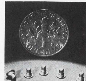
Snap varactor MA-43005 has low thermal resistance and high reliability in multisystem environments. It guarantees 0.25 w output at 10 Ghz. Typical breakdown voltage is 30 v; total capacitance is 0.65 pf minimum and effective minority carrier lifetime is 10 nsec. It is for circuits requiring high output power from 5 to 12Ghz. Microwave Associates Inc., Burlington, Mass. [443]
