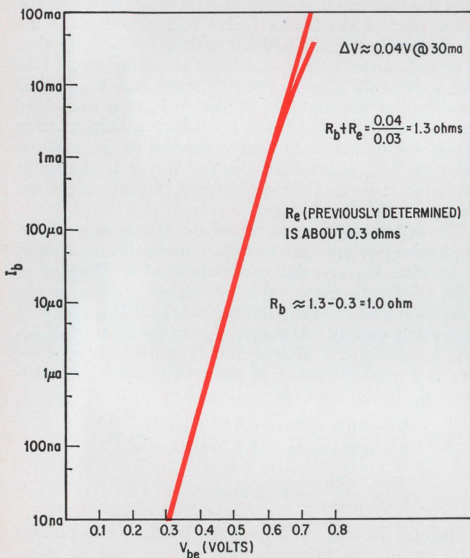
Resistance values. Resistors R_e and R_b can be evaluated graphically from a plot of I_b versus V_{be} .
