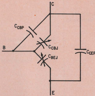
Typical transistor in can package
