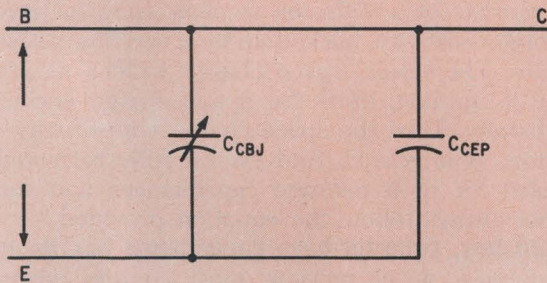
Base-emitter capacitance measured with collector-base shorted.
