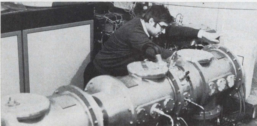
Plantation punch. Like an atom-smasher, Thomson-CSF's new machine accelerates particles for bombardment of a target, in this case semiconductor wafers. Simple controls allow in-plant use.
