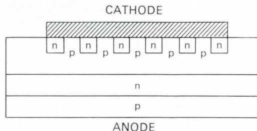
Fig. 2. AEI's Shorted Emitter Improved Thyristor
