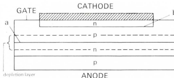
Fig. 1. Conventional Thyristor
