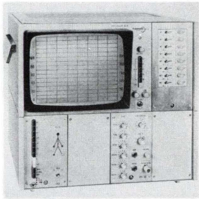
Phonocardiograph PH 53 comprises a heart noise sensor; a module (amplifier and filters) analyzing noise components in 6 preset bands; and a unit recording signals on photographic paper. Societe Thomson Medical Telco, 92 Saint Cloud, France. [219]
