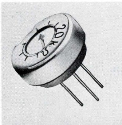
Wirewound potentiometer type 1113T has a range from 10 ohms to 50 kilohms and can take loads up to 0.75 watt at 70°C. The plastic-encapsulated device has \pm 10\% tolerance. Resista GmbH, 83 Landshut, Ludmillastr. 23, West Germany. [211]
