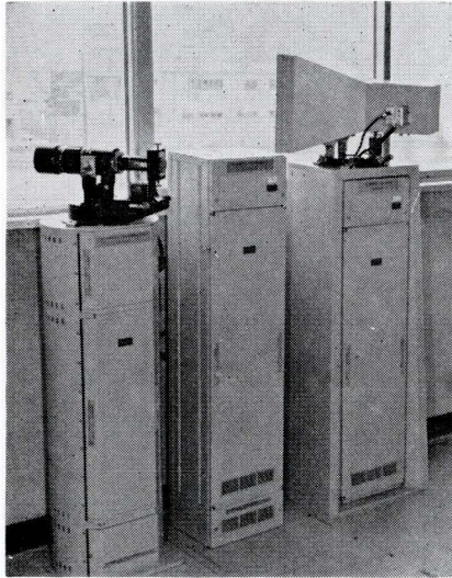
Short hop. Laser spans 3 kilometers to reach receiver, like one at right.
