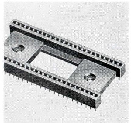
IC socket A23/2027 is a 50-lead dual in-line unit. The body is injection molded from glass-filled nylon type A190 and is available with a choice of contact material. Jermyn Industries, Vestry Estate, Sevenoaks, Kent., England. [212]
