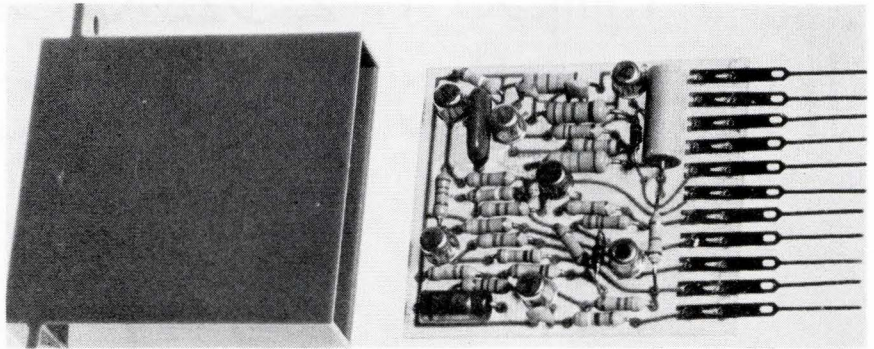
Drive circuit. As part of its work to keep deflection circuit power in 110° tubes down to 200° C, Philips used a switched-mode power supply.
