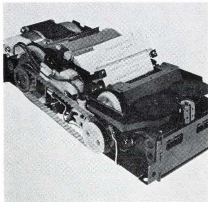
Mechanical printer P-12 is designed for electronic desk calculators. It prints up to 13 columns, one of which is decimal point, and one symbol on each line. Speed is 3 lines per second. Citizen Business Machines Co., Shinjuku-ku, Tokyo. [221]
