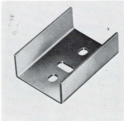
Heat sink A/25/2024 is manufactured from black anodized aluminum type NS4 quarter hard, with hole stamping compatible with both TO66 and SO55 device configurations. Jermyrn Industries, Vestry Estate, Sevenoaks, Kent., England. [220]
