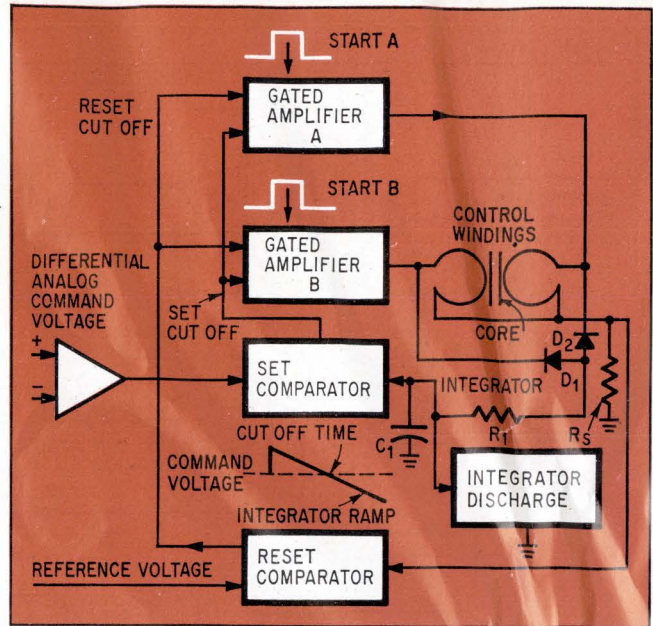
4. Dual roles. Control windings A and B alternately serve as magnetizing and sensing windings. The integrator monitors flux buildup for the comparator.
