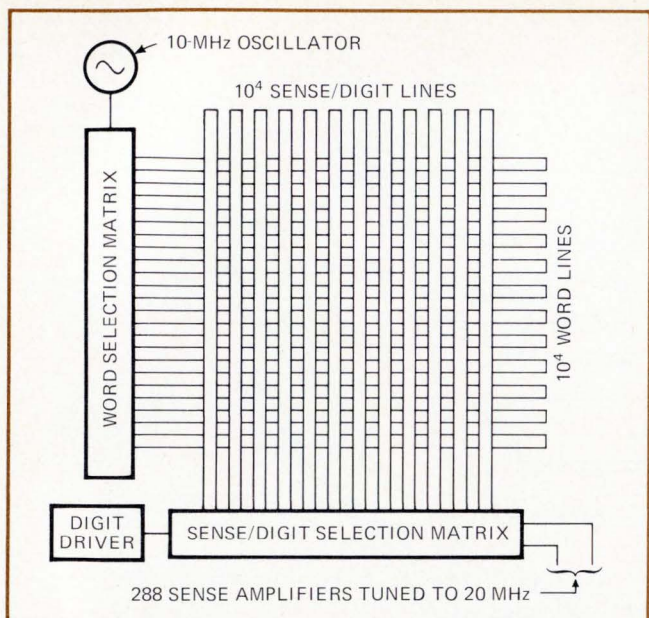
3. Memory layout. This oligatomic film layout holds 10^8 bits in a square format, with selection matrixes on two adjacent edges. Such a format minimizes electronic-circuit cost. Sense gates permit the number of sense amplifiers to be much less than the number of sense lines; but the 288 indicated are enough to move an eight-word block from the film to a cache memory in one 3-microsecond cycle.
