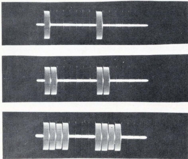
5. Sense line outputs. Scope traces show a sequence of one, two, and four 1s followed by 0s (sweep time is about 20 microseconds).
