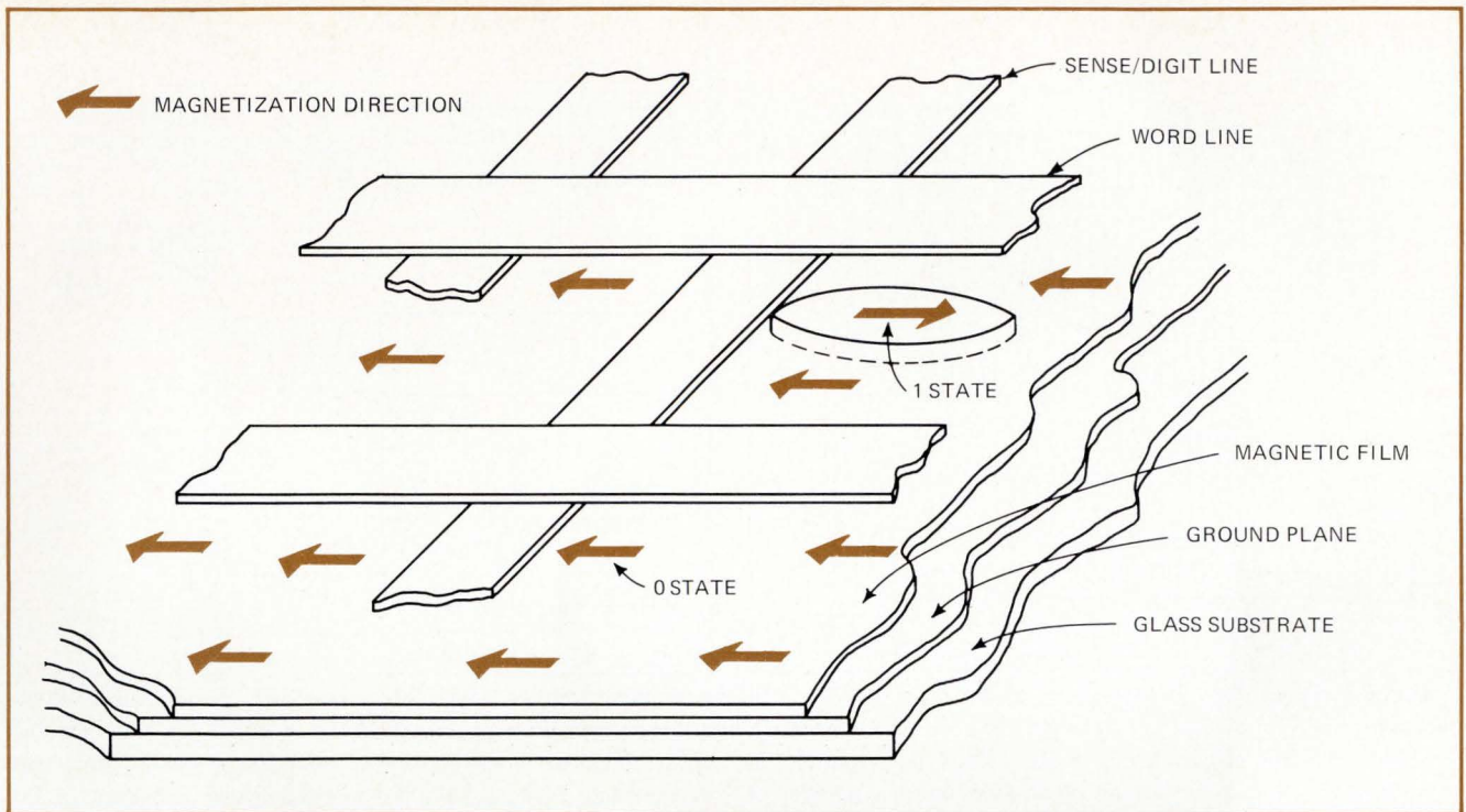
2. Thin film storage element. Colored arrows show normal magnetization along film's easy axis storing binary 0s. The one reversed arrow designates an area that has been switched, and therefore stores a 1. Word current rotates magnetization perpendicular to easy axis.
