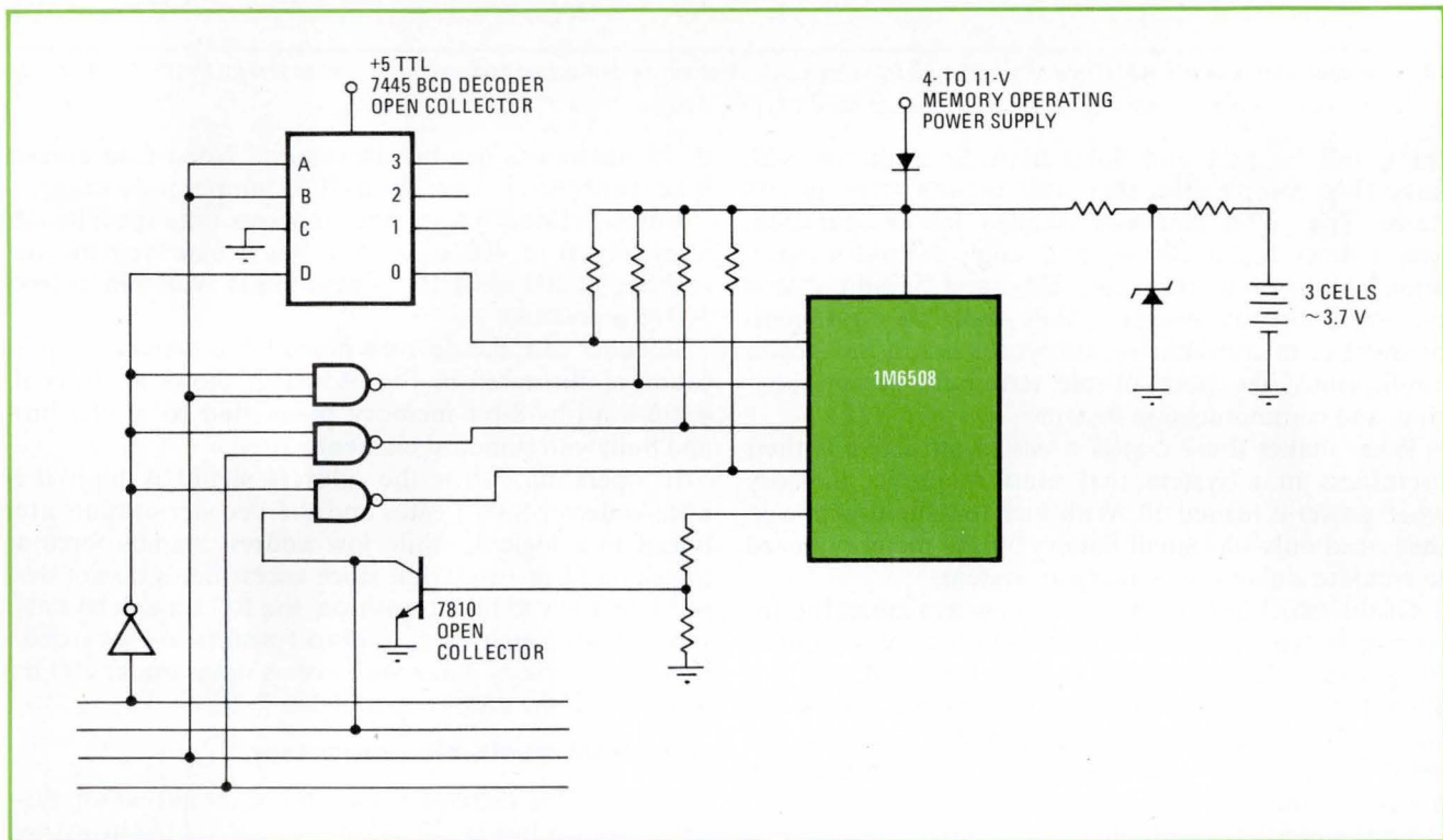
9. No forgetting. This C-MOS RAM system, built around Intersil's 1M6508 1,024-bit RAM, is a good approximation to a nonvolatile memory—it needs only a small battery to retain its data when system power goes off. The system, tied to a TTL bus, uses only off-the-shelf parts.
