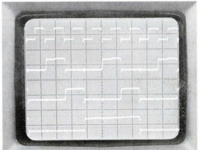
4. Time domain. The time-domain representation of a counter output yields more information about circuit operation than the equivalent data-domain pattern, but is more difficult to interpret if only logic-state information is required.
