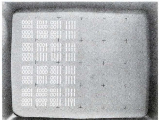
5. Arranging the sequence. To make a data-sequence table easier to read, a logic-state analyzer should display the information with the most significant bit on the left and the first word at the top.
