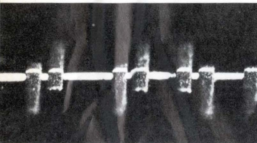
Beam leads on integrated circuits. Height and cross-section are measured.
