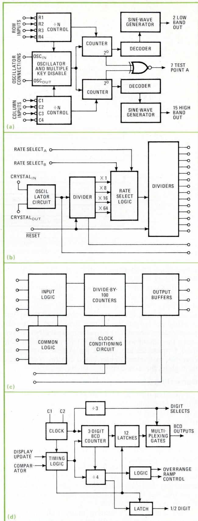
5. Better communication. Motorola puts complex functions on single chips. Tone generator (a) is for touch-tone dialing; bit-rate generator (b) provides wide range of frequencies, timer-driver (c) and converter logic (d) are aimed at printers and displays.
