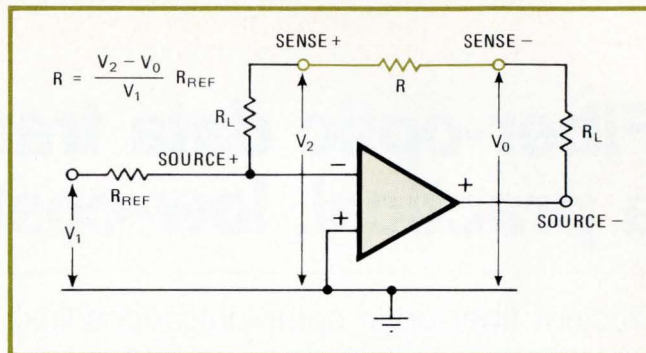
5. Resistance check. The availability of a microprocessor within a multimeter makes possible new measurement techniques. Here, three voltages are checked and the resistance calculated, eliminating variations in reference voltage as a source of error.
