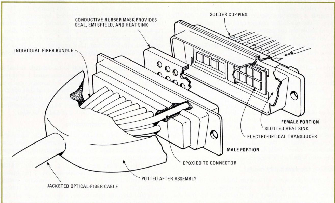
2. High-density packaging. All sources and photodetectors are mounted side by side, along with the electronic interface circuits, on a common substrate in the female half of the connector. The male half of the connector terminates the fiber-optic cable.
