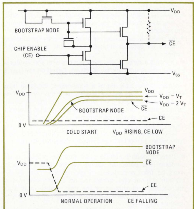
1. Startup. This precharge clock generator requires at least one cycle to charge the bootstrap capacitor (the MOS transistor with drain and source shorted) before the output reaches V_{DD} . The resistor shown dashed is sometimes used to help raise the output.
