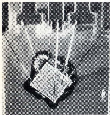
The TDA 2002 chip on its Pentawatt® frame.
