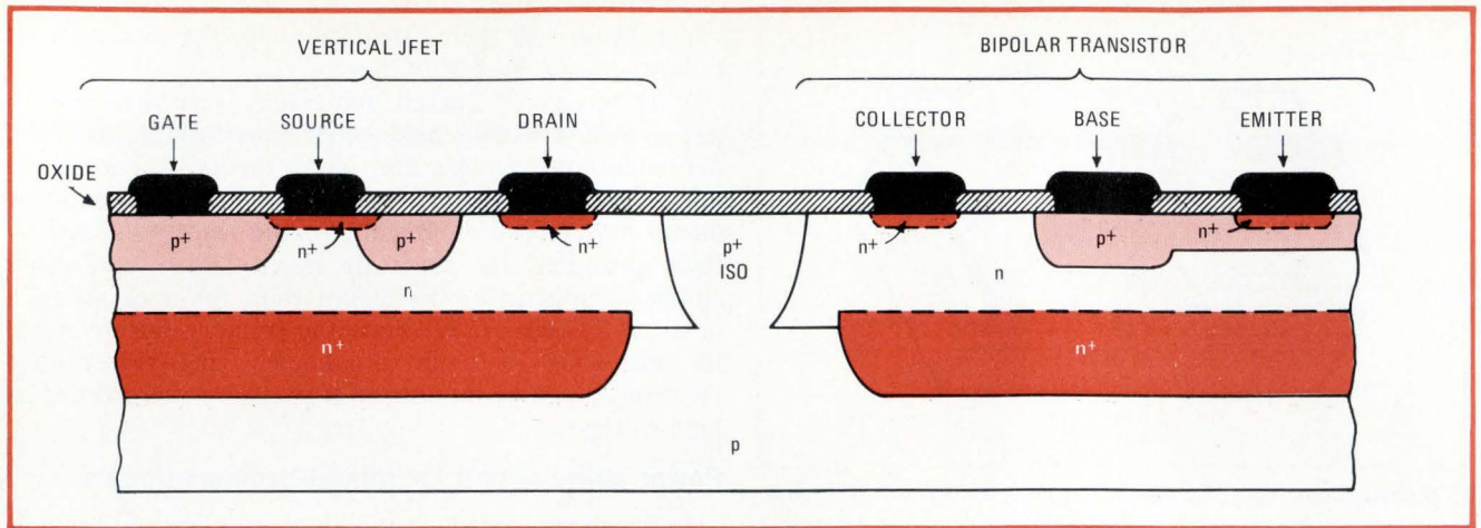
3. Mixed devices. With basically bipolar process, Hewlett-Packard has fabricated vertical JFETs on the same chip as bipolar transistors—with no additional processing steps. The vertical JFETs promise higher frequency and power capabilities for mixed-process linears.
