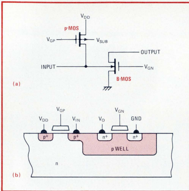
1. Now for B-MOS. A logic called back-gate-input MOS or B-MOS from Hitachi achieves low power and small size by using a back-gate driver to modulate a p-MOS current source (a). The B-MOS p well fits into the n substrate, taking up no extra space (b).
