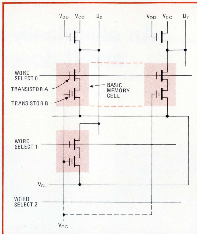
2. Basic cell. The memory cell contains two transistors—A, for selection, and B, for bit storage. Transistor B is shown schematically with a second, floating gate, which performs the basic storage operation. Eight memory cells are connected along one word line.
