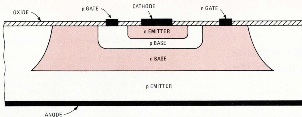
5. Temperature-sensitive. New four-layer thyristor-like switching device from Mitsubishi Electric Corp. turns on at predetermined temperature anywhere in the range of 50°C to 150°C. Triggering temperature depends on the value selected for the gate shunt resistance.
