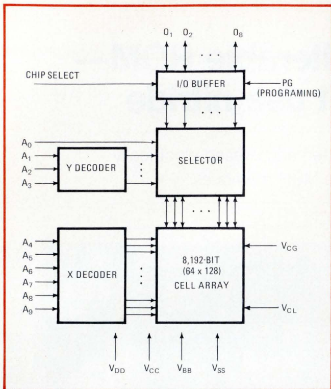
1. In the blocks. The electrically erasible PROM comprises an 8,192-bit array of memory cells, organized as 1,024 8-bit words plus decoders and buffers. In programming, all bits are initially turned off from the V_{CL} terminal and then selected bits are turned on from PG.
