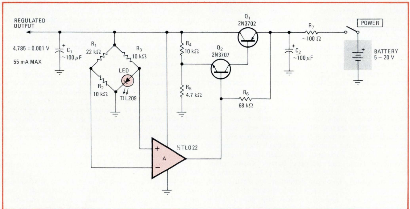
Battery supply regulator. Voltage drop across LED in bridge references op amp, controlling transistors in feedback loop. Under 5-milliampere load current, regulated output of 4.785 \pm .0005 V is achieved with supply voltages ranging from 4.835 to 20.00 V. With a 9.000-V supply, the regulated output is 4.785 \pm .001 V with loads ranging from 5 to 55 mA. Current through LED is barely enough to make it glow.
