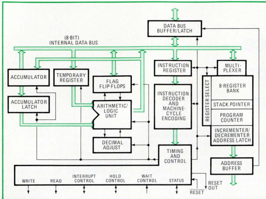
Meet the chip. The new 8085 microprocessor, which incorporates all the features of the older 8080 plus the clock generator and system controller, also has a multiplexed data bus. Addresses are split between the 8-bit address and the 8-bit data buses.
