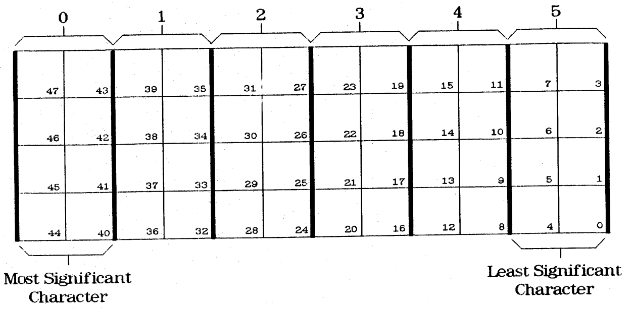
Figure B-2. EBCDIC Characters (8-Bit Fields)
