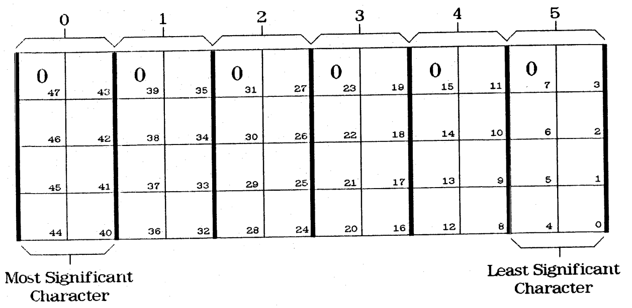
Figure B-3. ASCII Characters (8-Bit Fields)
