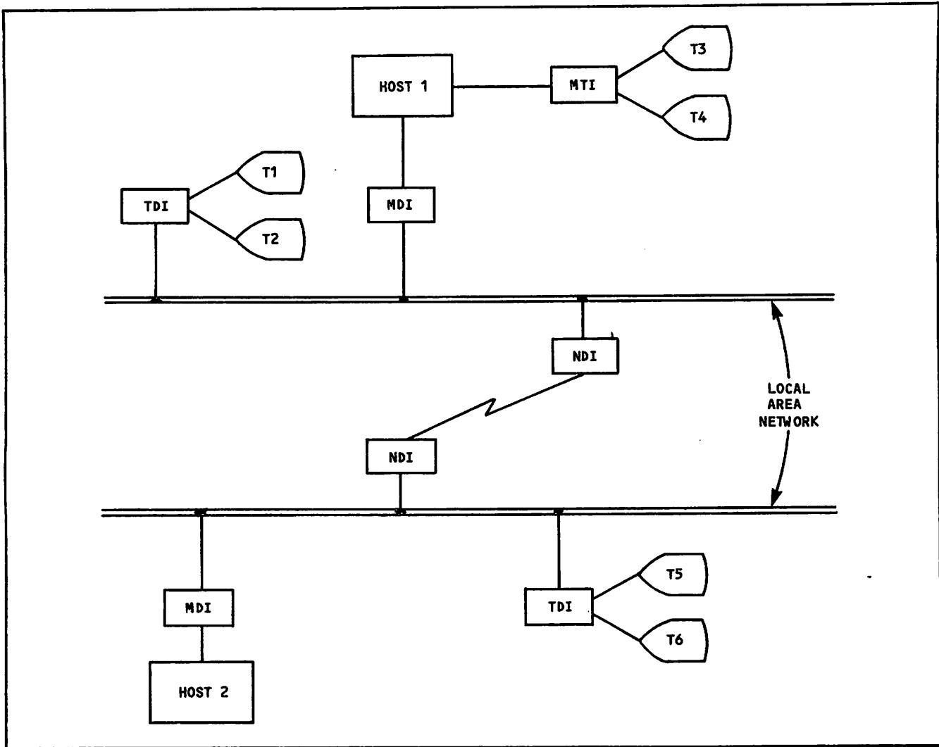
Figure 1-15 CDCNET Networks
