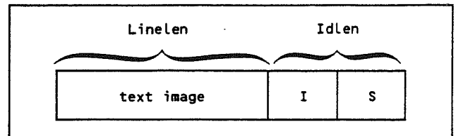
Figure 3-35. Fields of Line Image and Identification
