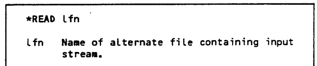
Figure 3-36. READ Directive Format
