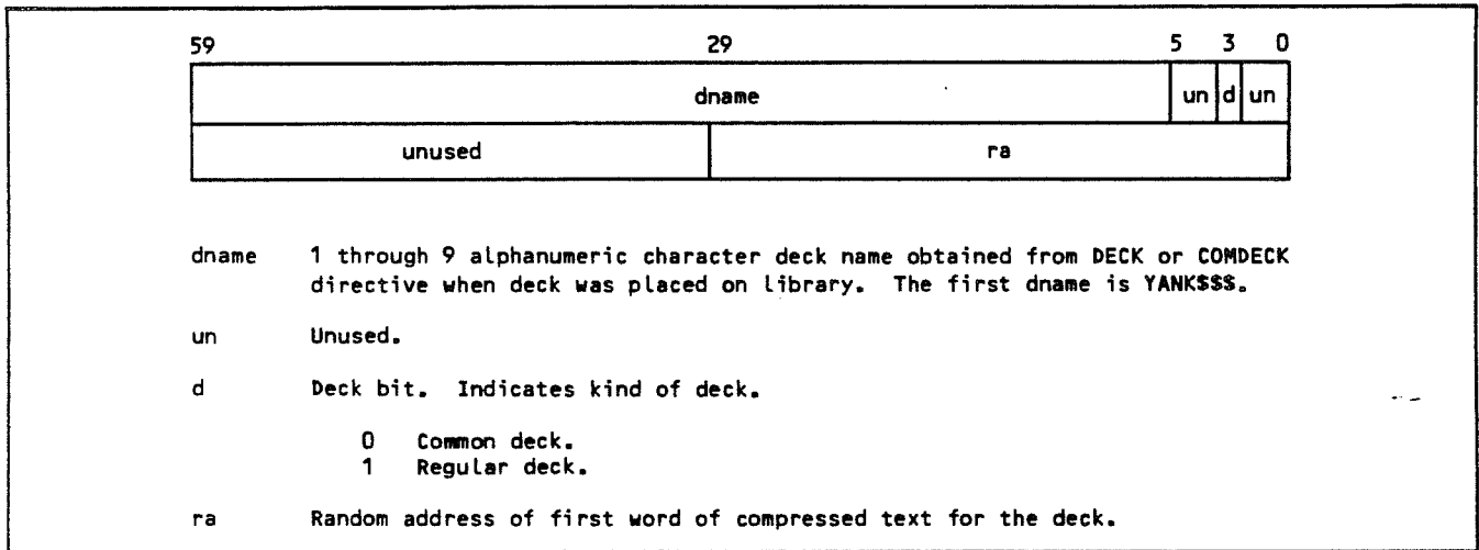
Figure D-8. Random Program Library Deck List Format
