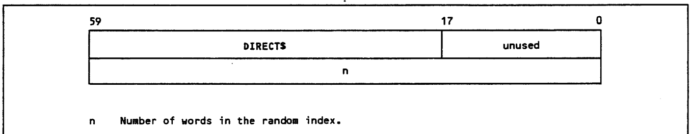
Figure D-3. SCOPE 2 Random Index Header Format
