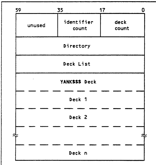
Figure D-11. Old Sequential Program Library Format
