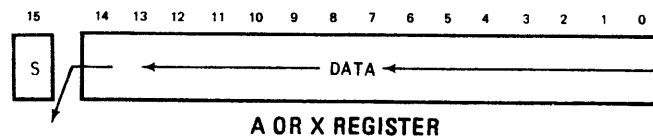
Figure 3-19. Arithmetic Left Shift
