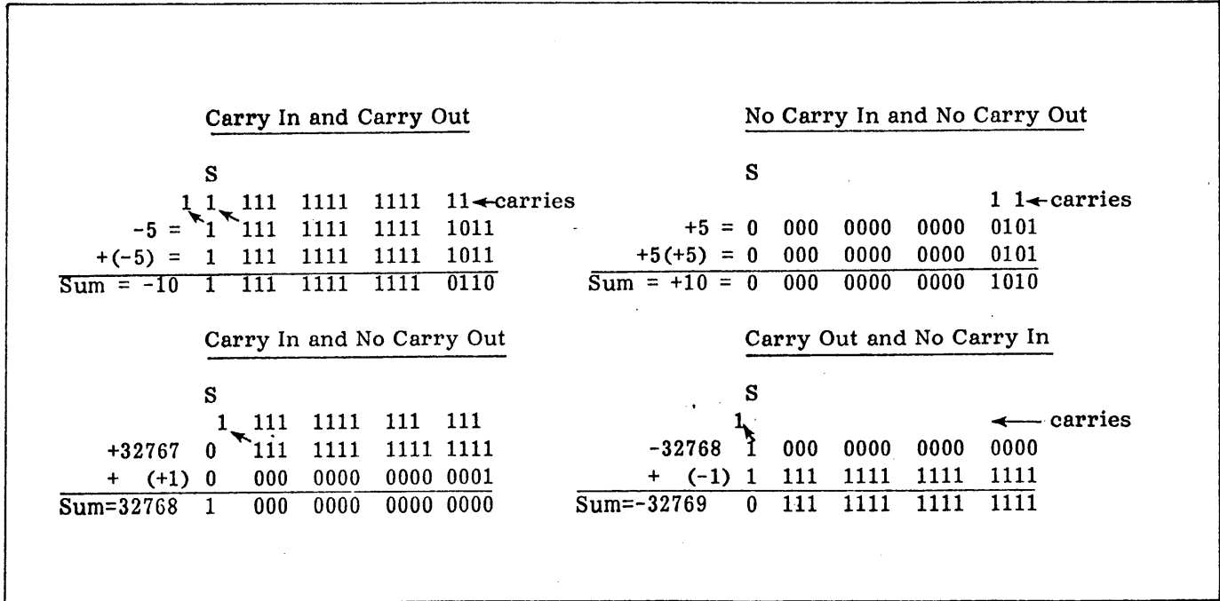
Figure 3-3. Arithmetic Overflow.
