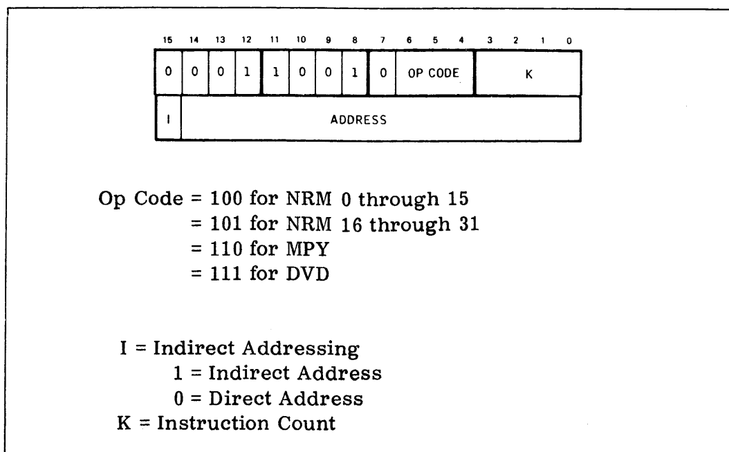
Figure E-2. Double-Word Memory Reference Instruction Machine Code Format
