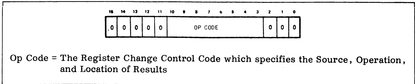
Figure E-7. Register Change Instruction Machine Code Format
