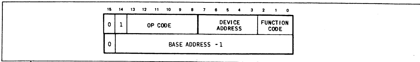
Figure E-11. Block Input/Output Instruction Machine Code Format
