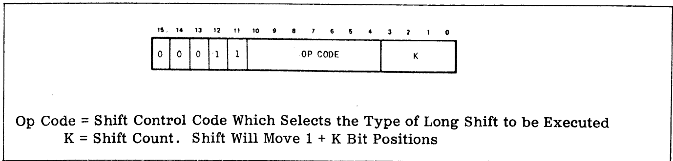
Figure E-6. Double-Register Shift Instruction Machine Code Format
