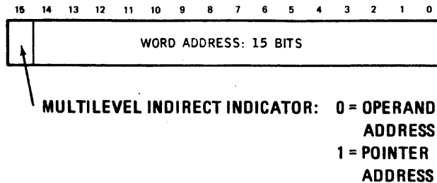
Figure 1-7. Indirect Address Pointer Format
