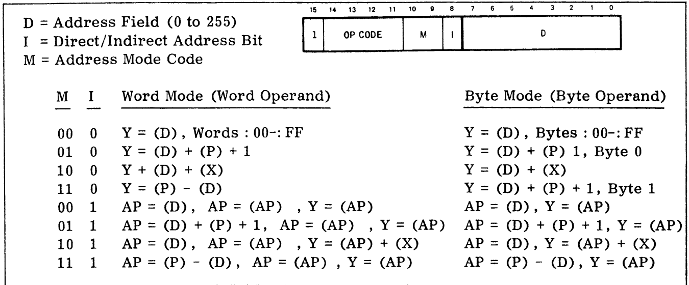
Figure E-1. Single-Word Memory Reference Instruction Machine Code Format
