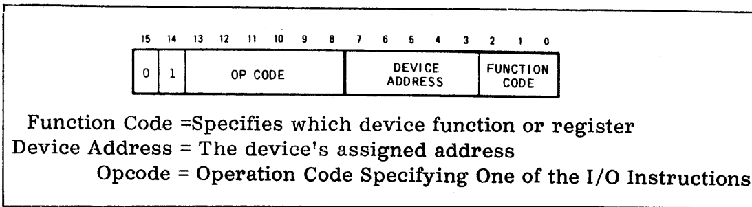
Figure E-9. Input/Output Instruction Machine Code Format
