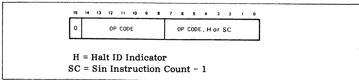
Figure E-8. Control Instruction Machine Code Format
