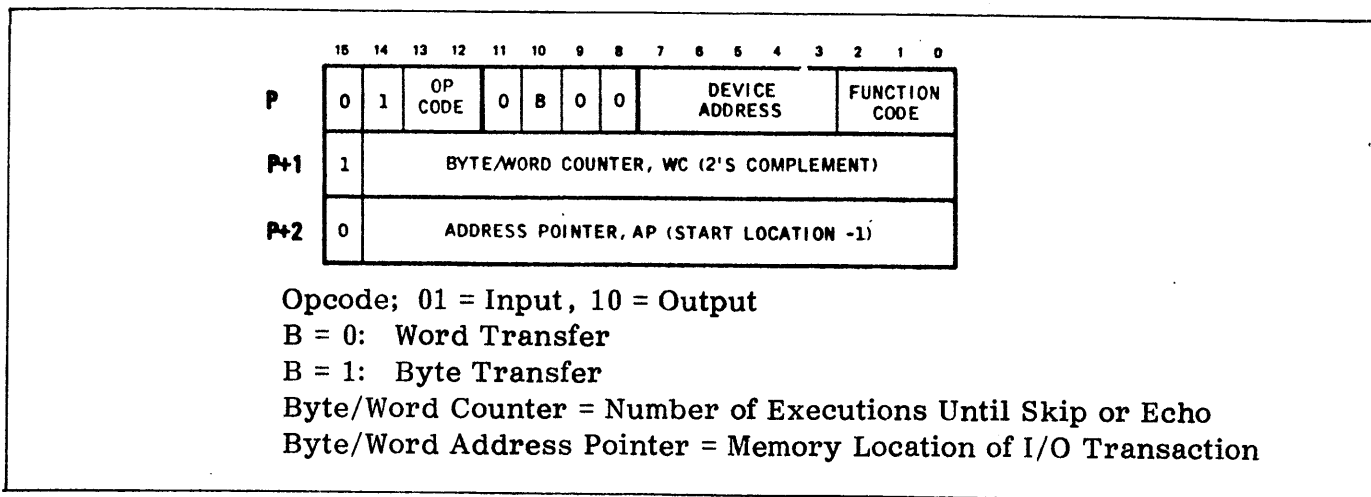
Figure E-10. Automatic Input/Output Instruction Machine Code Format
