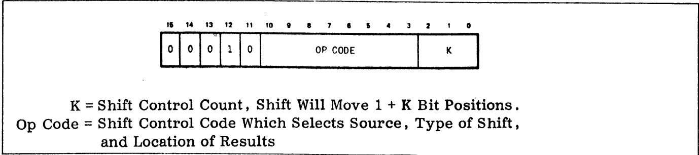
Figure E-5. Single-Register Shift Instruction Machine Code Format
