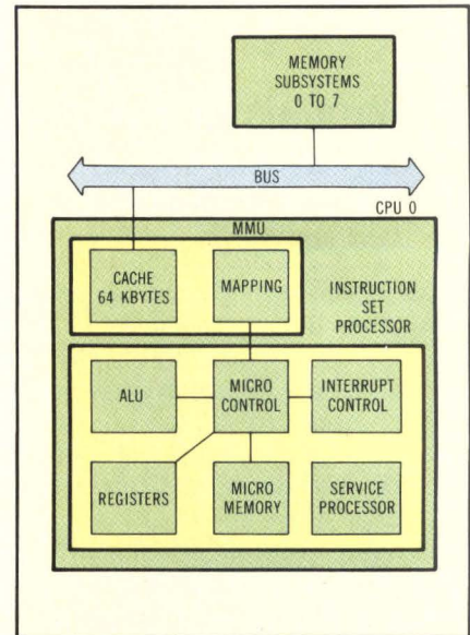
The CPU in Modcomp's 32/85 executes two instruction sets; one compatible with the 16-bit Classic II/75, the other providing 32-bit addressability. The instruction set processor is a complete ALU consisting of a functional microprogrammable processor with hardware multiply and floating point arithmetic. Microinstructions are contained in a writable control store.
