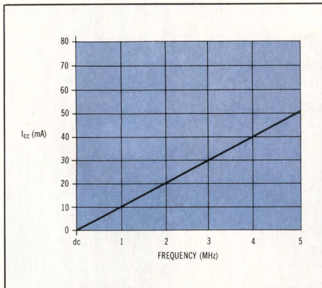
Fig 5 Power supply current of the 80C86 (and other CMOS micros) is linearly related to the operating frequency.
