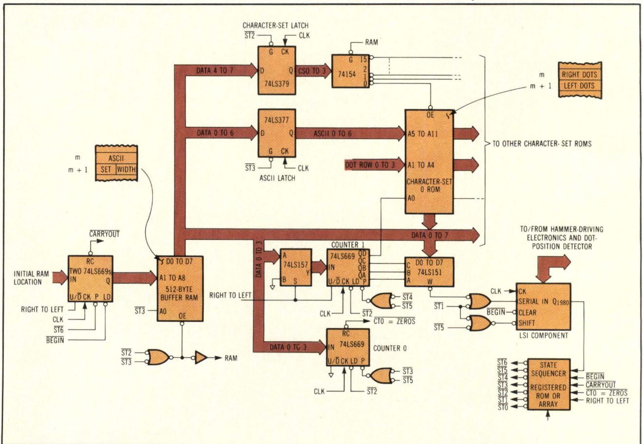
Fig 5 A simplified DGL schematic excludes circuitry needed by the control microprocessor to load the buffer RAM and other support circuitry. However, implementing a full-featured DGL for an impact line printer may require only a handful of common TTL devices.
