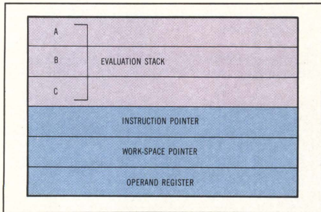
Fig 4 The register set consists of a small set of function specific registers to minimize process swap time and simplify compiler design.
