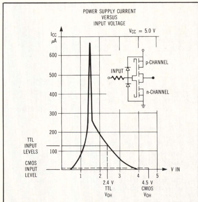
Fig 6 CMOS input circuit transfer characteristics show the danger of allowing the input voltage to float within the active region of the device. The floating inputs will settle at the threshold voltage where current flow is greatest. Consequently, unused inputs must be tied to either V_{CC} or ground.
