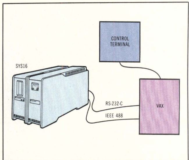
Fig 3 Developed on a VAX host, the Genix operating system is downline-loaded onto the NS16032-based SYS16 system. It accomplishes remote debugging by communication from a control terminal via the VAX and an RS-232-C line to a ROM monitor in the SYS16. The IEEE 488 bus provides fast file transfer.
