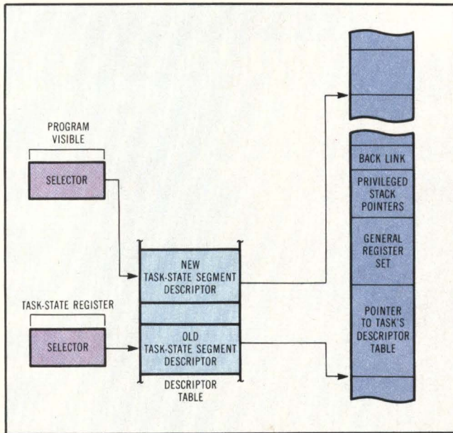
Fig 4 Just as with address translation, programmers are not bothered with the details of a task switch. Instead, after loading the task-state register with the selector to a new task-state segment's descriptor, they let the CPU bring in the information that specifies a task's state. This is contained in the task-state segment.
