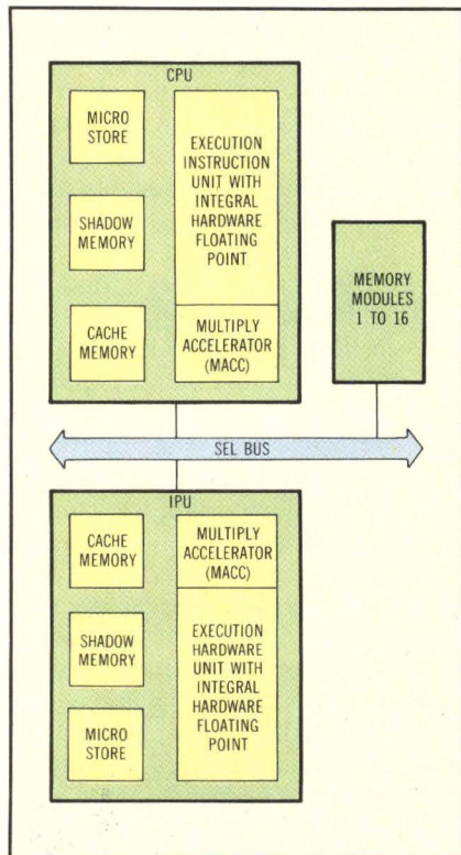
Functional units within the central and internal processing units that form the Concept 32/9780 are connected by internal buses that have 75-ns cycle times. During each 75-ns cycle, 4 macroinstructions are in various phases of execution, increasing the effective throughput of the system.
