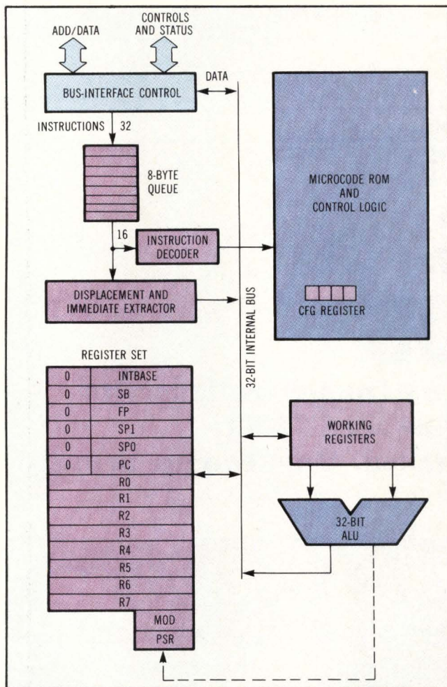
Fig 1 The NS32032 bus interface control unit makes 4-byte instruction transfers into an 8-byte queue. From there, instructions are decoded and passed to the execution unit. An intermediate preprocessor selects and runs microcode for address computation, operand fetching, execution, and result storage.
