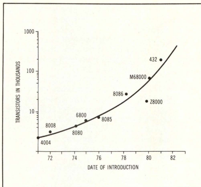
Fig 1 A microprocessor development curve shows the growth of transistor density, over time, in the attempt to wring more performance from what is essentially the same architecture.
