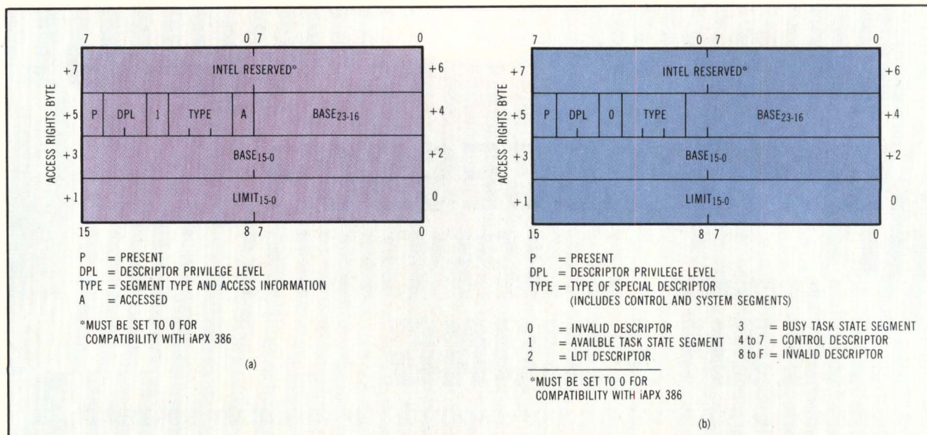
Fig 1 The 80286 segments all operations. To refer to these segments, the CPU uses one type of descriptor for code and data (a) and others for maintaining special structures like those used in multitasking (b).
