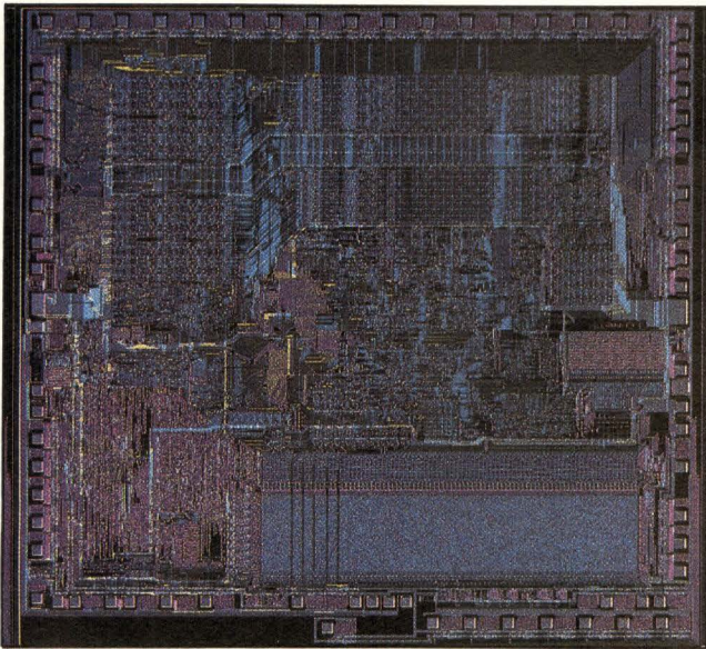
National Semiconductor's NS32032 is the first 32-bit chip available from a mainline semiconductor supplier. Like other members of the NS16000 family of microprocessors, it is organized to optimize support for high level language.
