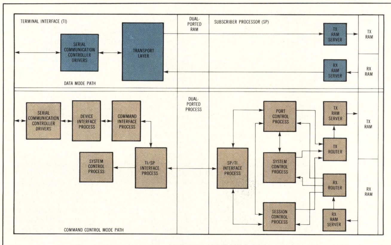
Fig 3 This modular software design follows the layering scheme promulgated by the International Standards Organization in its Open System Interconnection model. Software residing in the subscriber processor supports session layer functions while software on each device interface supports transport, presentation, and application layer functions. Transmit (TX) and receive (RX) RAM resides on the device interface.
