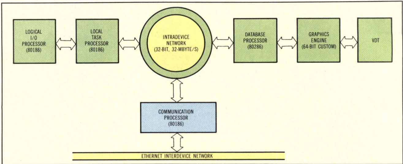
Distributing functions among several processors, the Merlin 9200 increases parallel processing. A 32-bit backplane serves as the network for interprocessor communications.
