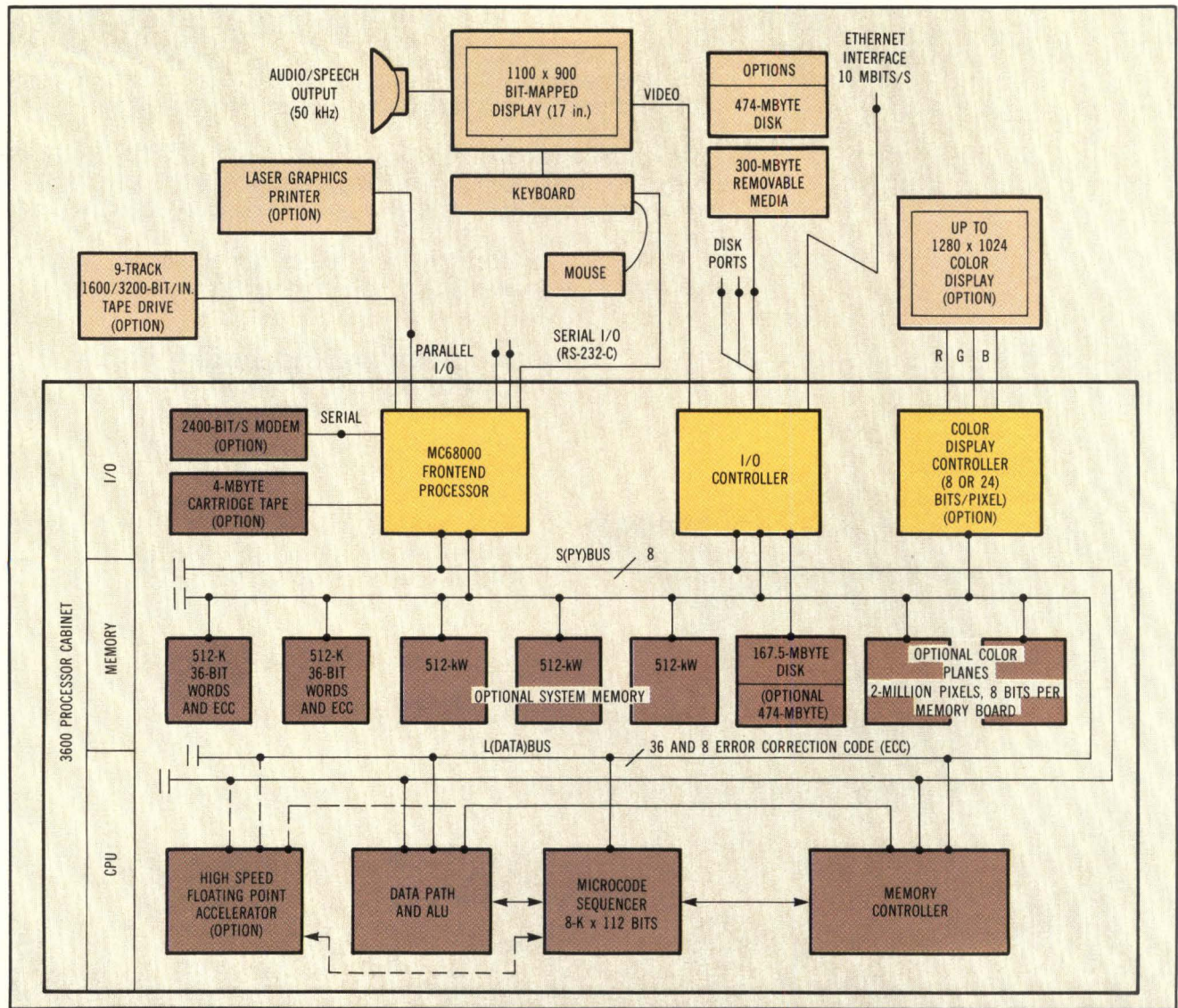
Fig 4 Like all computers, the 3600 symbol processor consists of three sections: CPU, memory, and I/O. However, the stack-oriented CPU and memory tagging provide an organization specifically designed for Lisp processing.
