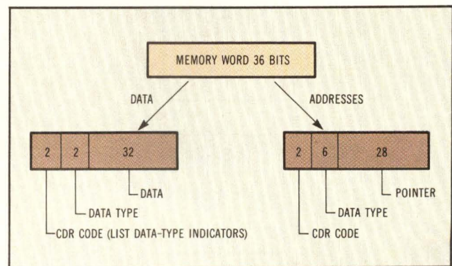
Fig 1 There are two basic formats for 36-bit words. The immediate number format consists of a 2-bit tag, a 2-bit contents of data register (CDR) code and 32 bits of immediate numerical data. The tagged pointer format consists of a 6-bit tag, 2-bit CDR code, and 28-bit data structure address.
