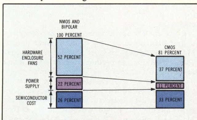
Fig 2 Despite higher semiconductor costs, CMOS reduces overall system costs by decreasing both cooling and power supply equipment.
