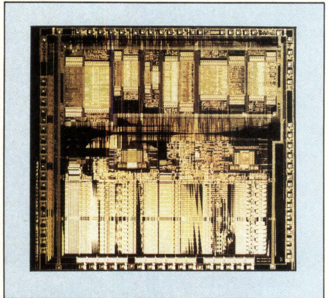
The WE32000 32-bit microprocessor has been available within AT&T for some time. A more advanced version, the WE32100, was recently introduced. However, there are no plans to make either chip available outside AT&T.
