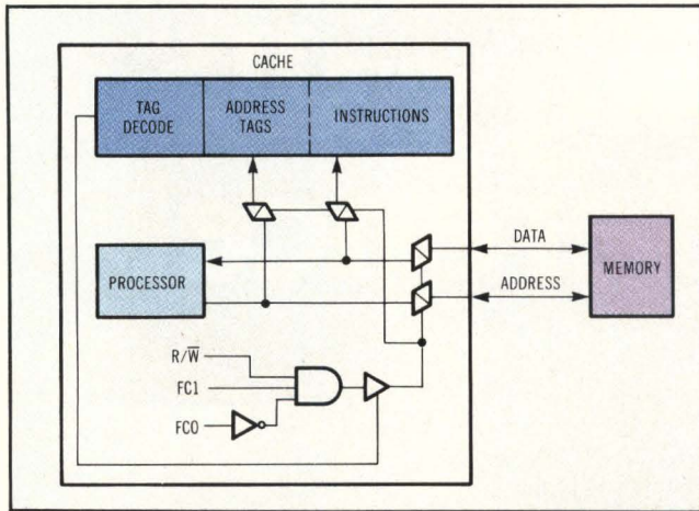
Fig 4 Because of the pipelined internal architecture of the Motorola MC68020, the ALU can execute instructions faster than they can be fetched from external memory. To permit the chip to run at full speed, an instruction cache is built into the chip. This cache is used only for instructions, not for data.
