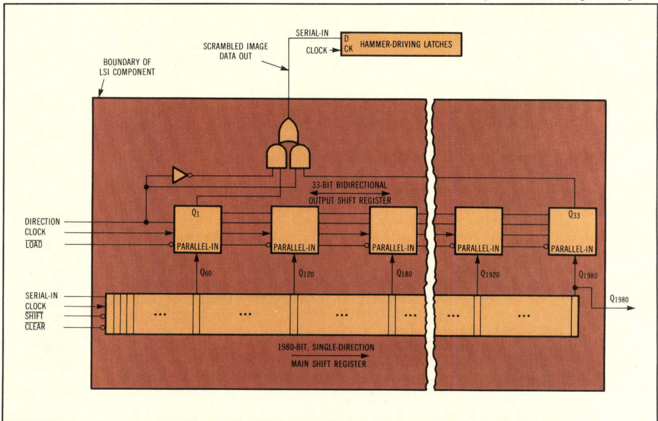
Fig 3 This 1980-bit LSI shift-register component supports a 33-hammer line printer at 150 dots/in. The hammers, 0.4 in. apart, can reach and print 60 dots. A 33-bit bidirectional shift register supports the main register and compensates for the print-bar direction.
