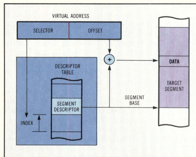
Fig 2 An address in the 80286 is comprised of an offset and a selector. In virtual addressing, the selector is used as an index into a table of descriptors for building the physical address. In real address mode, instead of the operation indicated in the shaded portion of the figure, the CPU multiplies the segment selector by 16 and adds the result to the offset to point to the desired location in memory.
