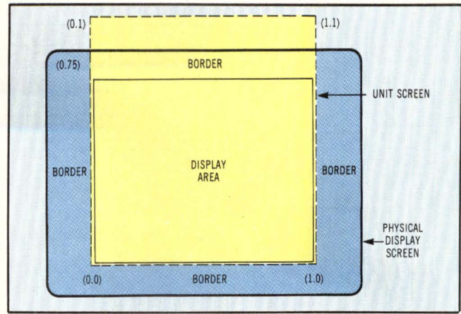
Fig 4 The NAPLPS standard adheres to the unit screen concept. This means that all coordinate data is transmitted as fractions of the unit screen, thus making the NAPLPS standard resolution independent.
