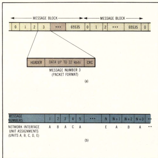
Fig 1 The UniLINK scheme divides time into numbered message blocks allocated to specific network interfaces. Each message includes a header, data, and cyclic redundancy check (CRC), as shown in (a). UniLINK operates on either a contention or dedicated basis. In the latter type (b), assigning more message numbers to certain interfaces gives these interfaces priority, thus improving on typical CSMA/CD schemes.
