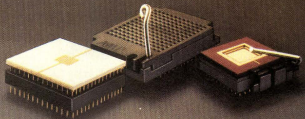
AMP Pin-Grid Array Sockets: Up to 324 positions in 18 x 18 array. Zero- and low-insertion force production versions, plus a zero-insertion force test socket.
