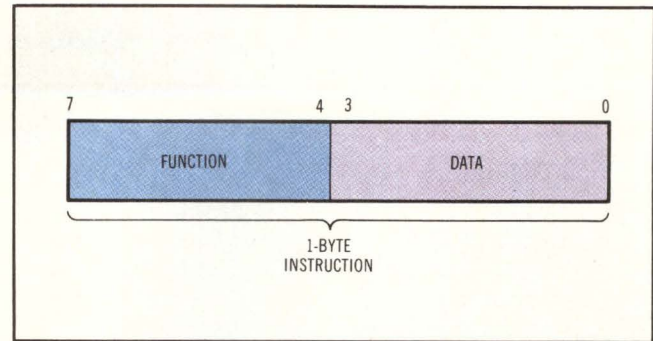
Fig 5 In the instruction set, all instructions are 1 byte long. The 4 MSBs represent a function code and the 4 LSBs are data.
