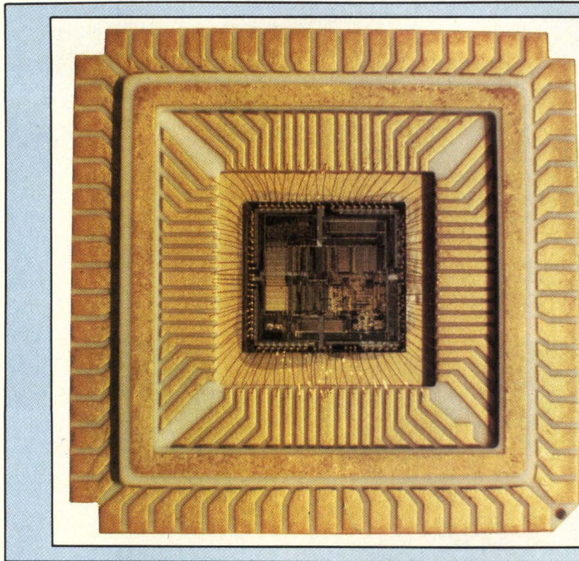
The NCR/32 VLSI processor family contains the only micros designed to emulate existing midrange mainframes. Shown here is the NCR 32-000 central processor chip, the heart of the chip set. This externally microprogrammable VLSI system is currently available.
