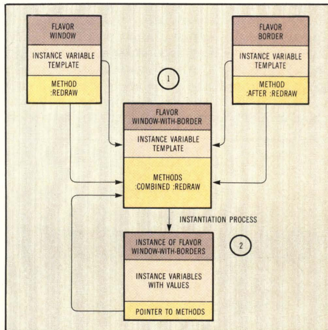
Fig 3 The Flavors system (abstract type) can be combined to form new flavors (see No. 1). When generic flavors are provided with specific variables, flavor instances (objects) that can be manipulated by sending messages (requests for specific operations) are produced, as shown in No. 2.
