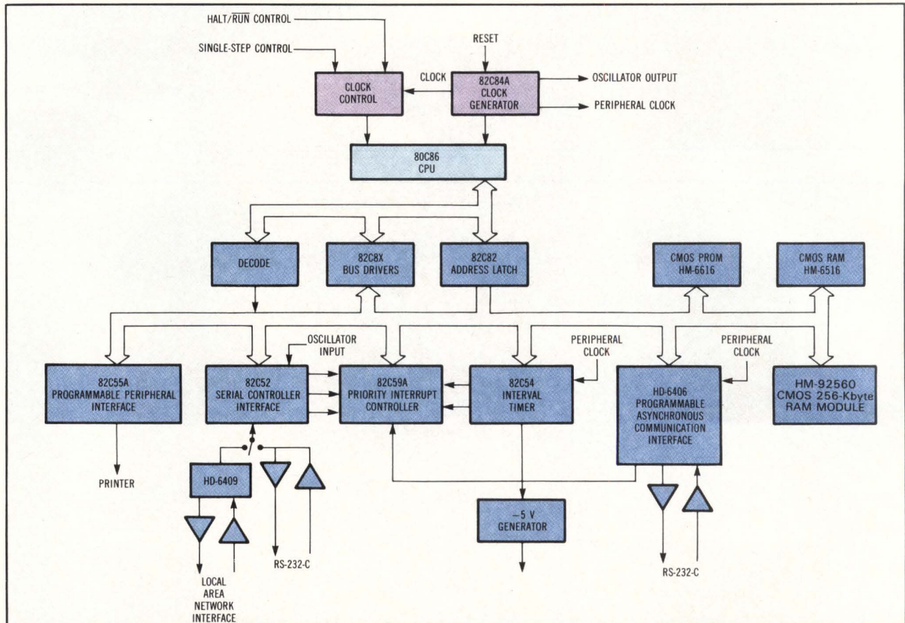
Fig 3 The CPU input board built around the 80C86 processor chip shows a CMOS approach to building a 16-bit processor. This prototype system also features a completely static design and a parallel interface using the 82C55A programmable peripheral interface.
