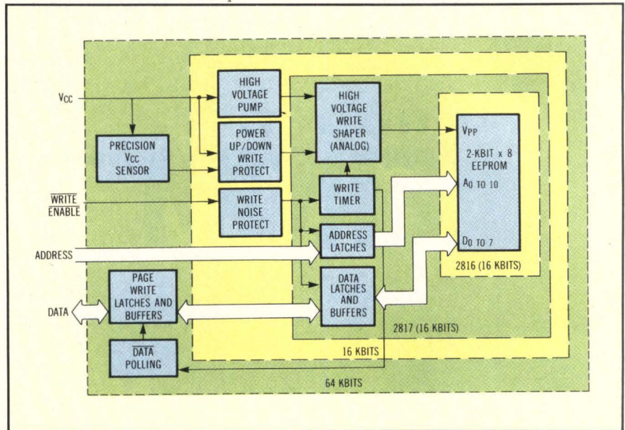
As EEPROM densities have increased, peripheral circuits and features incorporated onchip have grown. Features at the 16-Kbit level evolved through several stages. The 64-Kbit level has demanded even more. (Source: Xicor Corp)
