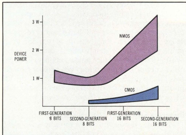
Fig 1 As shown, the power dissipation of complex 16-bit NMOS microprocessors is reaching a limit. This is causing a move to CMOS.
