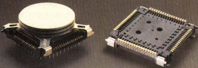
AMP Low-Height Chip Carrier Sockets: Duplex plated contacts eliminate solder-bath contamination. Surface-mount or through-hole versions, overall installed height 0.275" for 44-84 positions, 0.350" for 100 positions, to allow 0.500" pc board spacing.
