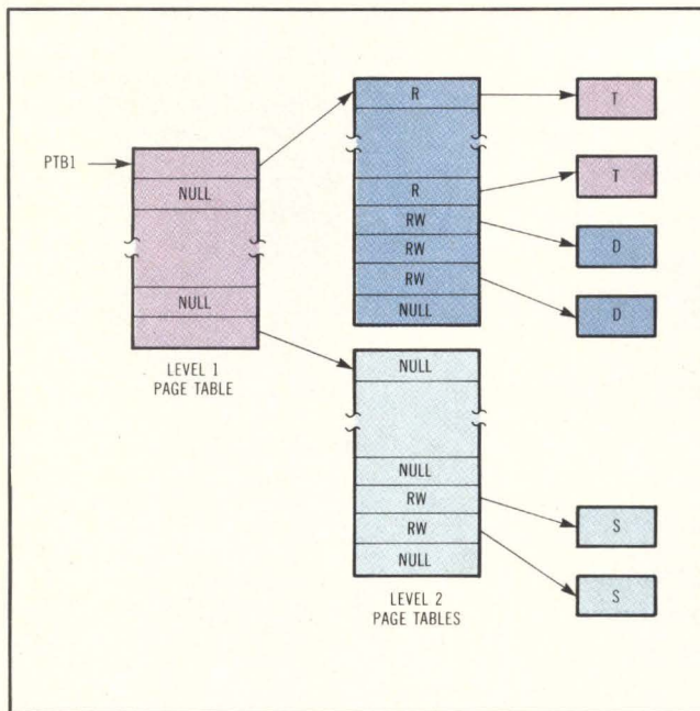
Fig 2 This user process map shows that in the NS16000 memory management scheme, the first-level page table entries point to second-level page table entries, which in turn point to the text (T), data (D), or stack (S) areas. Protection is provided in hardware. Text is read only (R), data is read/write (RW), and the stack is read/write.
