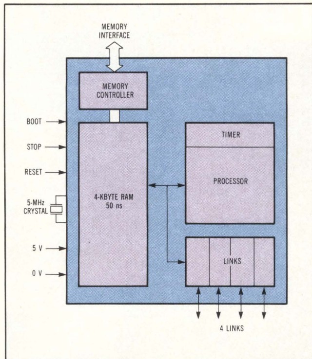
Fig 3 The IMS T424, 32-bit transputer contains a 10-MIPS processor, 4 Kbytes of 50-ns RAM, and four 1.5 Mbyte/s full-duplex communication links. It addresses 4 Gbytes of memory and has an external memory bandwidth of 25 Mbytes/s. Implemented in a 2- \mu m CMOS process, the chip contains 250,000 devices.
