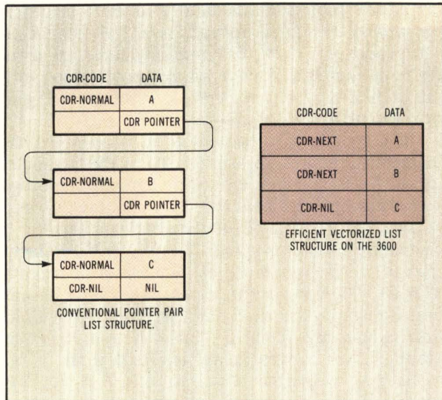
Fig 2 An analysis of Lisp CDR coding, comparing conventional computer architecture Lisp implementations (a) to tagged architecture (b), is shown.
