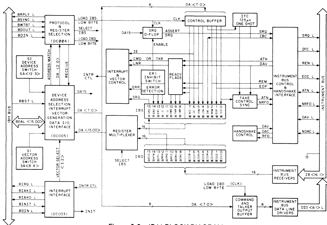
Figure 6-9 IB11 BLOCK DIAGRAM
