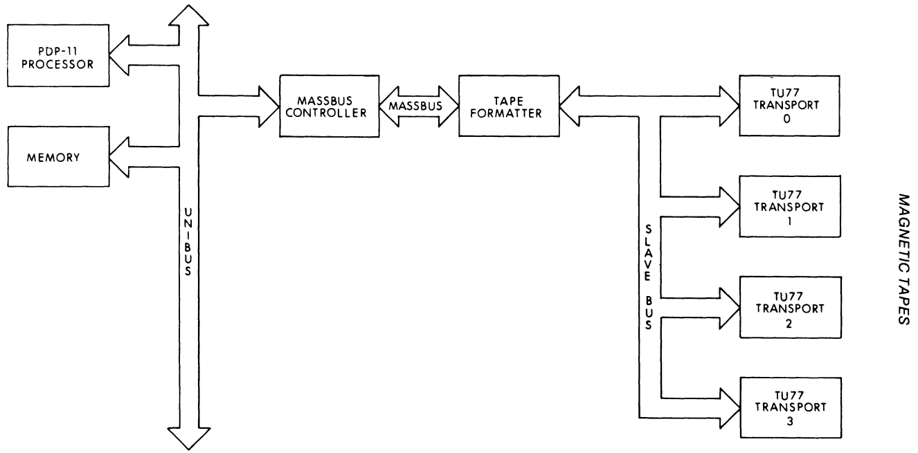
Figure 3-12 TJU77 SYSTEM BLOCK DIAGRAM
