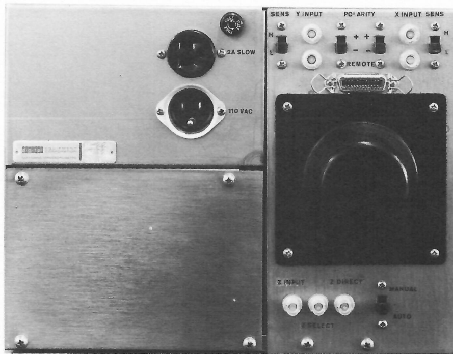
Figure 8-5 VP15C Oscilloscope Display, Rear View
