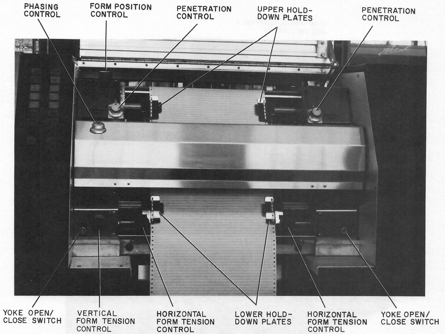
Figure 4-2 LP15C Line Printer Controls and Indicators
