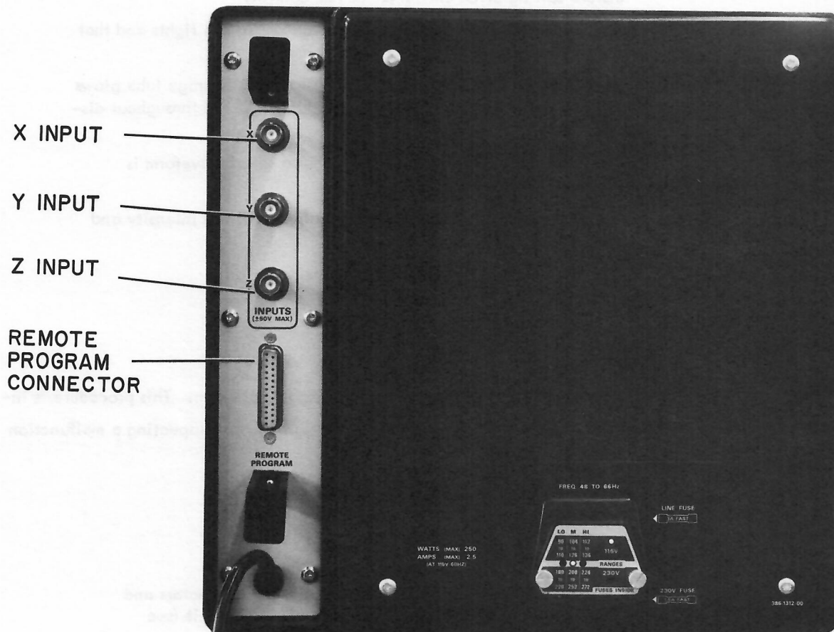
Figure 8-2 VP15A, Rear View
