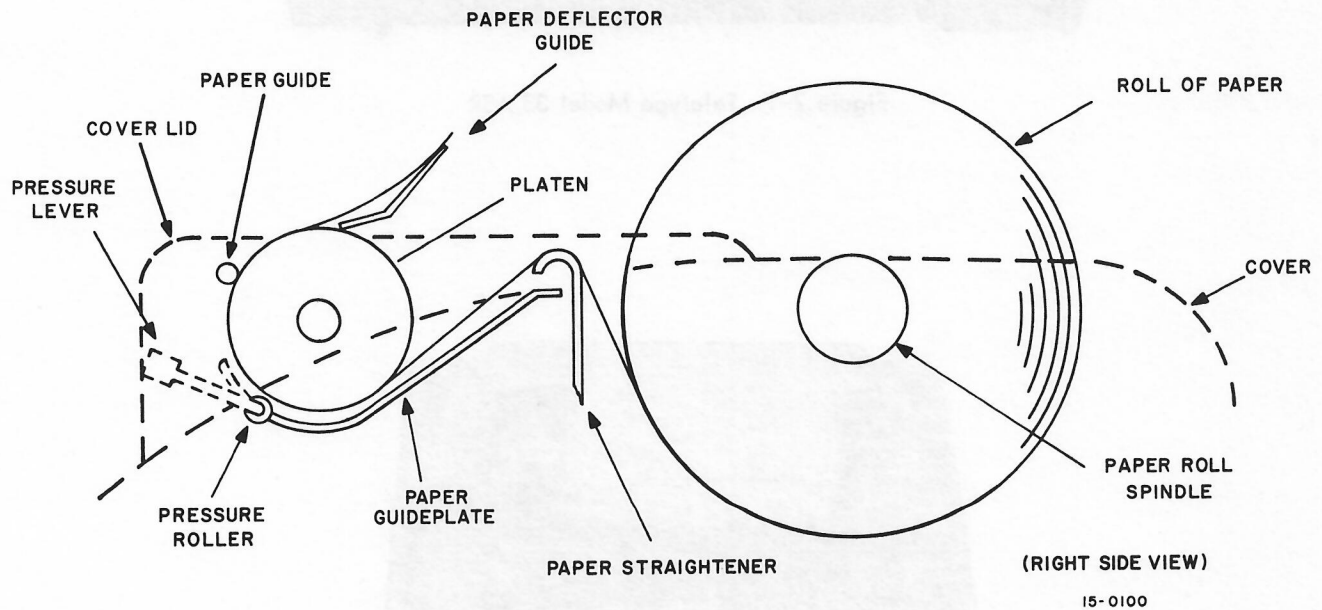
Figure 2-3 Roll Paper Installation*
