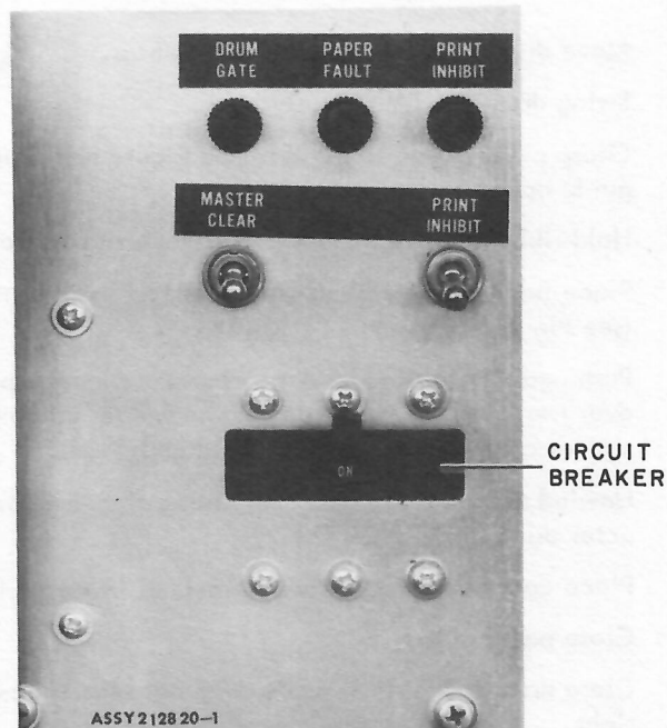
Figure 4-17 LP15F Inside Control Panel
