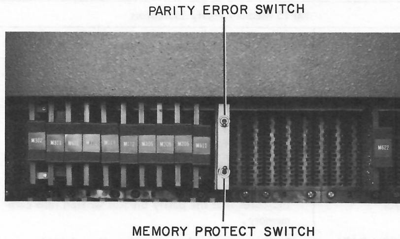
Figure 1-5 BB15 Control Switches
