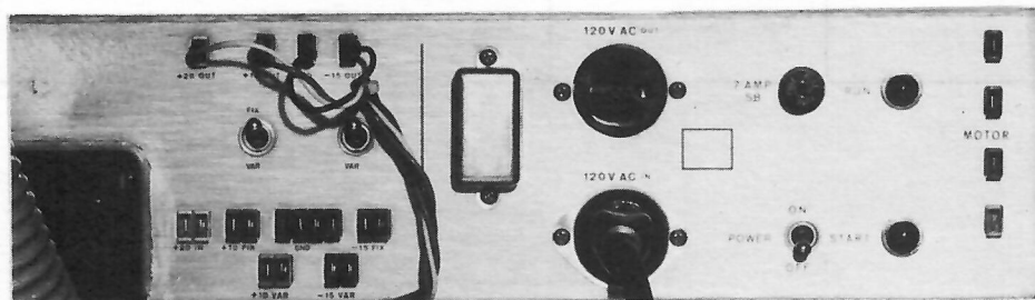
Figure 6-6 RS09 DECdisk Drive, Power Controls and Indicators
