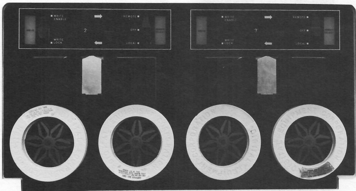
Figure 7-8 TU56 Dual DECtape Transport
