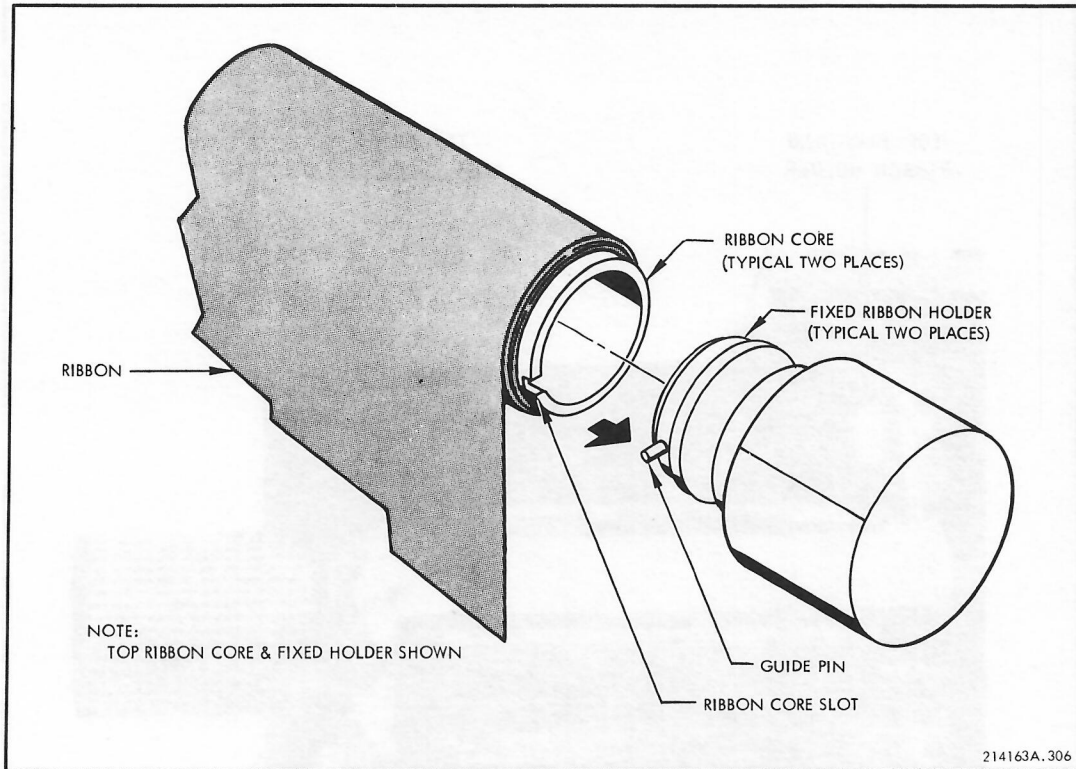
Figure 4-19 Installation of Ribbon Core on Fixed Ribbon Holder*
