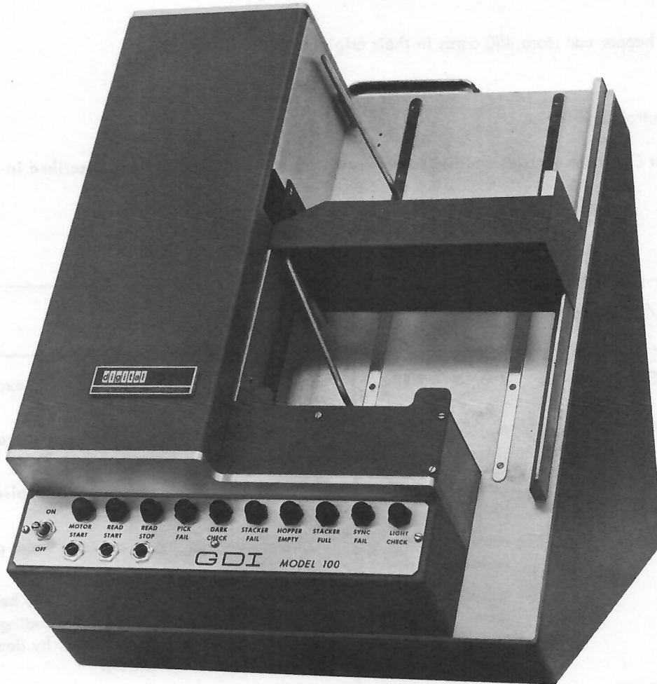
Figure 3-1 Card Reader CR03B
