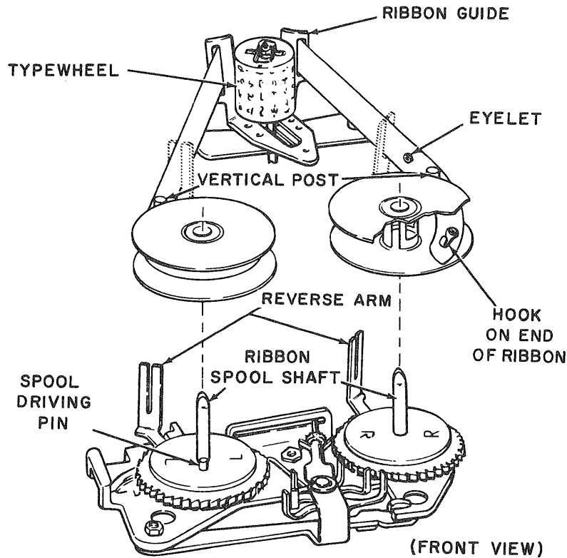
Figure 2-5 Ribbon Installation*
