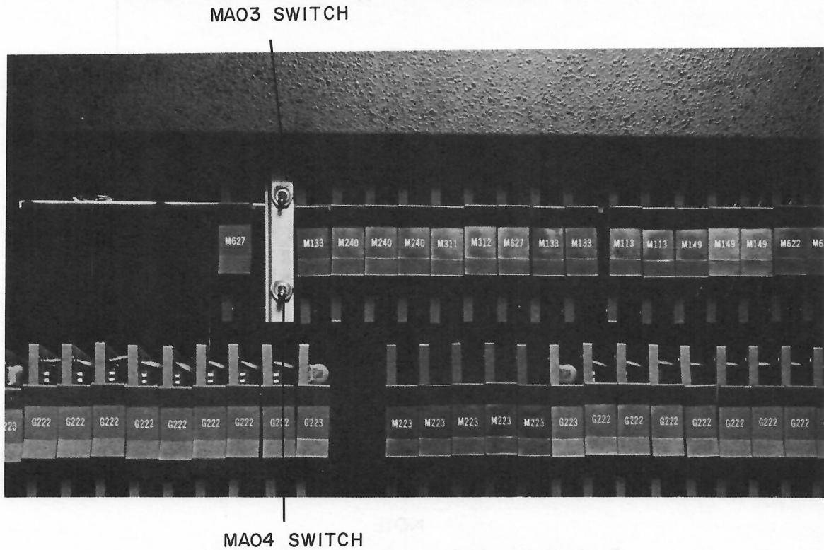
Figure 1-3 Memory Bank Selection Switches
