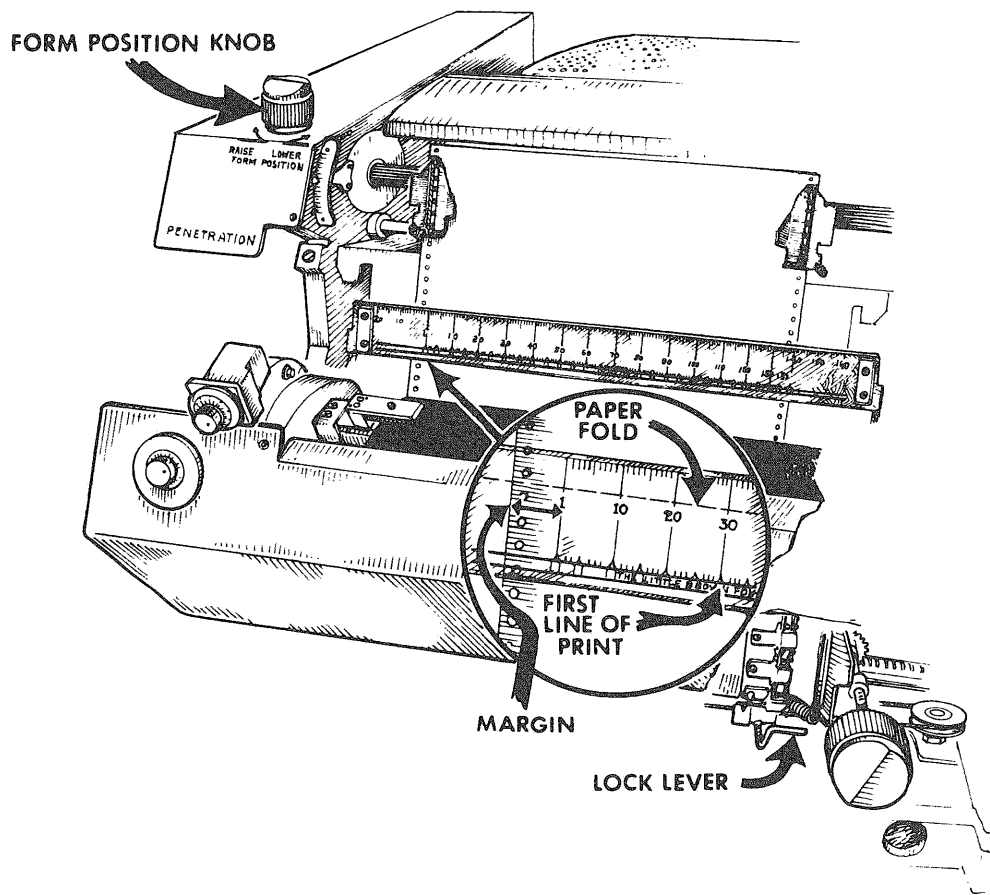
Figure 4-10 Paper Alignment*
