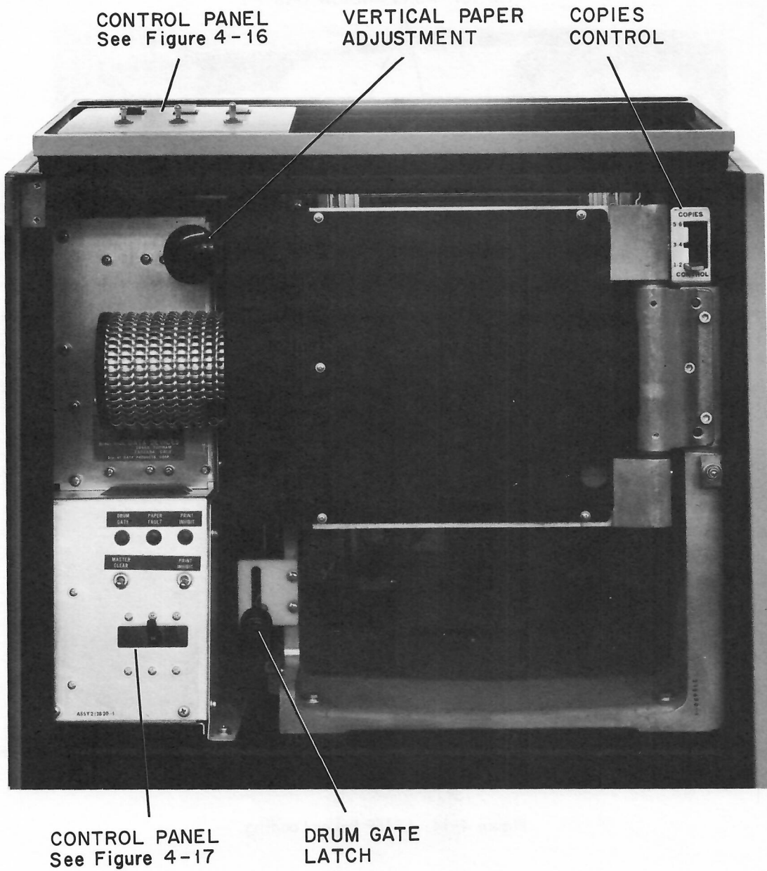
Figure 4-15 LP15F Line Printer Controls
