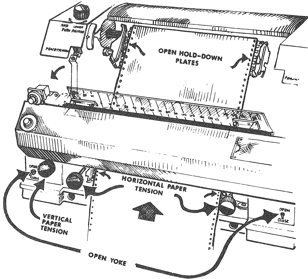
Figure 4-9 Paper Loading*
