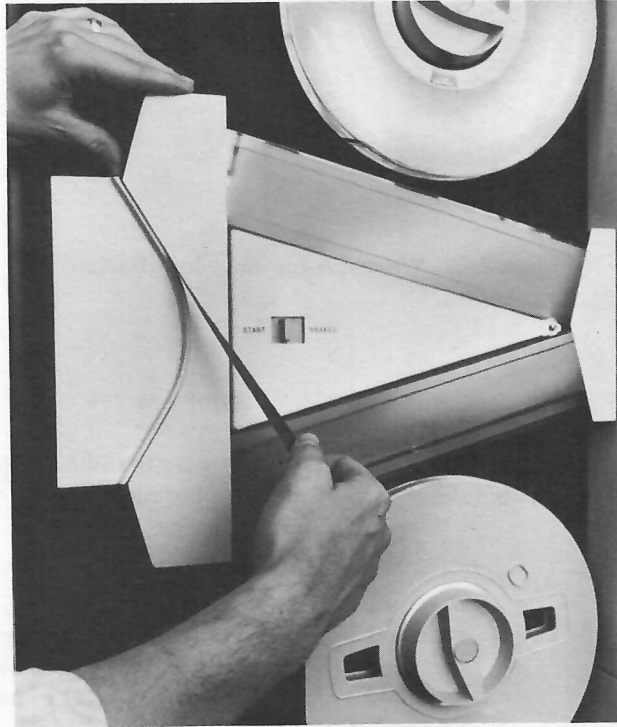
Figure 7-4 Starting Tape in Tape Insertion Slot
