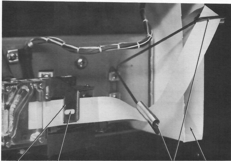
BACKING PLATE OUT-OF-TAPE SWITCH (BELOW TAPE) TAPE GUIDES FEED BOX
