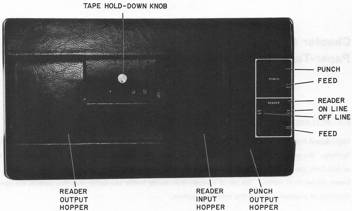
Figure 5-1 Paper-Tape Reader and Punch
