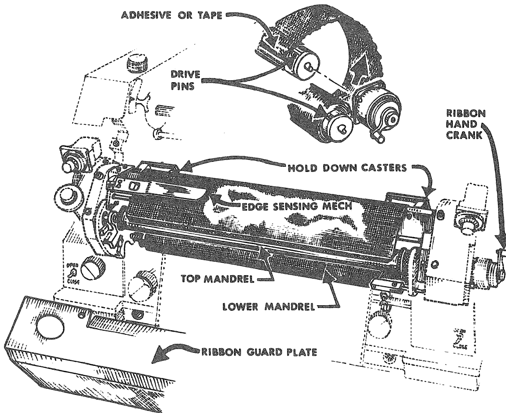
Figure 4-11 Ribbon Installation*
