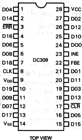
Figure 2 • DC309 Pin Assignments
