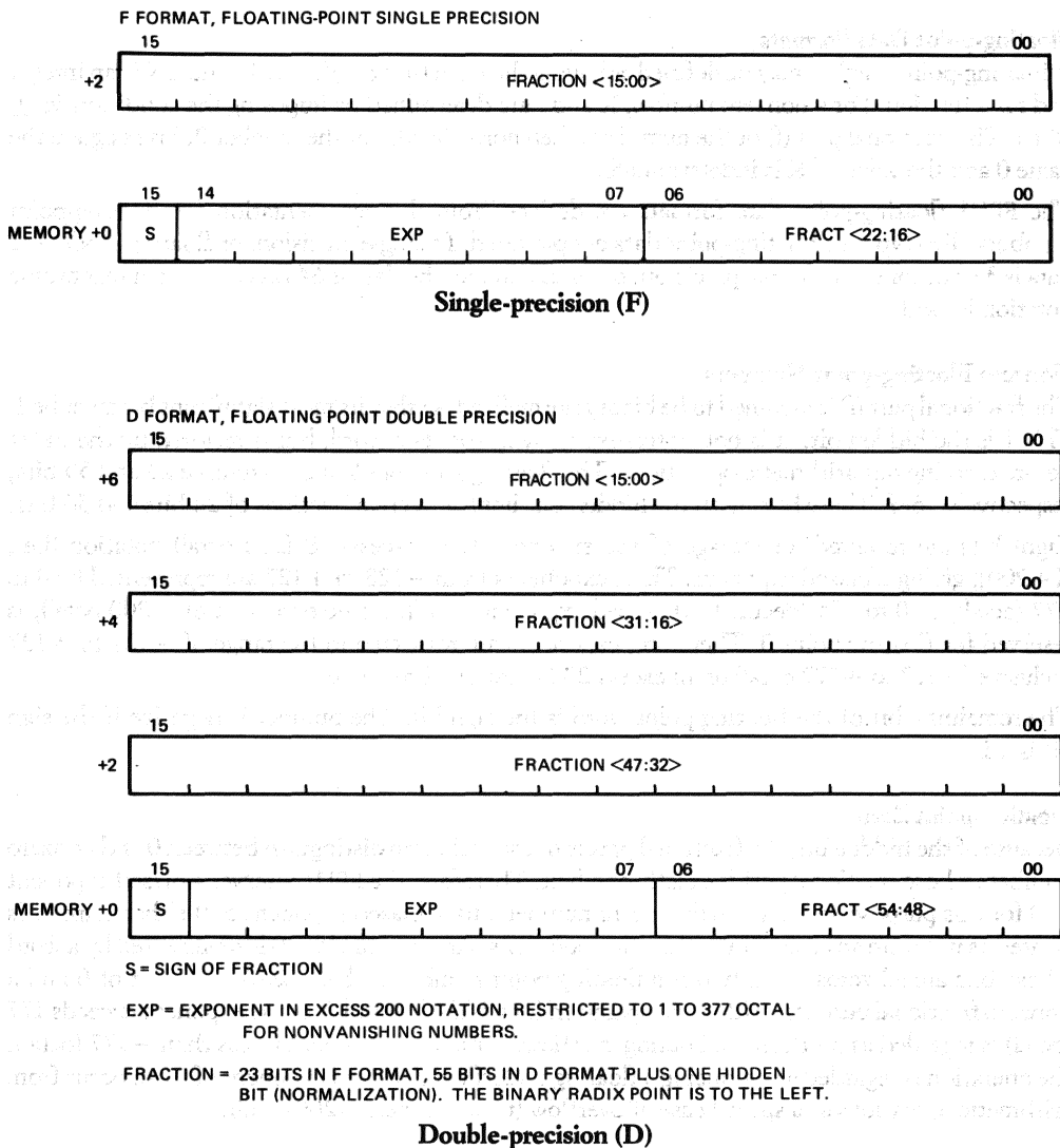
Figure 4 • FPJ11 Floating-point Data Formats
