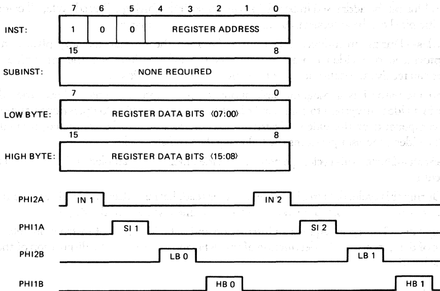
Figure 4 • 78680 Register Load Data Transfer Model
