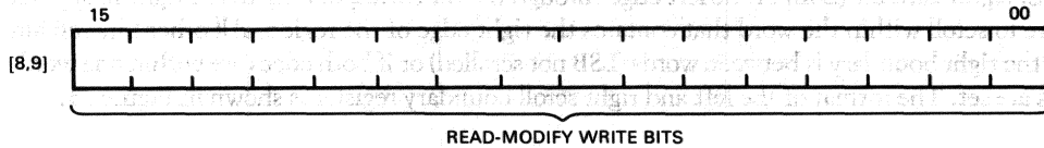
Figure 10 • 78680 Data Mask 1 and 2 Register Format
