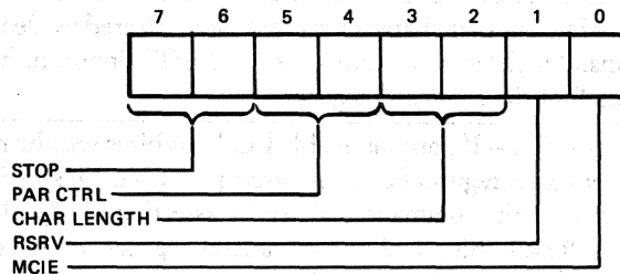
Figure 4 • 78808 Mode Registers 1 (Line 0-7) Format
