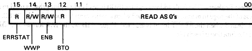
Figure 3 - MicroVAX 78584 Control Status Register Format
