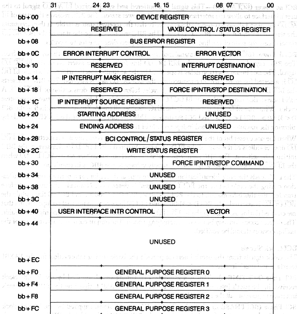
Figure 5 • VAXBI 78732 BIIC Registers and Address Assignments
