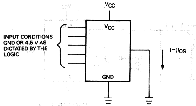
DC TEST CIRCUIT C6
