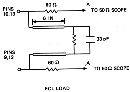
Figure 8 • VAXBI 78701 ac Load Circuits
