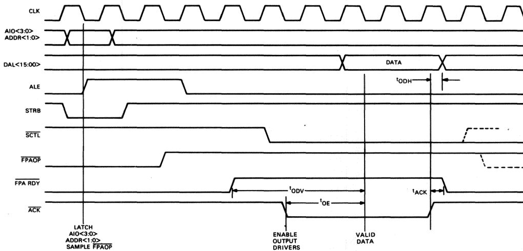
Writes with FPA RDY Asserted before \overline{SCTL}
