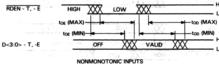
Figure 8 • DC022 Enable and Disable Signal Timing
