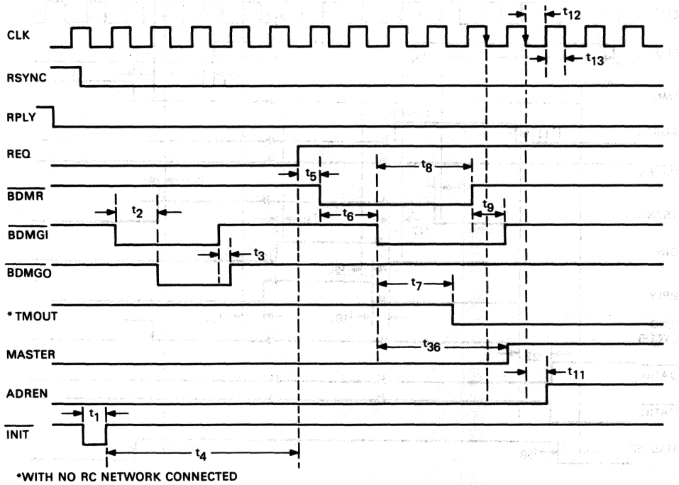
Figure 3 • DC010 DMA Bus Request and Grant Signal Timing Sequence
