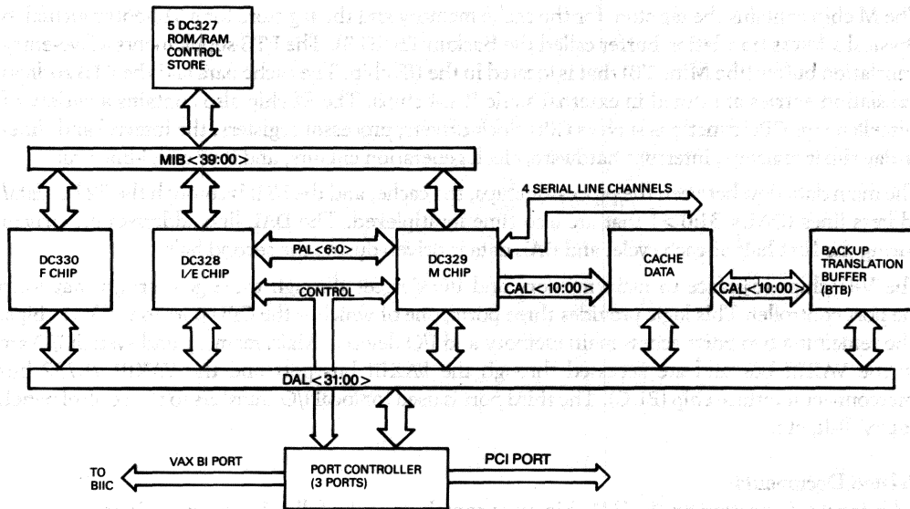
Figure 1 • V-11 Scorpio Microprocessor Block Diagram
