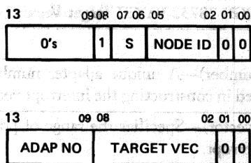
Figure 34 • VAXBI 78732 VAXBI Interrupt Vector Formats
