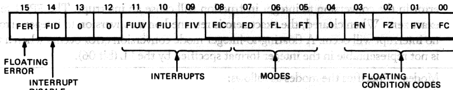
Figure 6 • FPJ11 Floating-point Status Register Format
