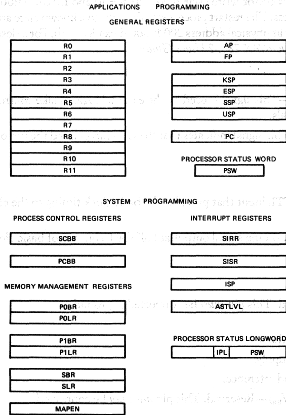
Figure 3 - MicroVAX 78032 Programming Model
