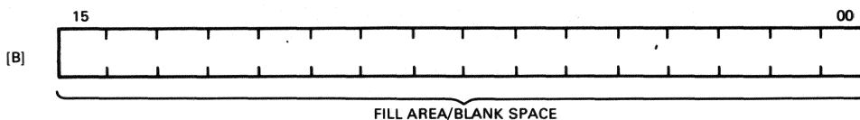
Figure 12 • 78680 Fill Register Format
