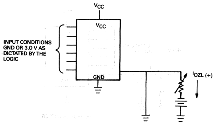
DC TEST CIRCUIT C8
