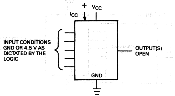
DC TEST CIRCUIT C7
