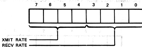
Figure 5 • 78808 Mode Registers 2 (Line 0-7) Format
