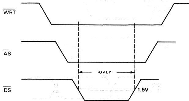
Figure 9 • DC503 Write and Data/Address Strobe Timing Delay
