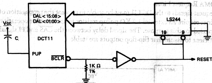
Figure 27 • DCT11 Typical Mode Register Load Circuit
