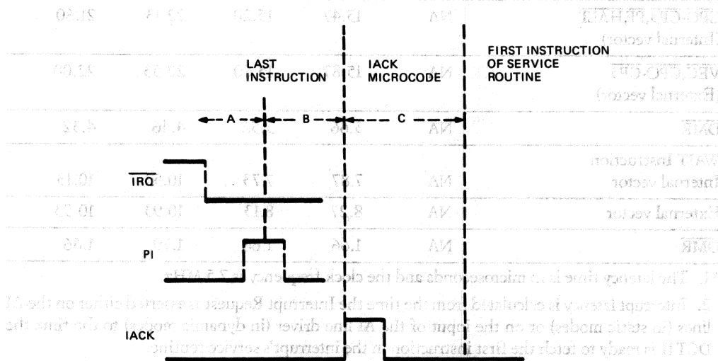
Figure 20 • DCT11 Interrupt Latency Measurements
