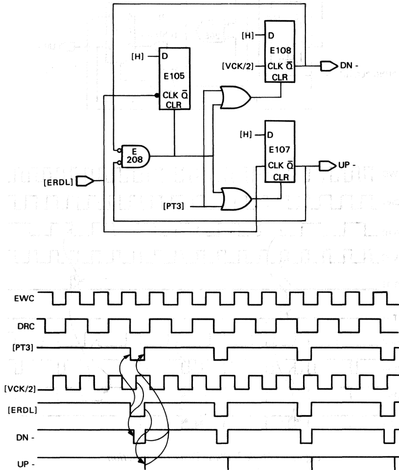
Figure 5 • Mode C Phase Detector Operation
