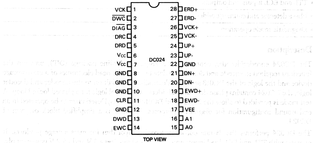
Figure 2 • DC024 Pin Assignments
