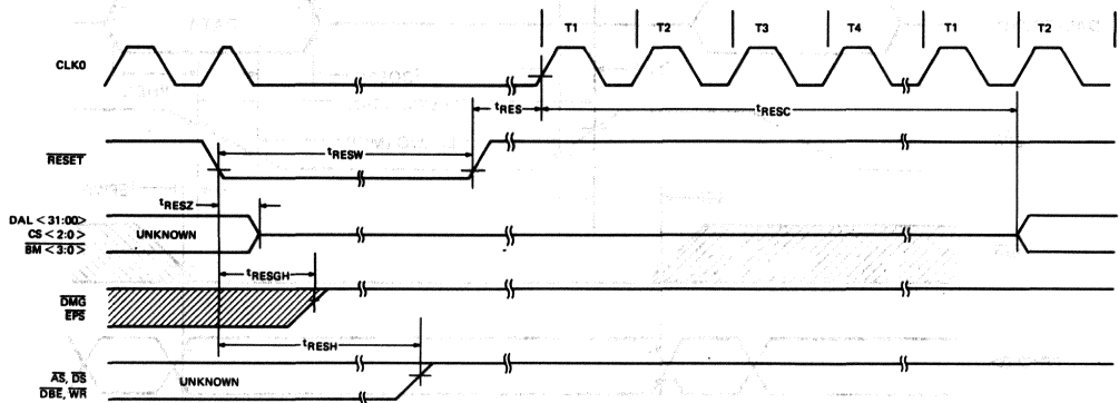
Figure 43 • MicroVAX 78032 Reset Timing Sequence
