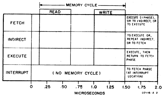
Figure 2-2. Machine Timing
