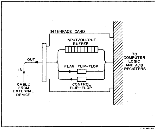
Figure 2-10. Components of Typical Input/Output Interface Card
