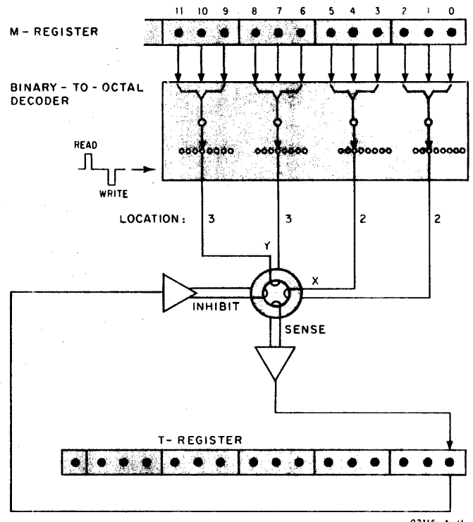
Figure 3-8. Core Addressing, Reading, and Writing
