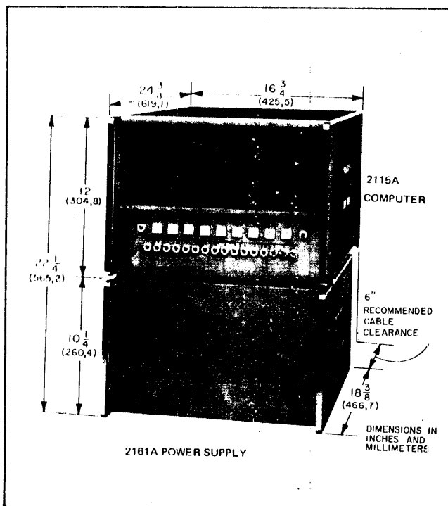
Figure 2-1. HP 2115A Dimensions (Showing HP 2161A Power Supply)
