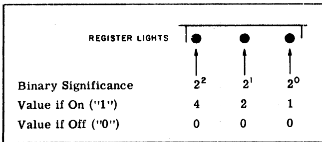
Figure 3-2. Composition of Octal Digit
