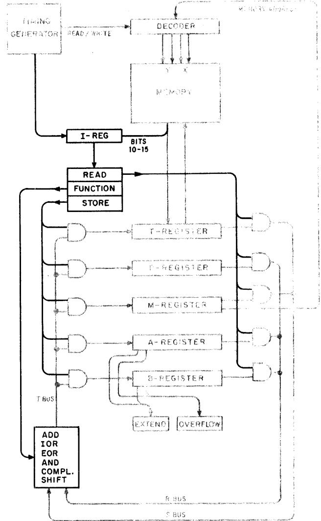
Figure 3-13. Instruction Logic Block Diagram
