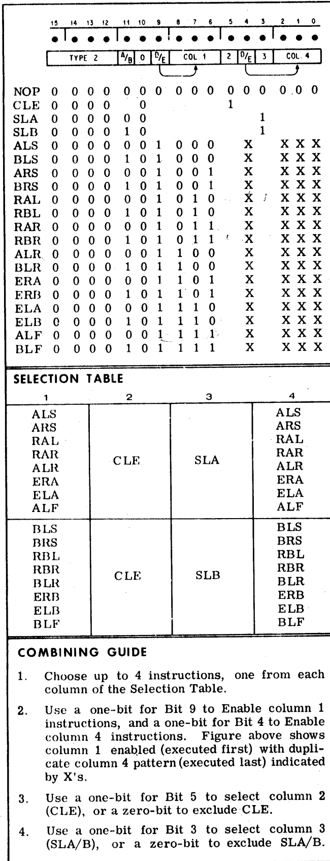
Figure 2-5. Shift-Rotate Instructions
