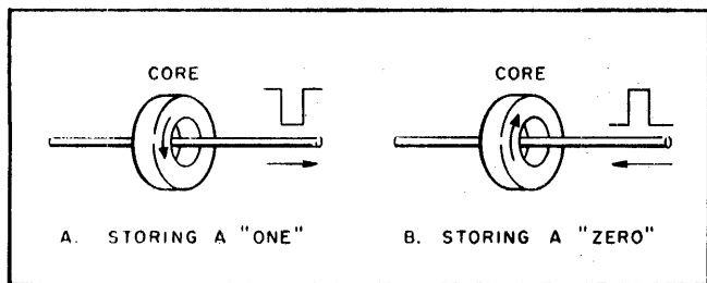
Figure 3-7. Binary Storage in a Magnetic Core
