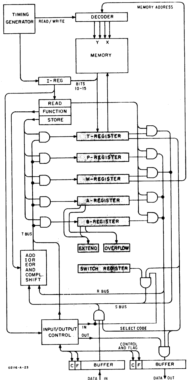
Figure 3-1. HP 2115A Simplified Block Diagram
