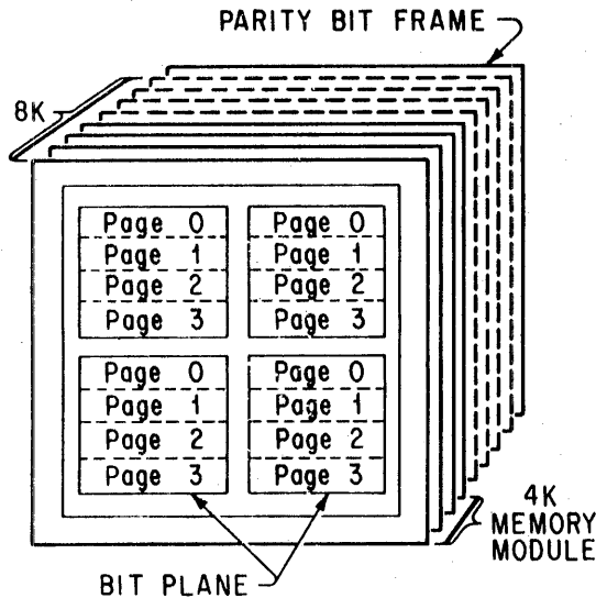
Figure 3-6. Core Memory Module
