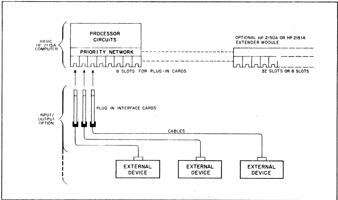
Figure 2-9. Input/Output Design Arrangement
