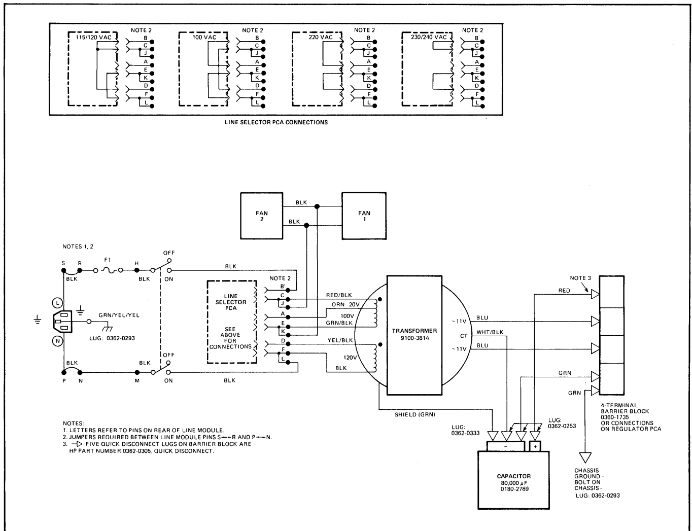
Figure A-5. Controller Power Distribution
