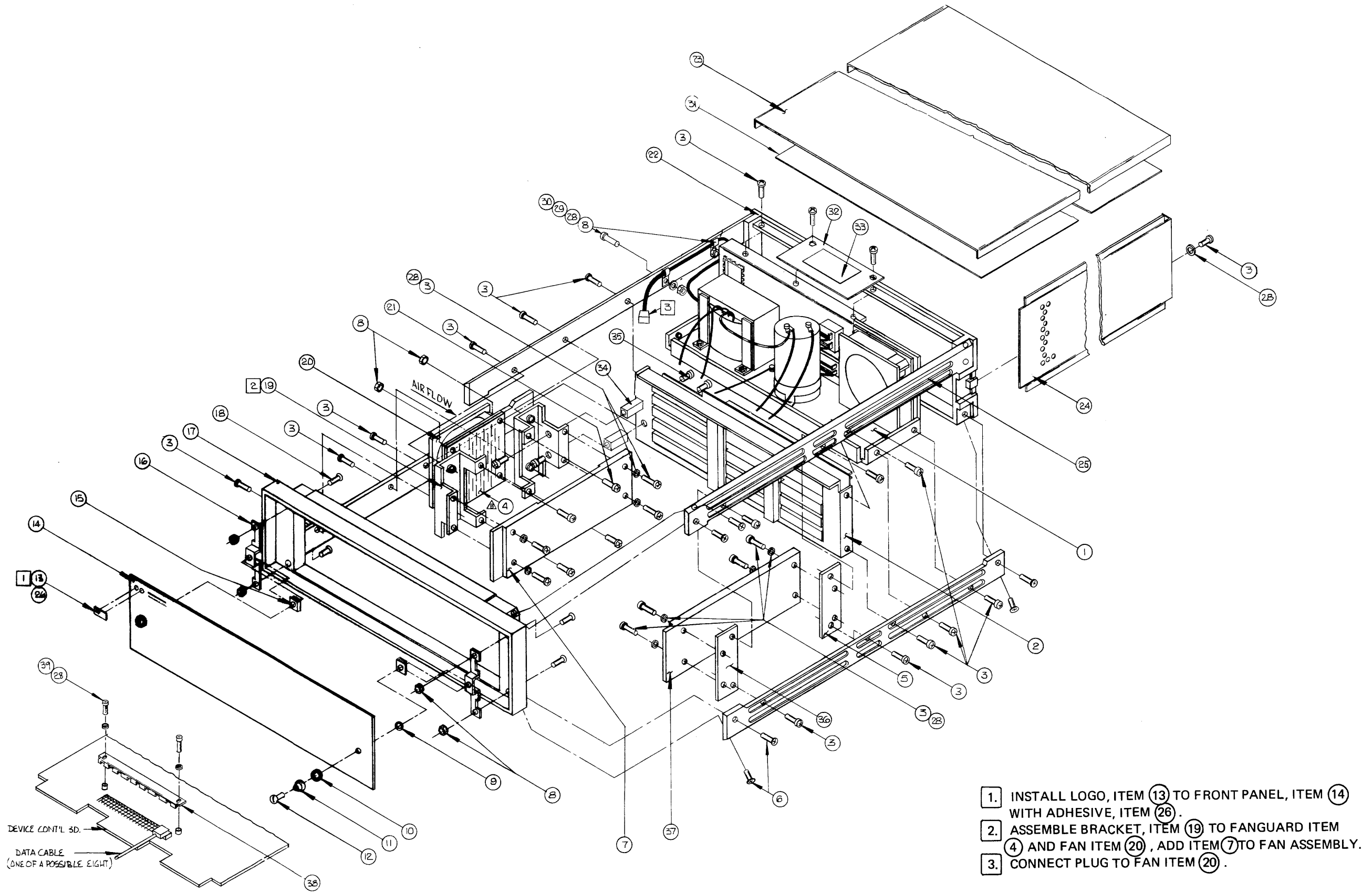
Figure A-6. Controller Main Frame Assembly
