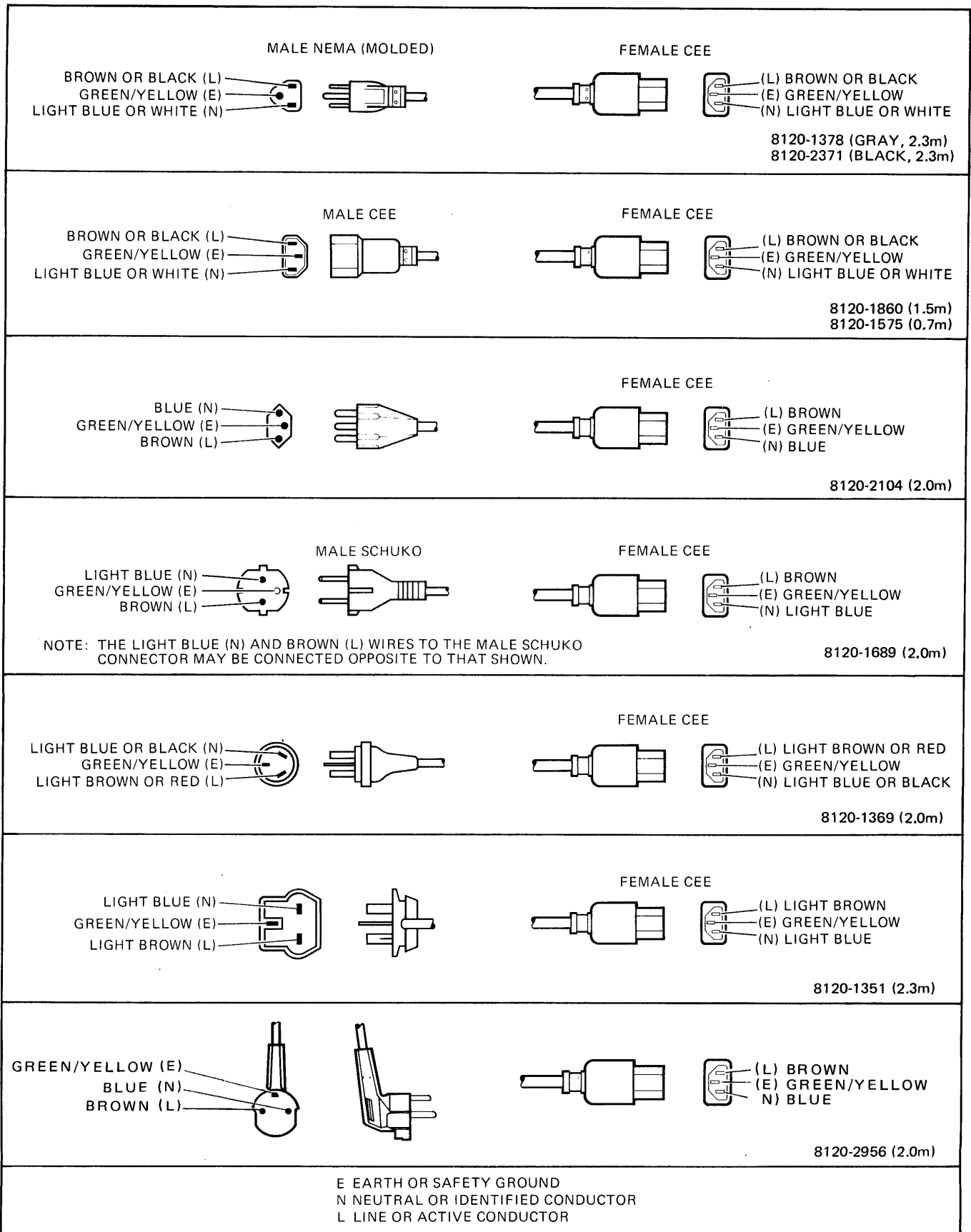
Figure 2-2. AC Power Cord Sets
