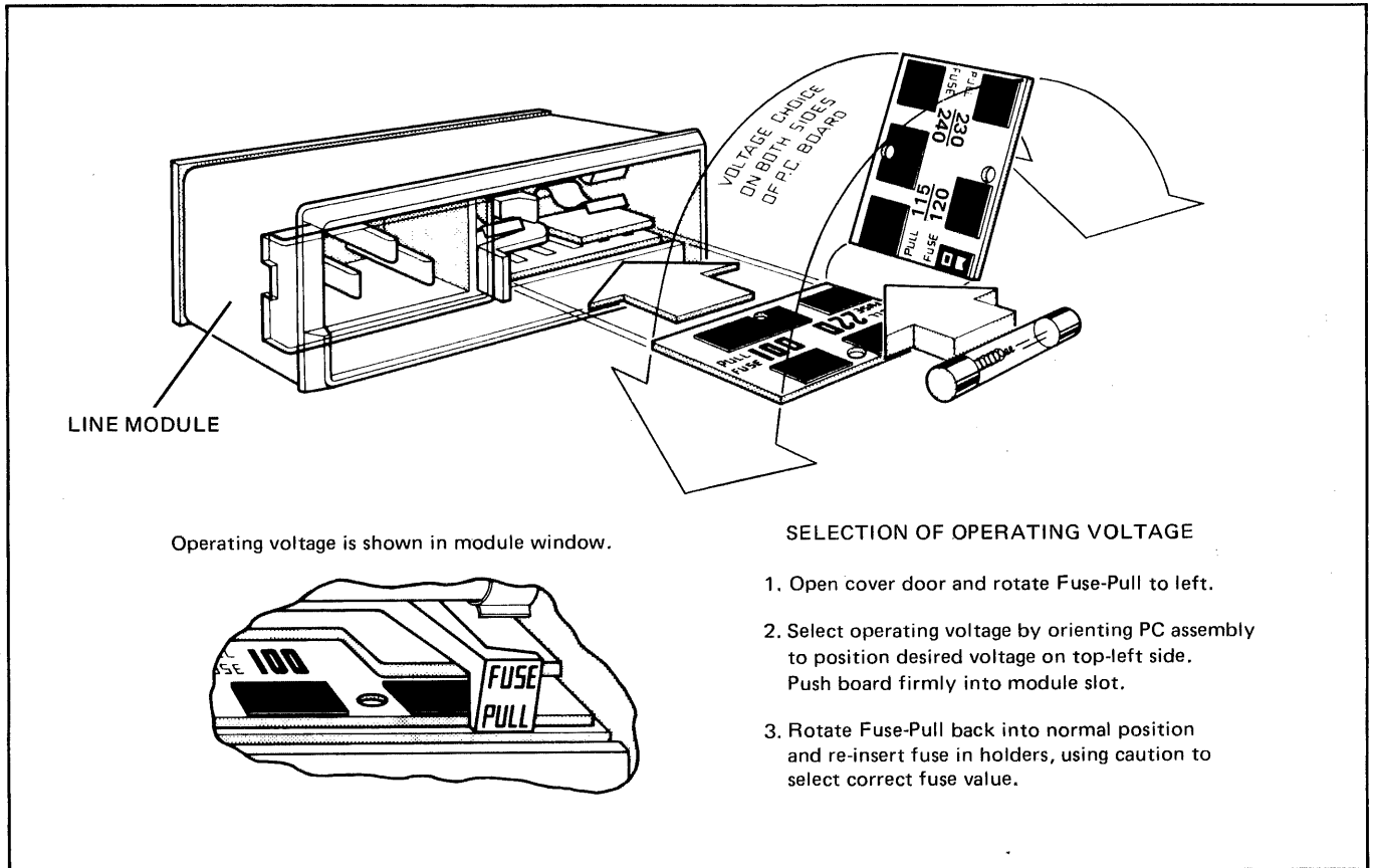
Figure A-1. Line Module Voltage Selection
