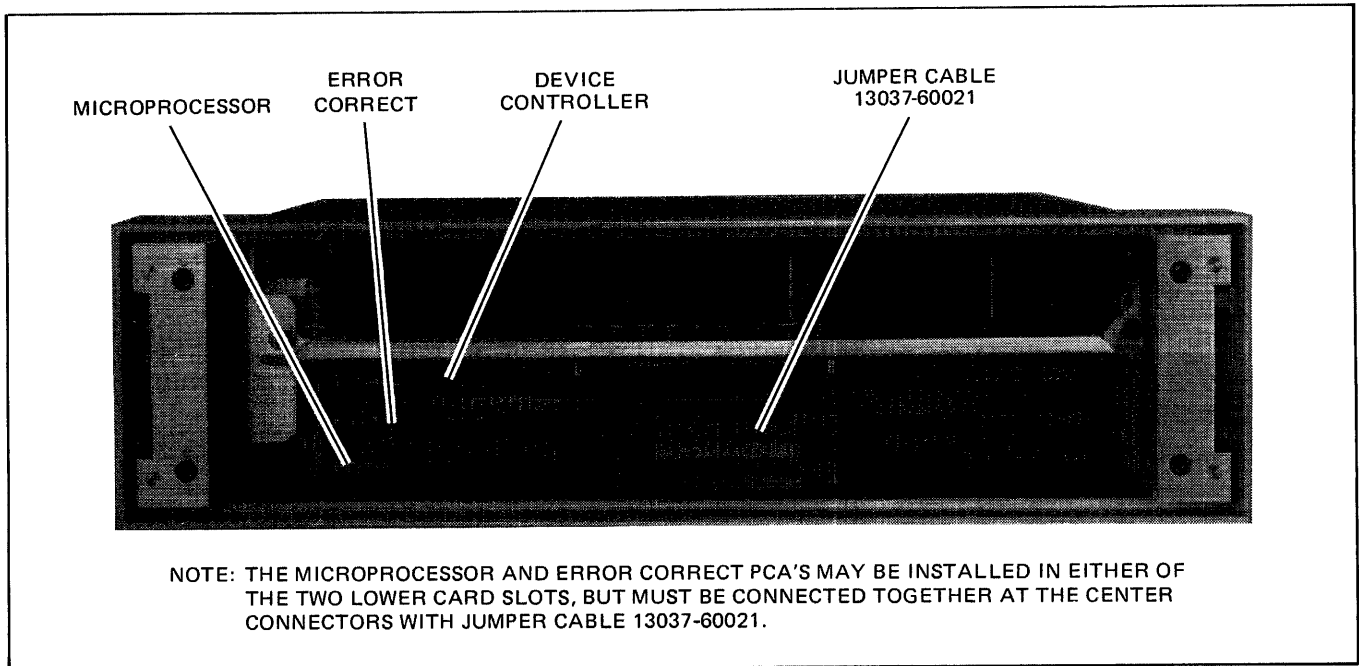
Figure 2-4. Controller PCA Configuration
