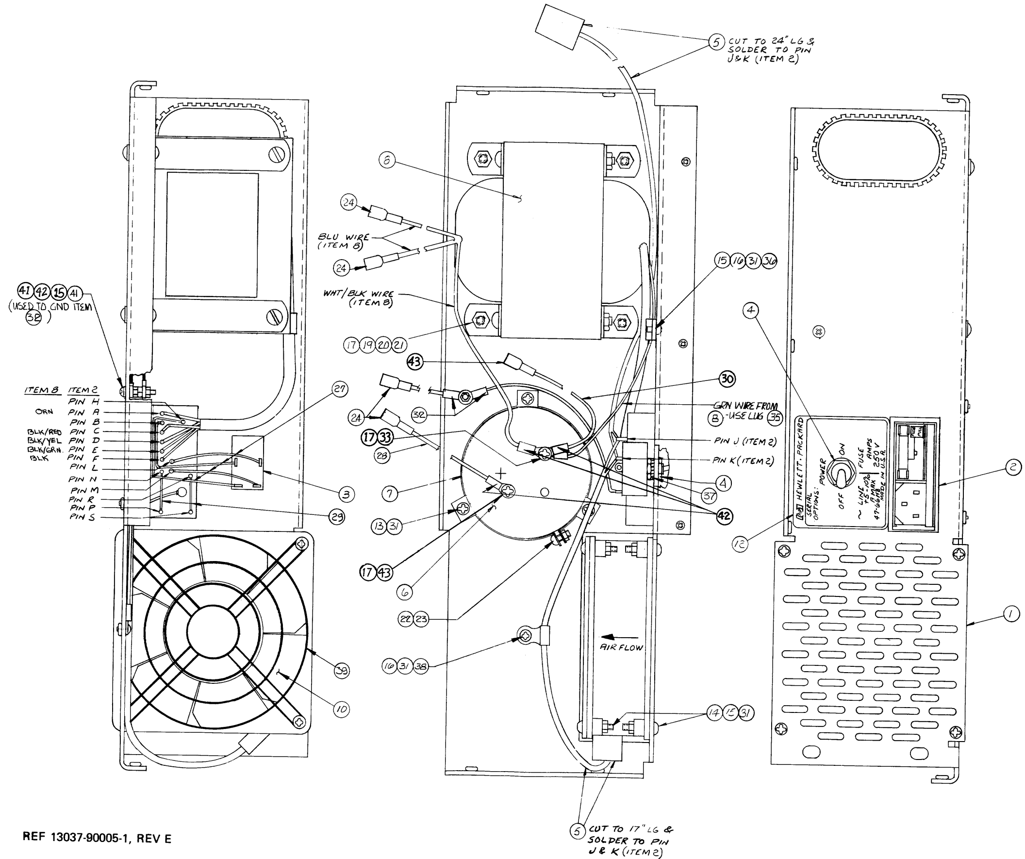
Figure A-8. Rear Deck Assembly
