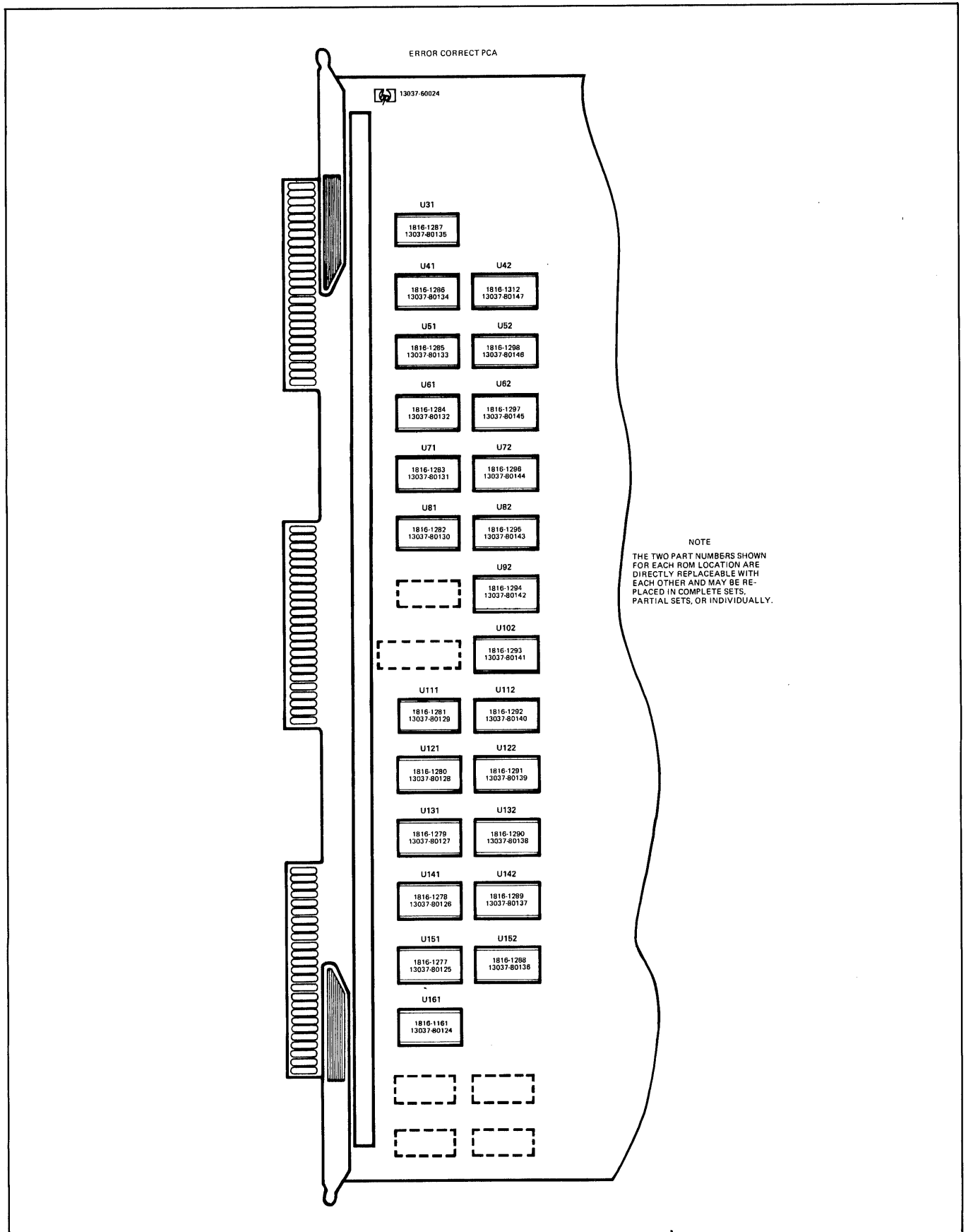
Figure 5-3. Error Correct PCA ROM Locations
