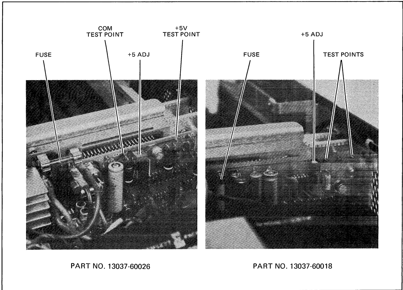
Figure A-2. Power Supply Adjustment and Test Points
