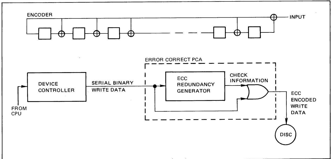
Figure 4-9. ECC Write Circuit
