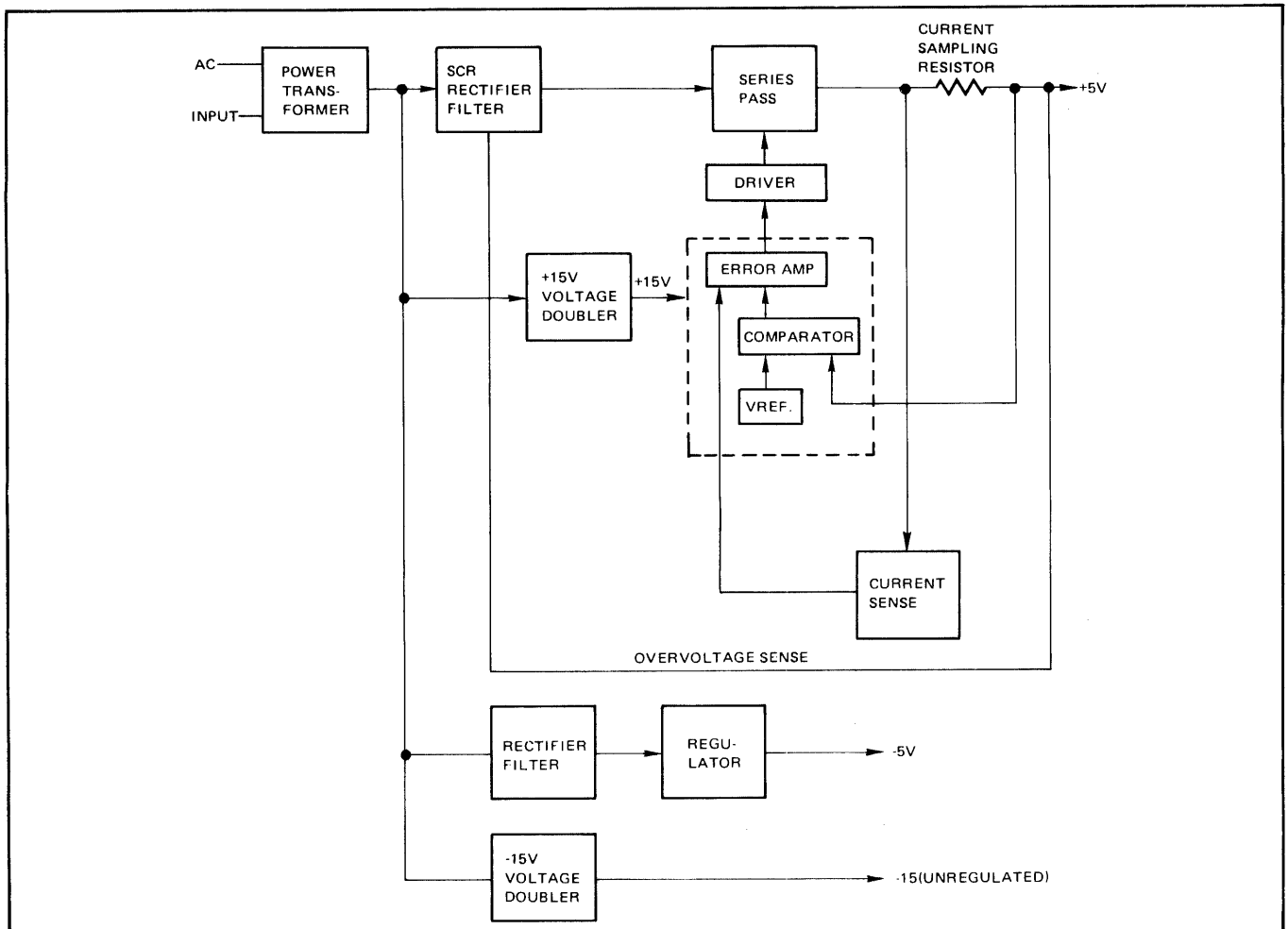
Figure A-4. Power Supply Functional Block Diagram
