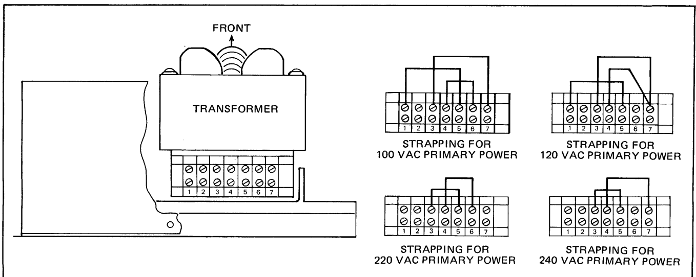
Figure 2-1. Transformer Strapping Configurations
