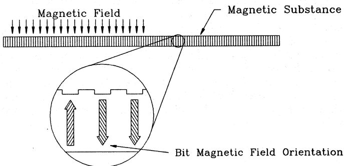
Figure 2: Magneto-Optical Recording
