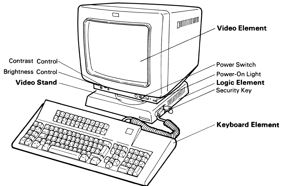
Figure 1-1. Locations of Switches and Controls
