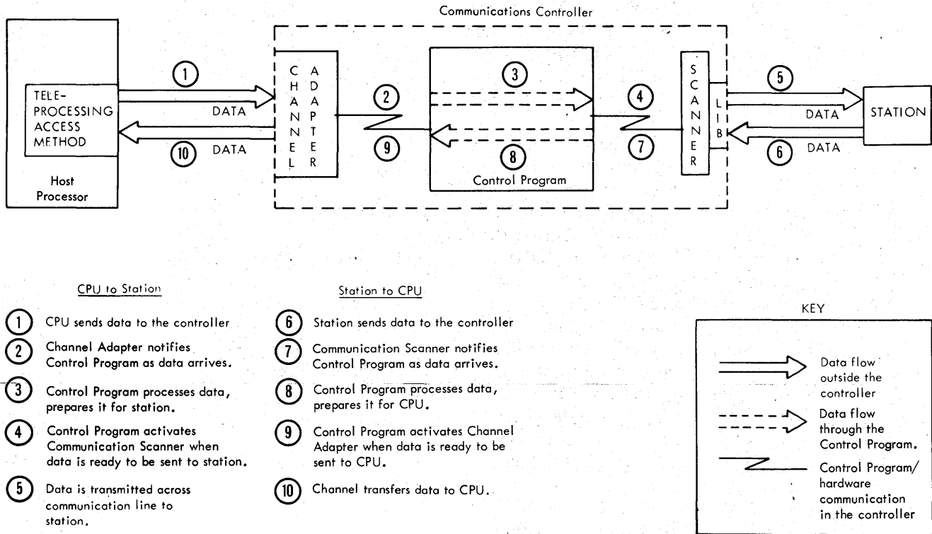
Figure 1-4. System Data Flow
