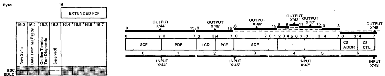
Figure 8-5. Interface Control Word Type 3 Scanner
