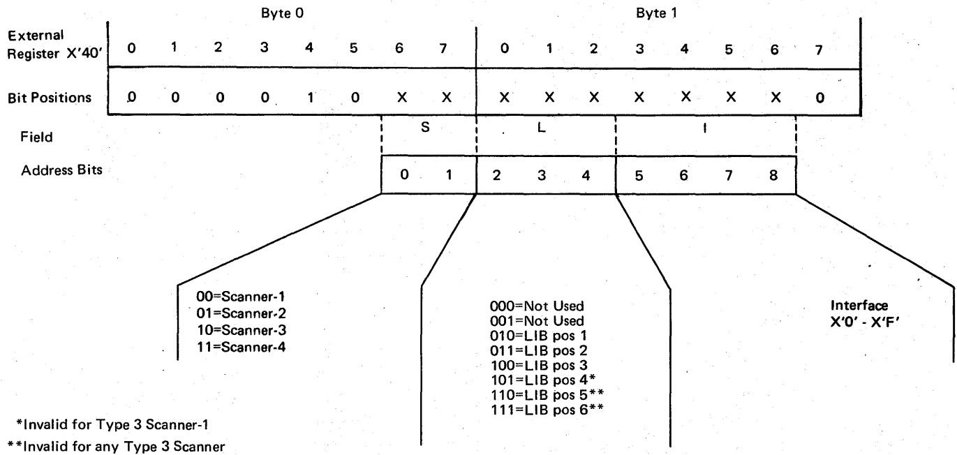
Figure 3-4. Types 2 and 3 Scanner Interface Address Bits
