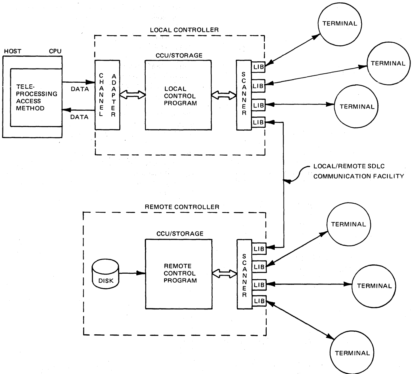
Figure 11-1. Teleprocessing System with Local and Remote Communications Controllers.
