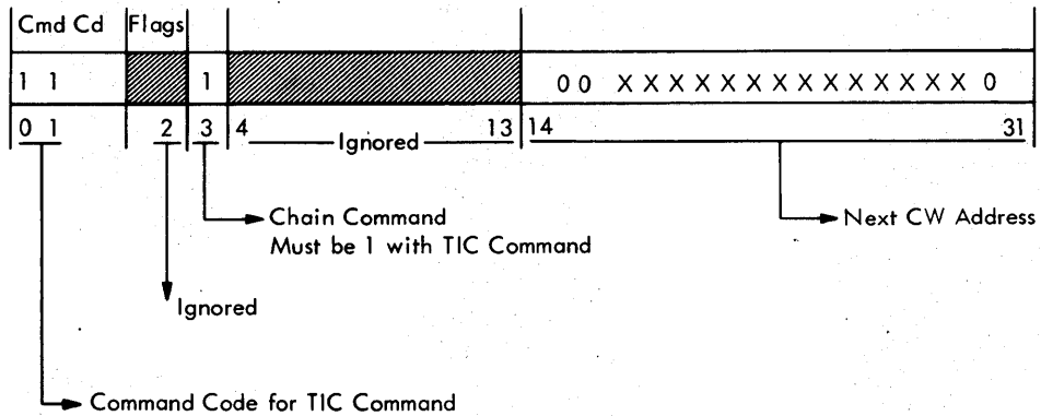
Figure 10-1. Type 2 and Type 3 Channel Adapter Control Word
