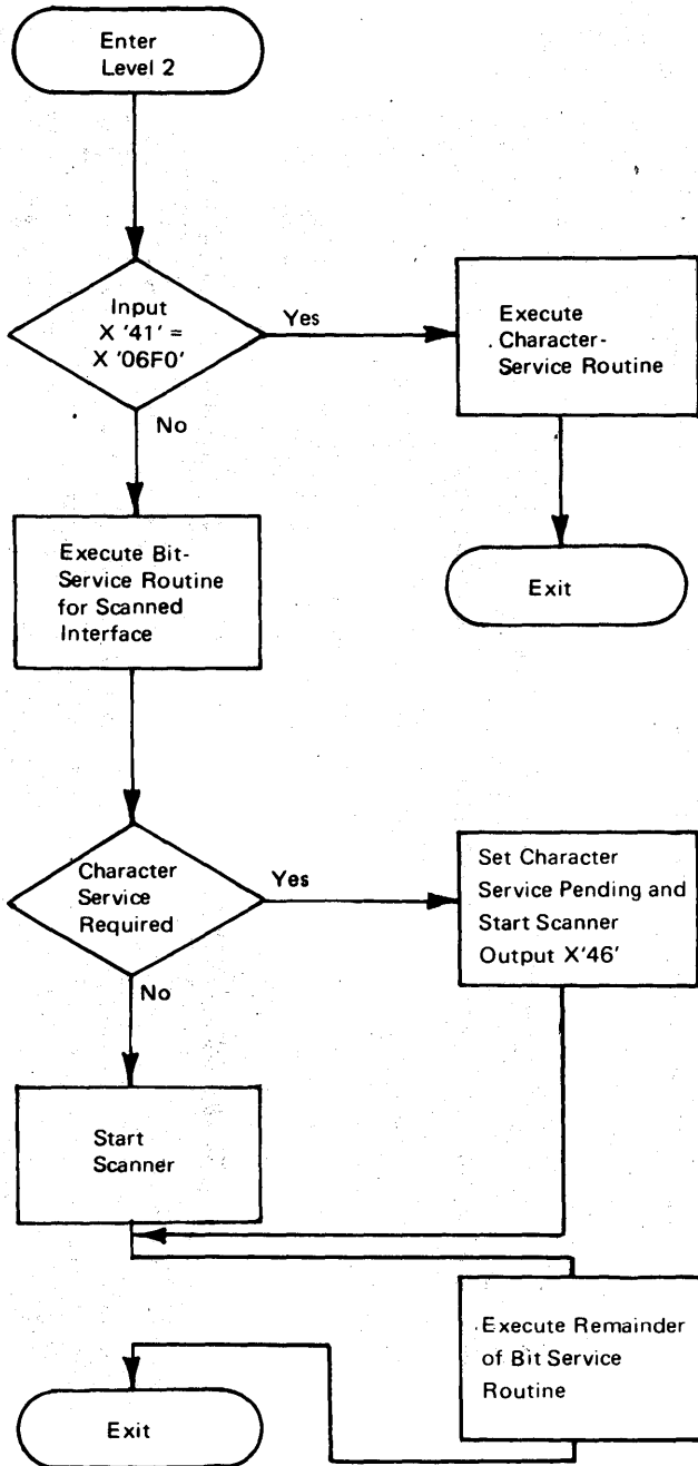
Figure 6-2. Level 2 Program Flow (Type 1 Communication Scanner)
