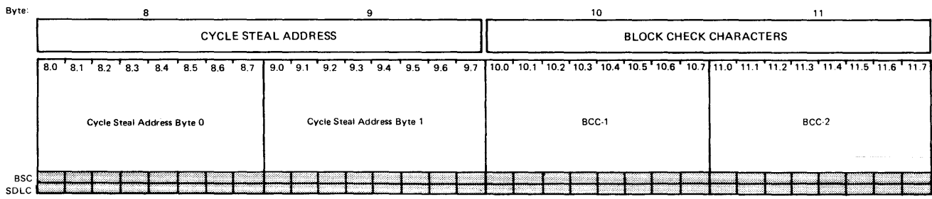
Figure 8-5. Interface Control Word Type 3 and Type 3HS Scanner (Part 1 of 2)
