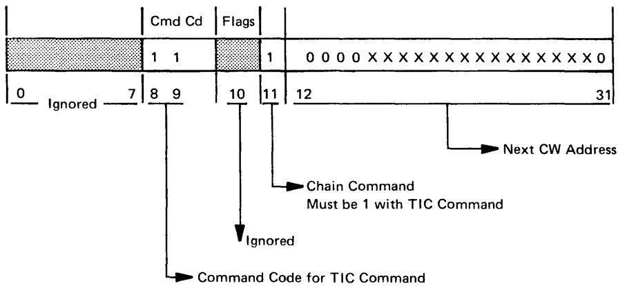
Figure 10-2. Type 2 and Type 3 Channel Adapter Control Word (3705 Models J–L only)
