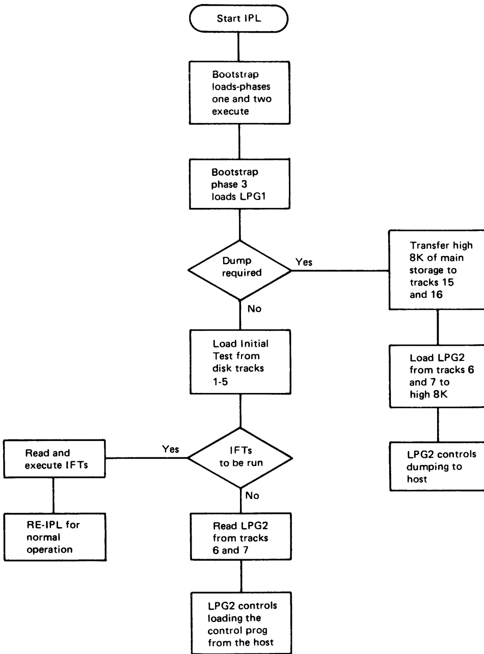
Figure 11-2. IPL—Remote Communications Controller
