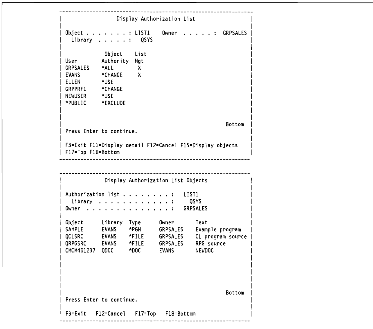
Figure 85. DSPAUTL AUTL(LIST1) and DSPAUTLOBJ AUTL(LIST1). Users and Objects on Authorization List
