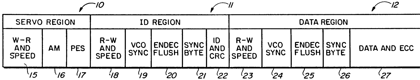
FIG. 1 (PRIOR ART)
