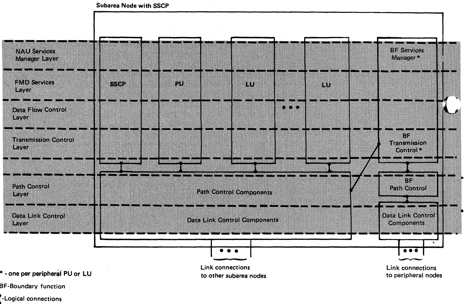
Figure 3-1. Network Addressable Units in a Subarea Node with an SSCP
