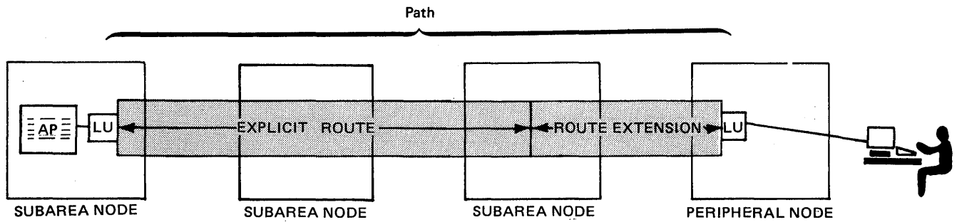
Figure 2-17. Explicit Route and Route Extension in Path
