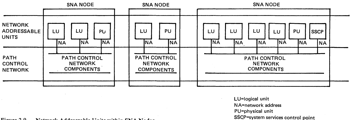
Figure 2-9. Network Addressable Units within SNA Nodes
