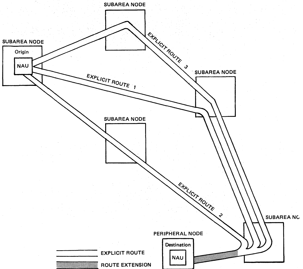
Figure 2-18. Multiple Active Routes between Subarea Nodes
