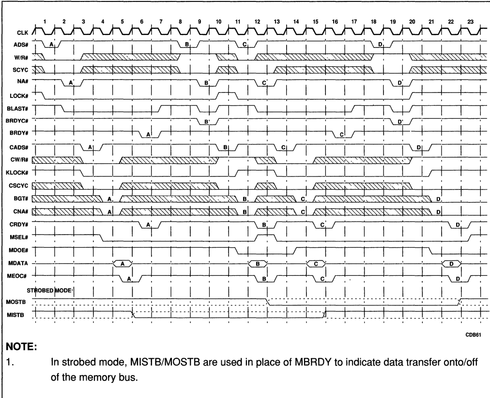
Figure 6-8. Locked Read Modify Write Cycles
