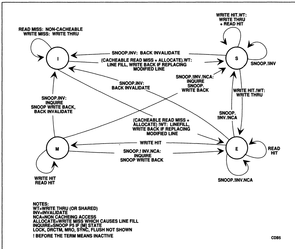
Figure 3-1. State Changes
