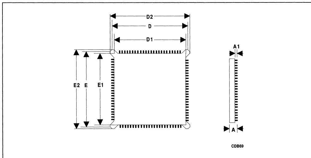
Figure 9-3. 82491 Cache SRAM Mechanical Specifications
