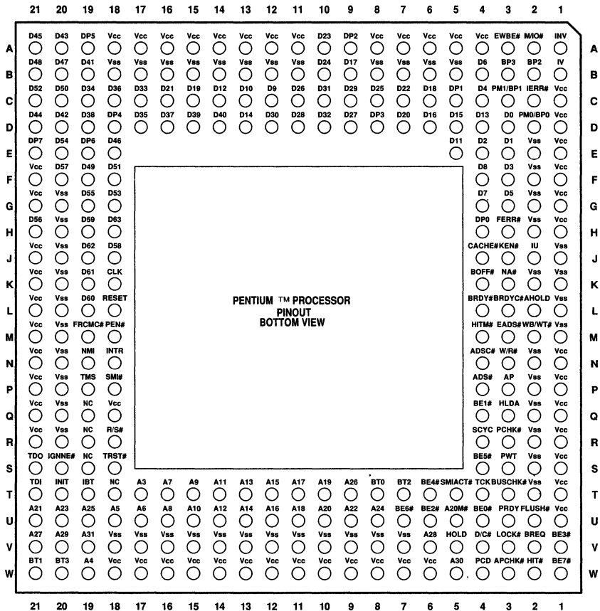
Figure 1-2. Pentium™ Processor Pinout (Bottom View)
