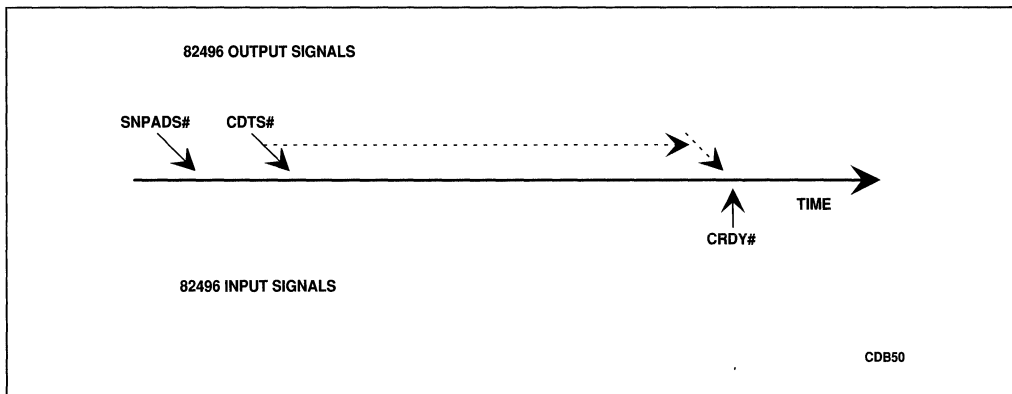
Figure 5-16. Cycle Progress for Snoop Write Back Cycles
