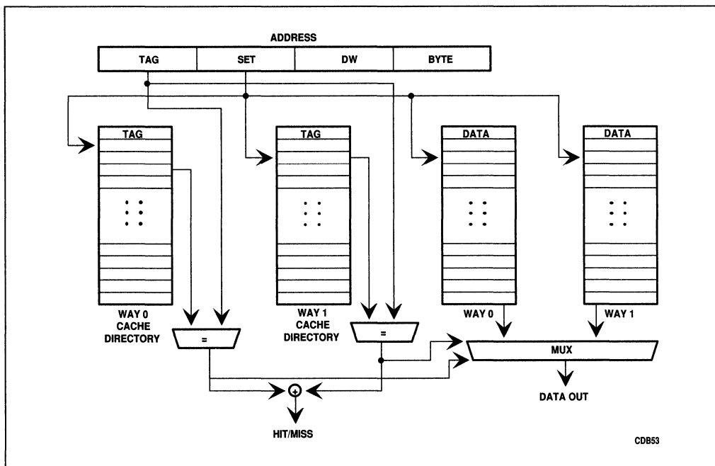
Figure 4-4. Two-Way Set Associative TagRAM Structure
