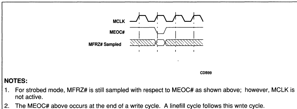
Figure 5-28. MFRZ# Sampling
