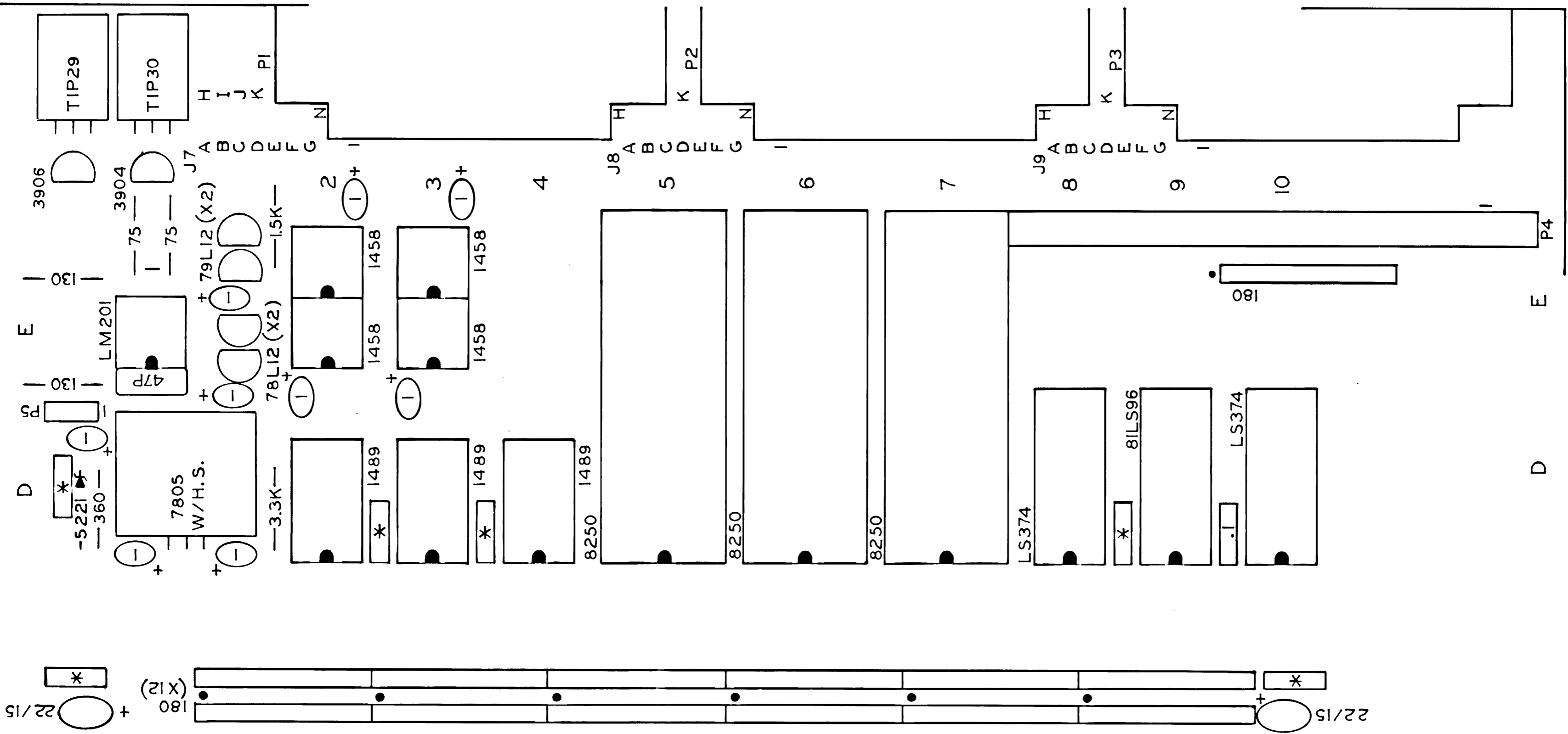
WUNDER BUS I/O COMPONENT SILKSCREEN REV. 1
