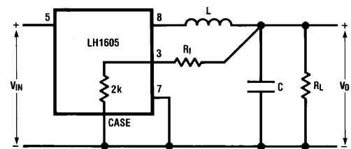
FIGURE 11. Output Voltage Feedback with LH1605
