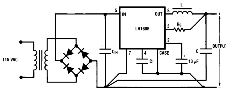
FIGURE 18. Typical Power Supply System
