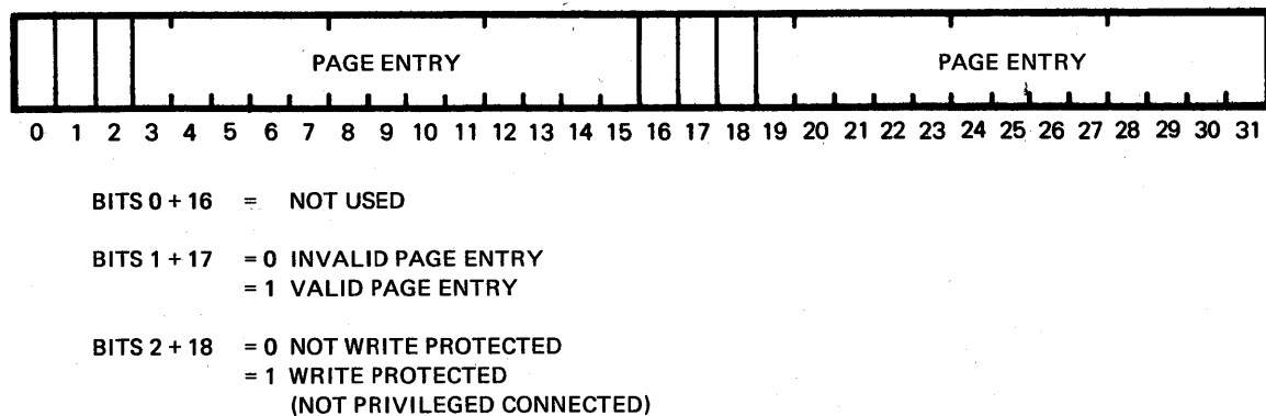
Figure 4-7. MAP Image Descriptor (MID)
