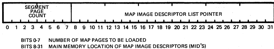
Figure 4-6. MAP Segment Descriptor (MSD)
