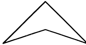
concave polygon
