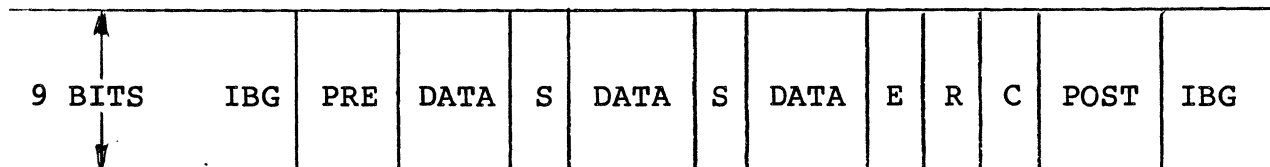
Figure 8-2 GCR Data Block Format
