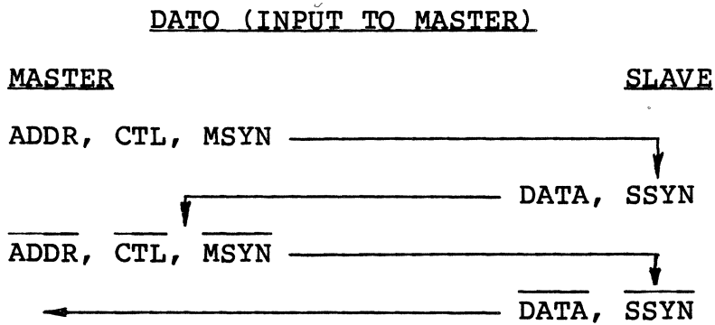
Figure 4-3 Bus Transfer Sequences
