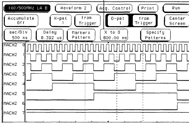
X to O Display Field
