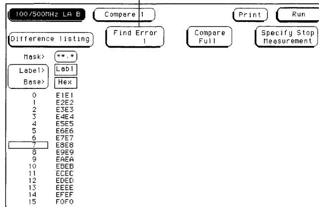
Find Error Field
