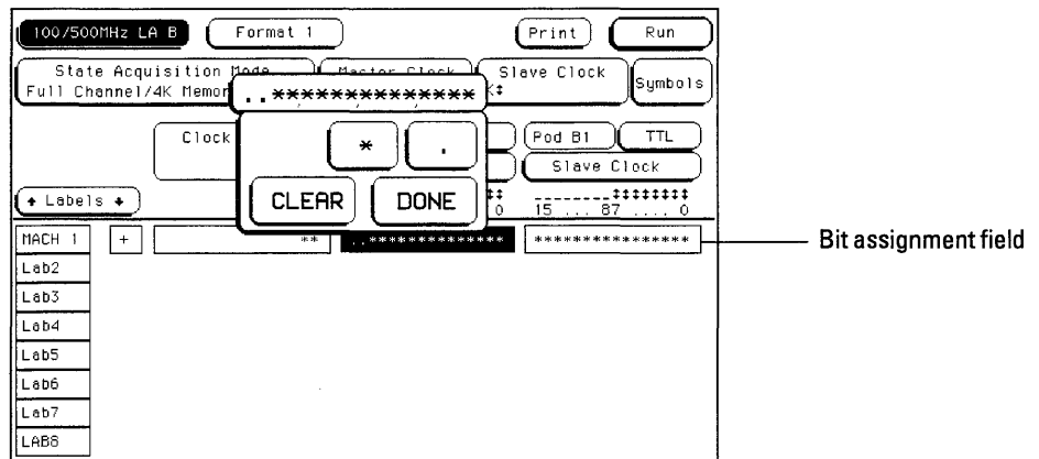
Bit Assignment Field
