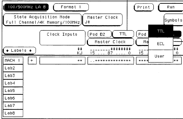
Pod threshold field
