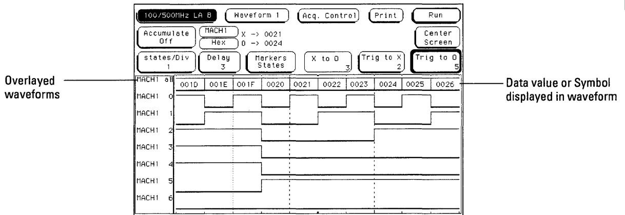
State Data or Symbols In Overlaid Waveform
