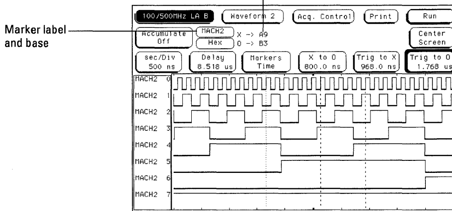
Marker Label / Base and Display
