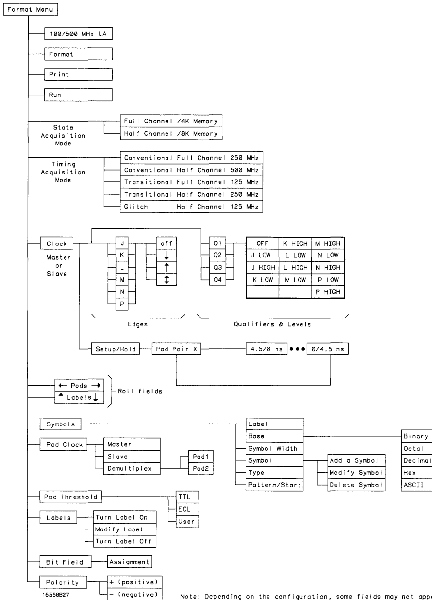
The State Format Menu Map
