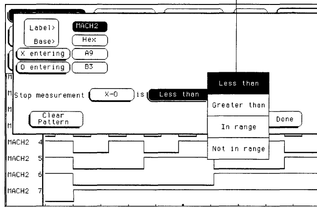
X to O option menu
