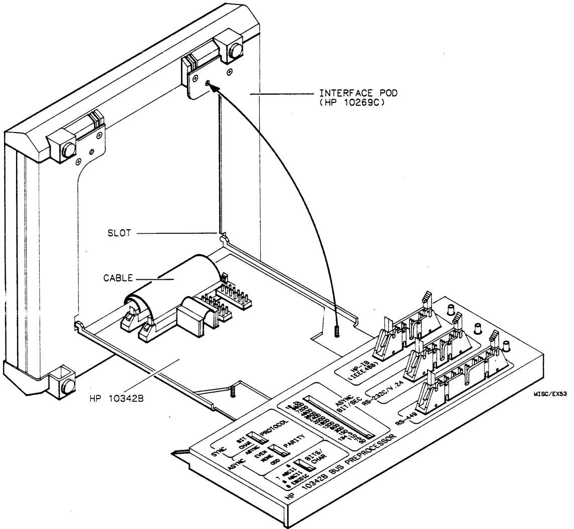
Figure 6-3. Installing the HP 10342B in the HP 10269C
