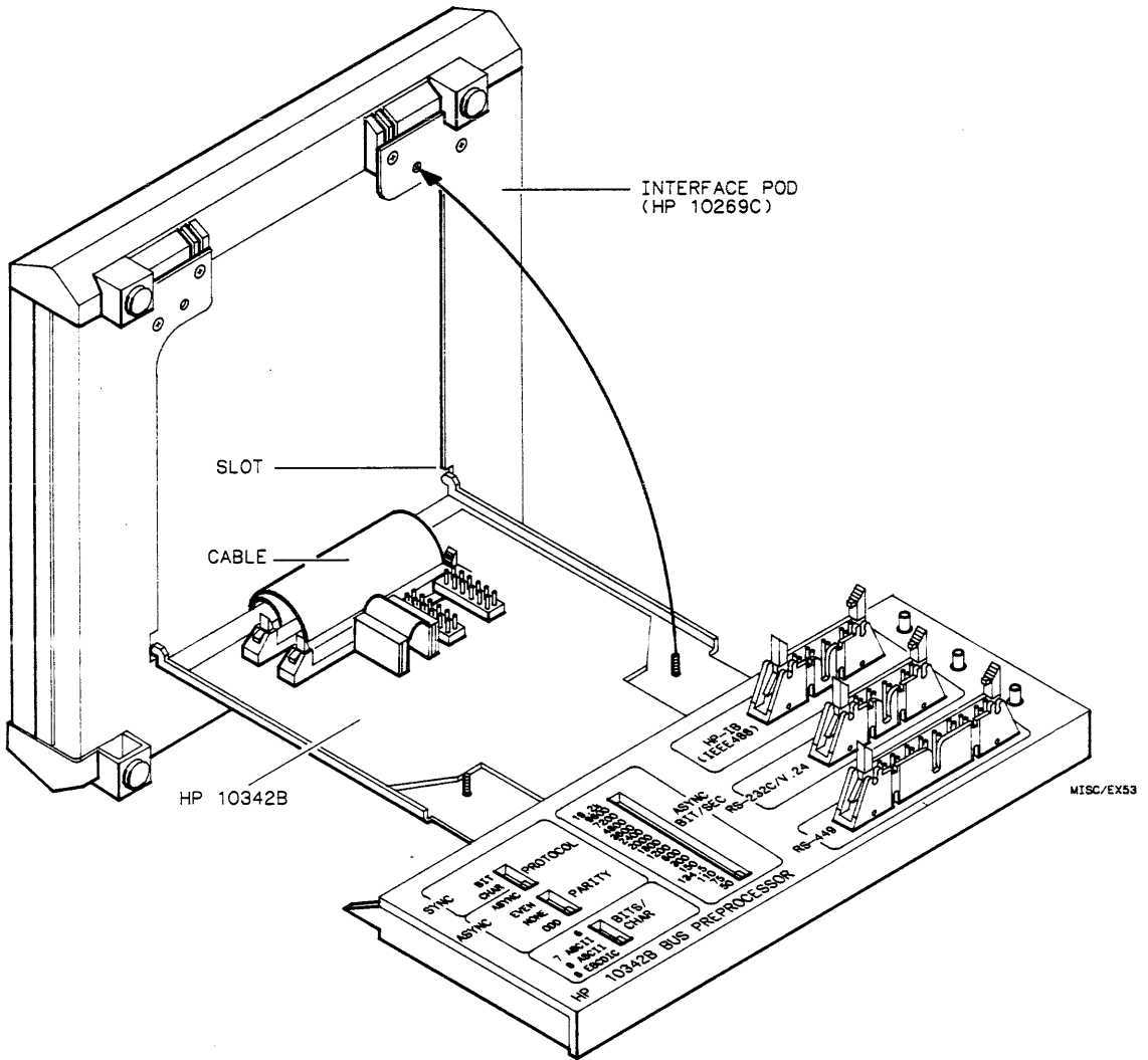
Figure 5-3. Installing the HP 10342B in the HP 10269C
