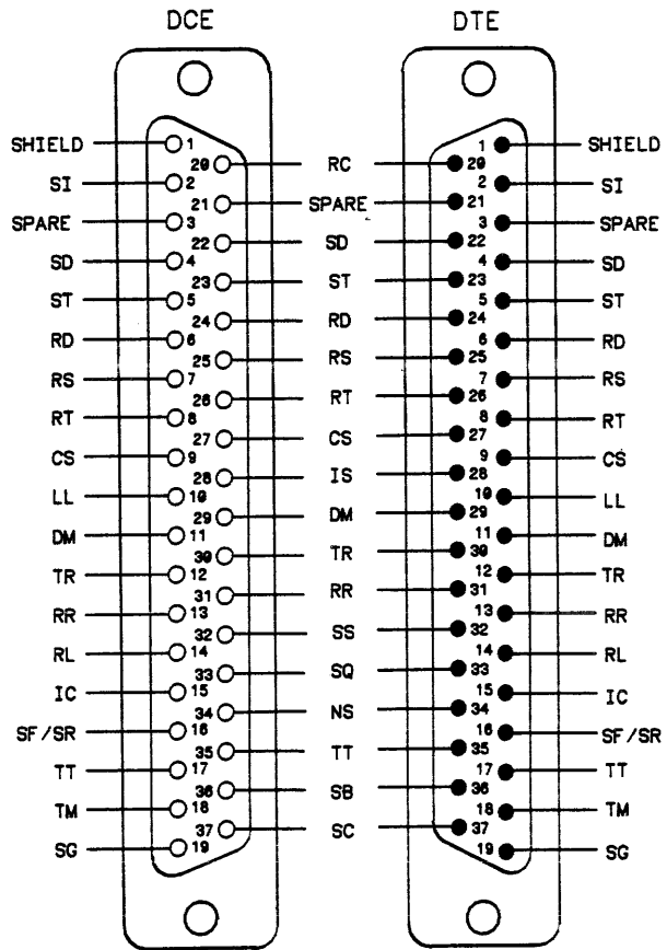
Figure D-1. RS-449 Connector with Pin Assignments
